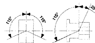
Mounting position
