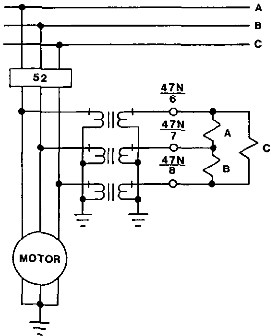
FIGURE 3. WYE VOLTAGE SENSING
