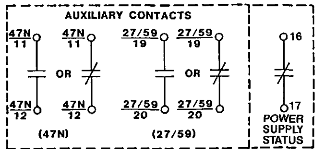
FIGURE 5. CONTROL CIRCUITS
