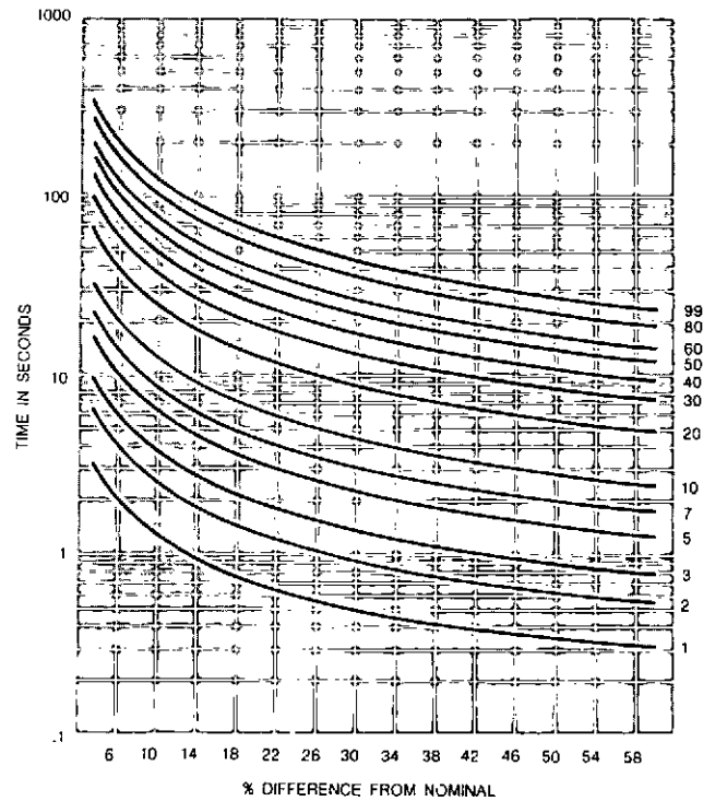
FIGURE 2. INVERSE TIME CHARACTERISTIC CURVES
