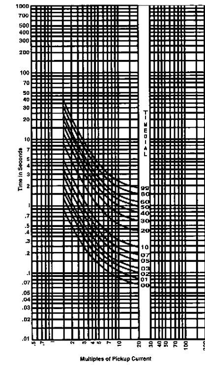
FIGURE 12. B6 - VERY INVERSE
