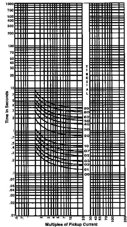
FIGURE 9. B3 - DEFINITE TIME
