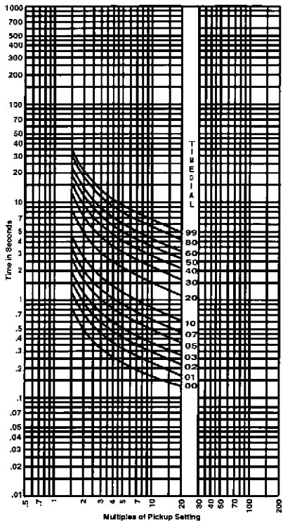
FIGURE 16. E5 - INVERSE (2.9) BRITISH STANDARD 142 CURVE
