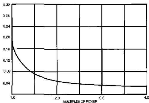
Figure 6. Typical Instantaneous Function Response Time
