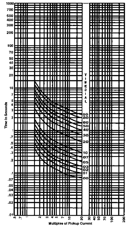
FIGURE 15. E4 - INVERSE (1.3) BRITISH STANDARD 142 CURVE
