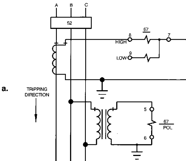
Figure 1 - Directional Overcurrent (Single-Phase)
