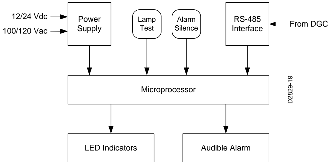
Figure 4. RDP-110 Function Blocks
