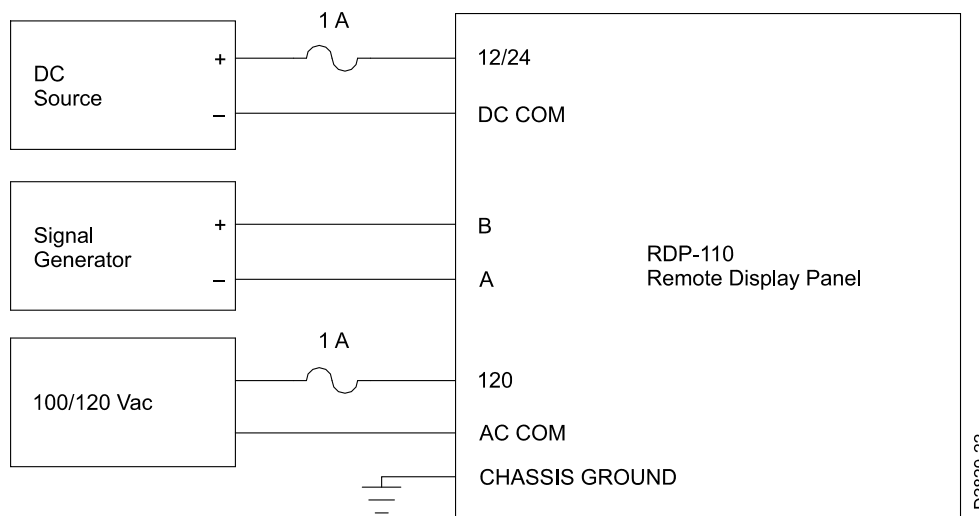
Figure 9. RDP-110 Test Setup
