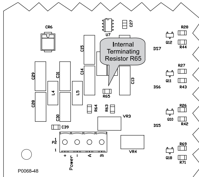
Figure 7. RS-485 Terminating Resistor Location
