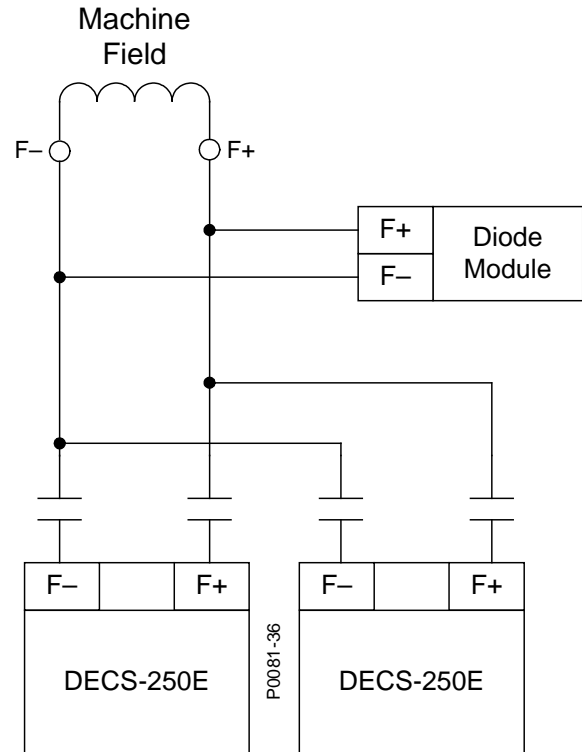
Figure 2. Typical Connections
