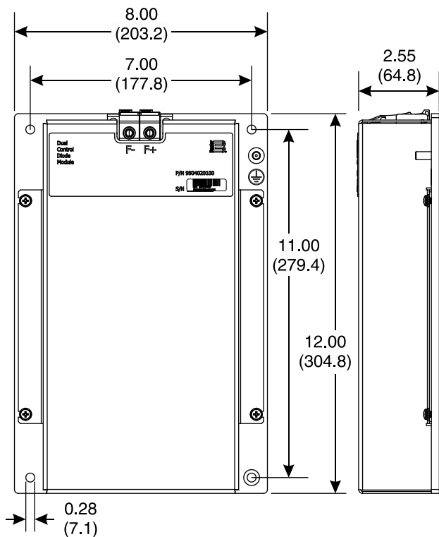
Figure 1. Overall Dimensions
