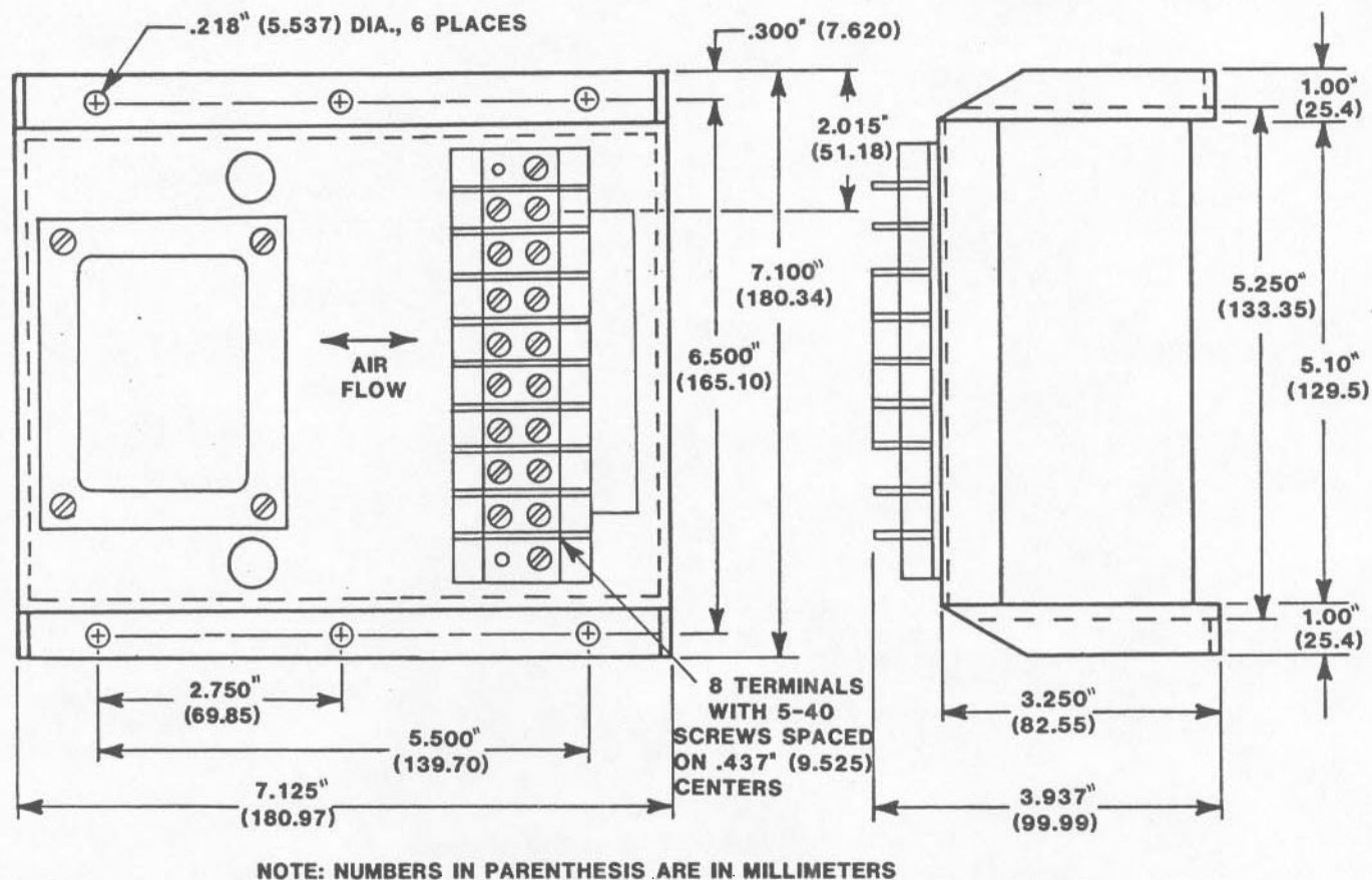
Figure 4-3. Outline Drawing.
