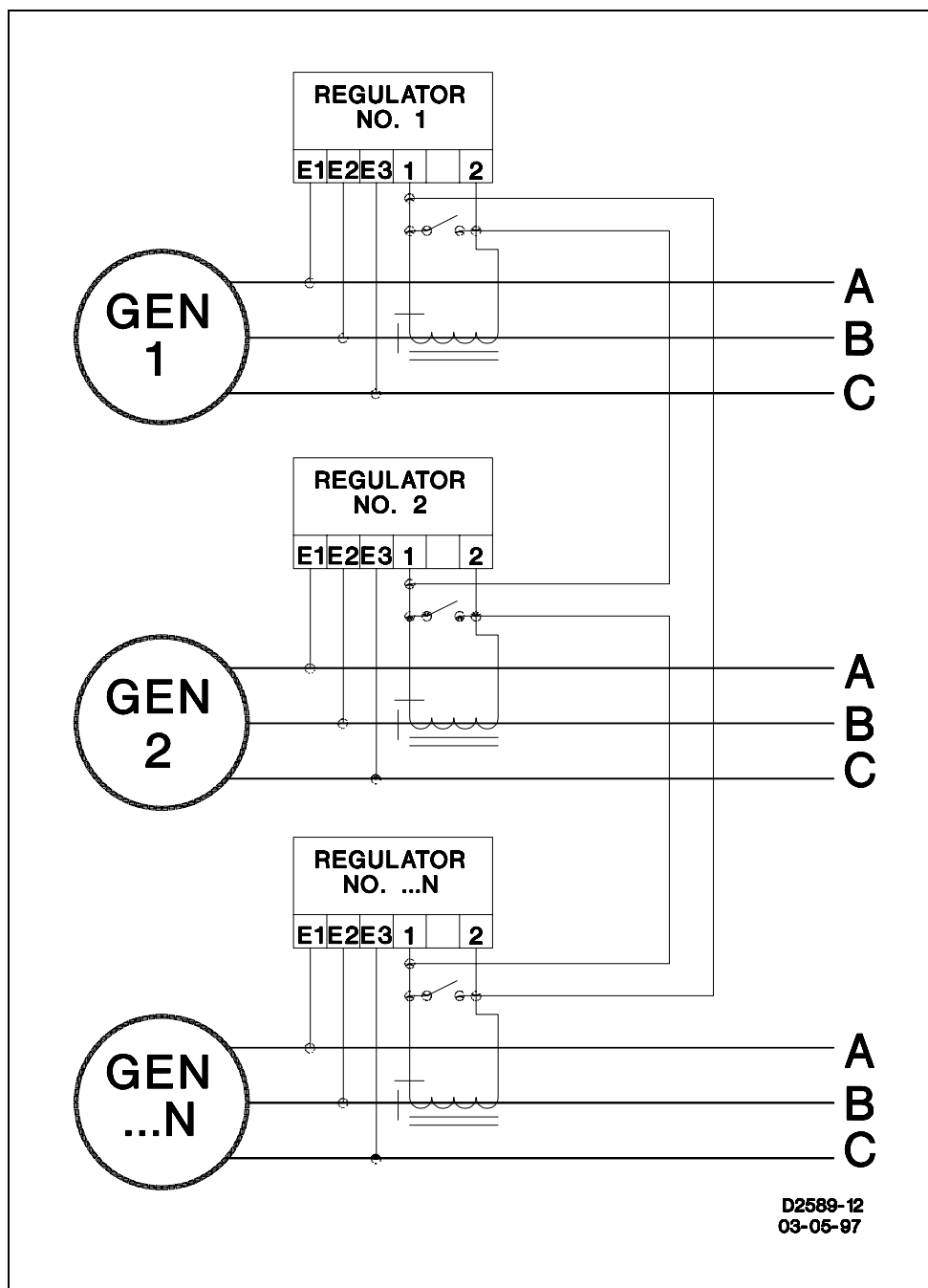
Figure 3-6. Reactive Differential (Cross-current) Compensation CT Interconnection.
