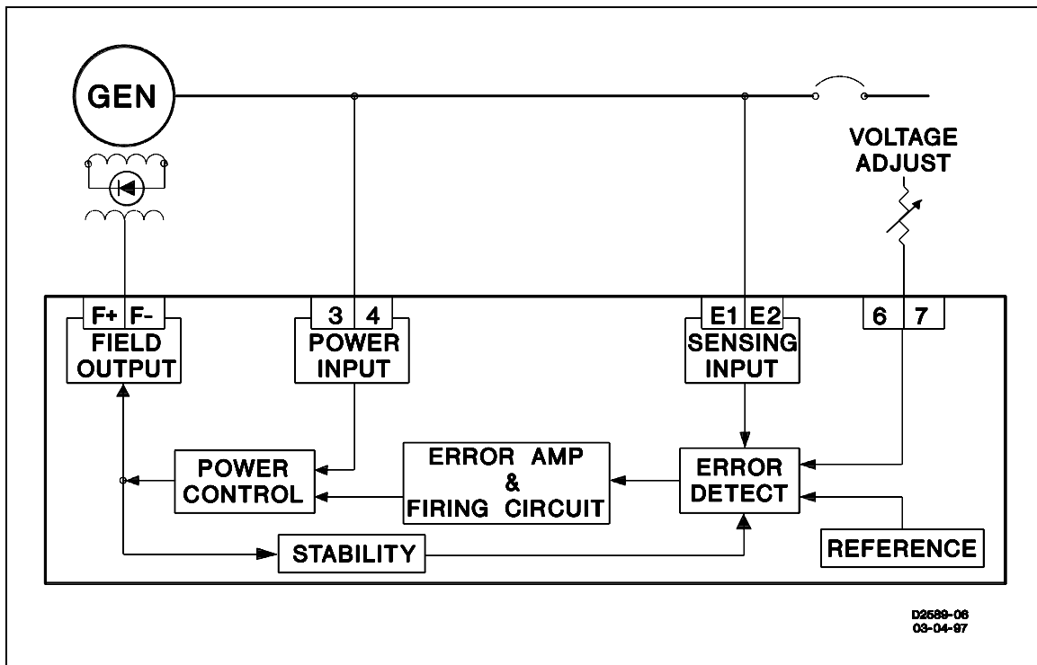
Figure 2-1. Overall Block Diagram.
