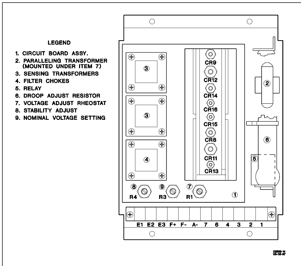
Figure 5-2. Component Location and Identification.
