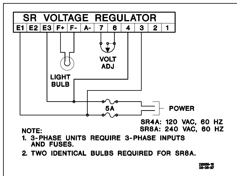
Figure 5-1. Operational Test.
