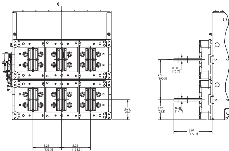
Horizontal Main Bus Connectors
