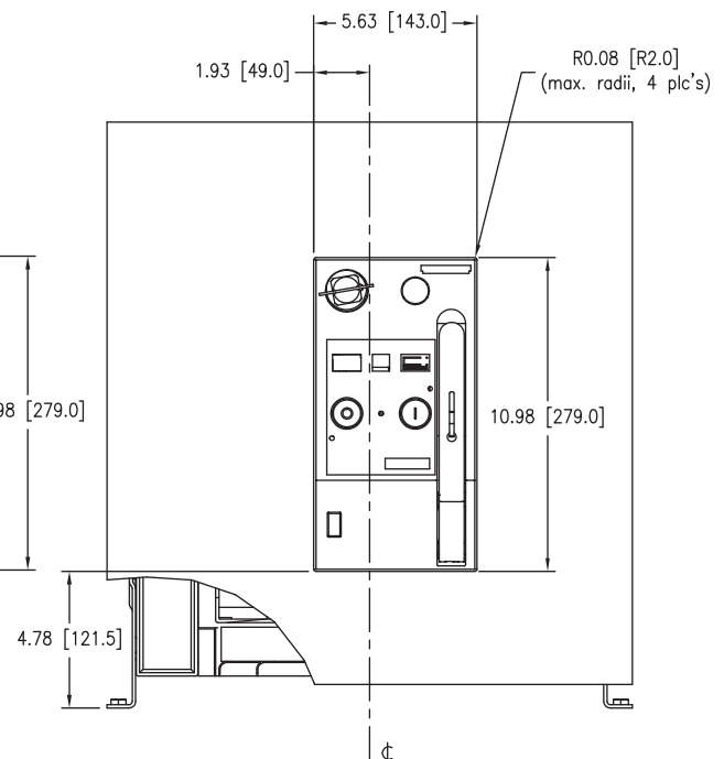
Minimal door cut-out (Only center eustcheon visible)
