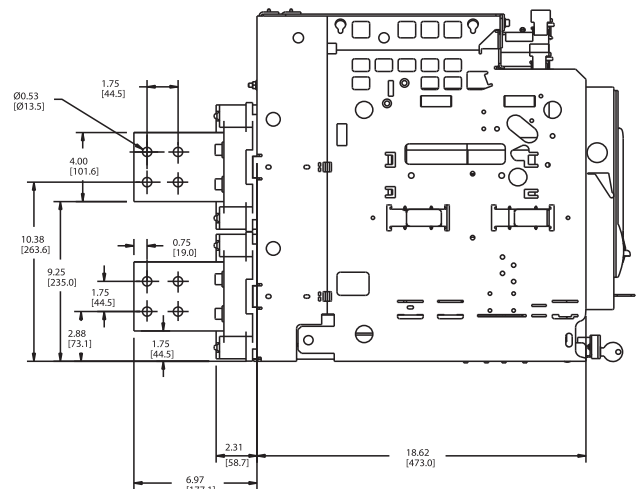
Vertical Main Bus Connectors
