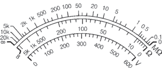
Figure 3—Typical scale on the Megger insulation tester.
