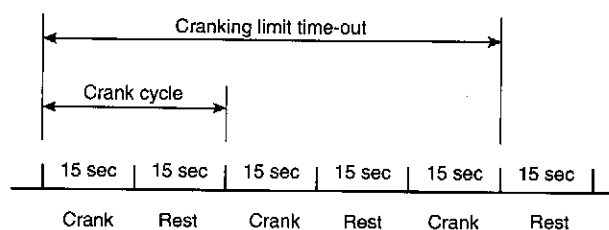
FIGURE A.5.6.4.2 Diagram of Cranking Cycles.
