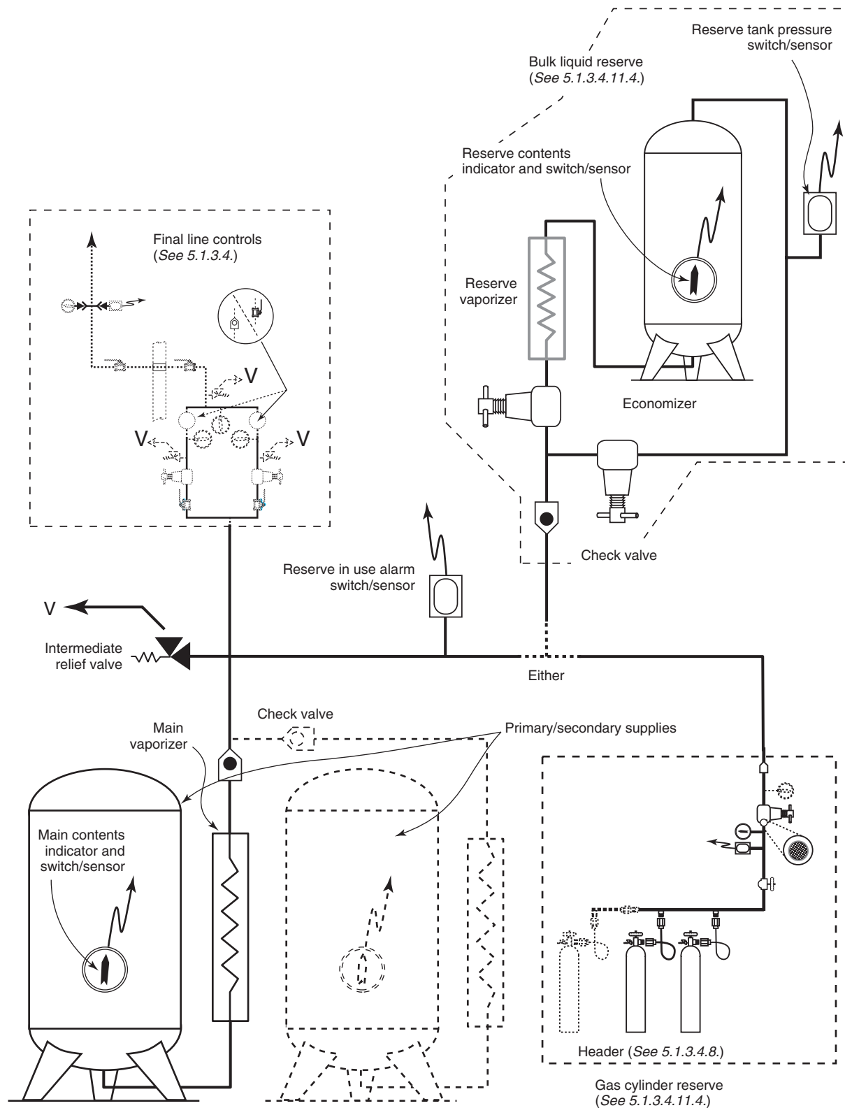
FIGURE A.5.1.3.4.11 Typical Source of Supply for Cryogenic Gas in Bulk.
