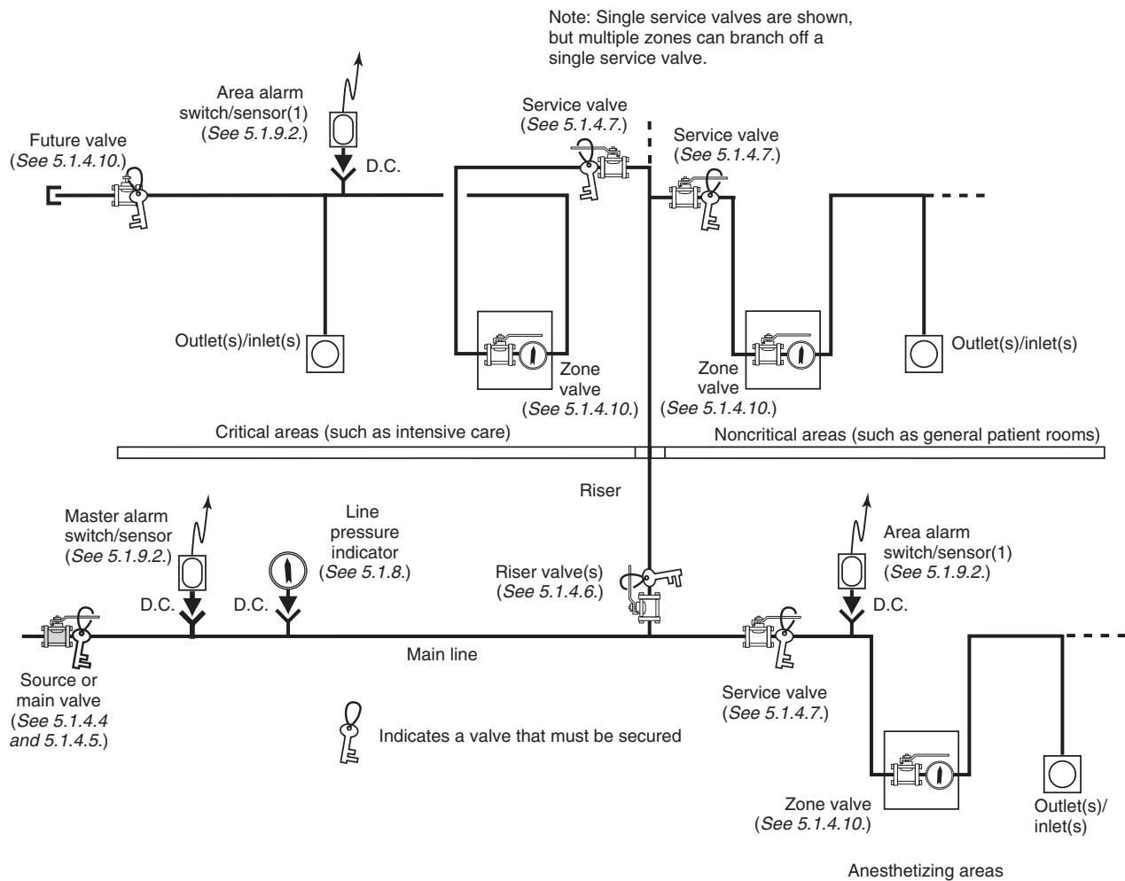
FIGURE A.5.1.4 Arrangement of Pipeline Components.
