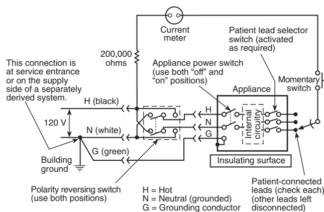
FIGURE 10.2.13.5.3.2 Test Circuit for Measuring the Electrical Isolation of Isolated Patient Leads.
