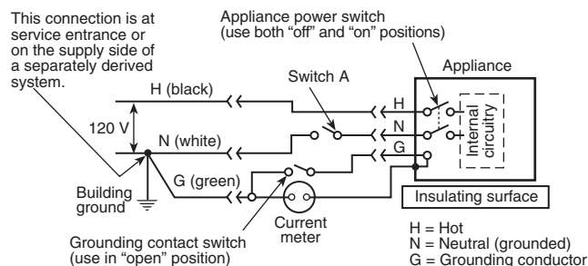
FIGURE 8.4.1.3.5.5 Test Circuit for Measuring Chassis Leakage Current.
