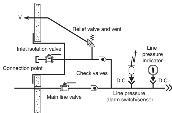
FIGURE A.5.1.3.4.12 Emergency Oxygen Supply Connection.
