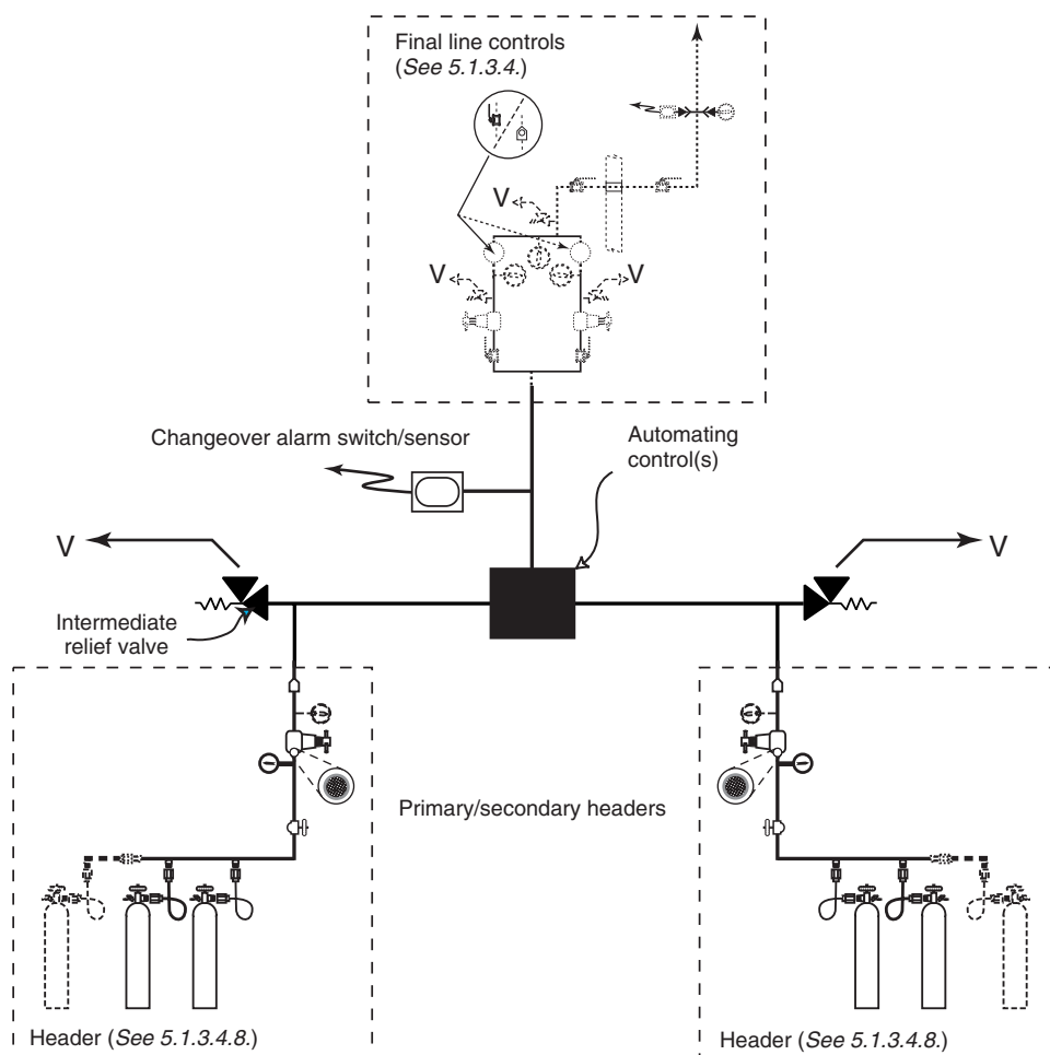
FIGURE A.5.1.3.4.9 Manifold for Gas Cylinders.
