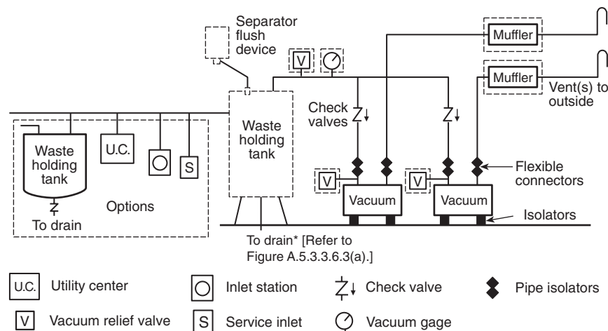
FIGURE A.5.3.3.6(c) Typical Level 3 Wet or Dry Piping System with Single Vacuum Source.
