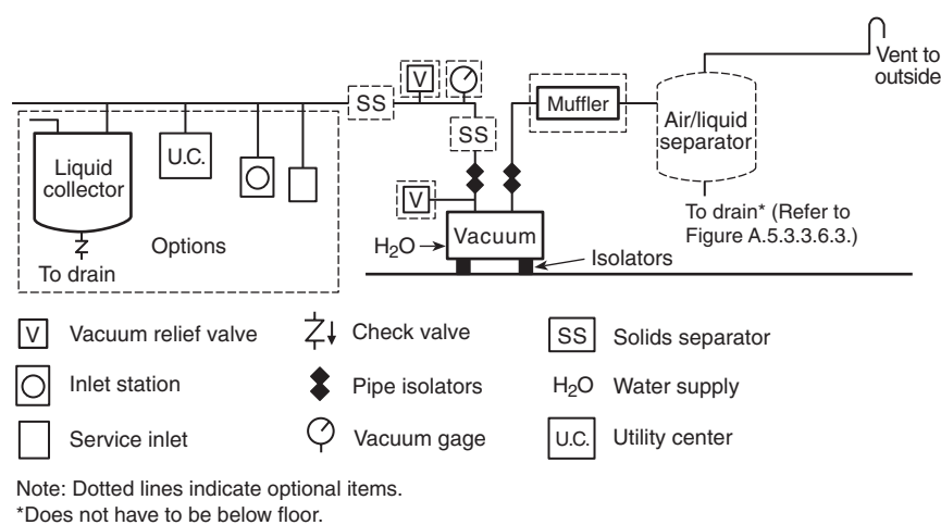
FIGURE A.5.3.3.6(a) Typical Level 3 Wet or Dry Piping Systems with Single Vacuum Pump Source.
