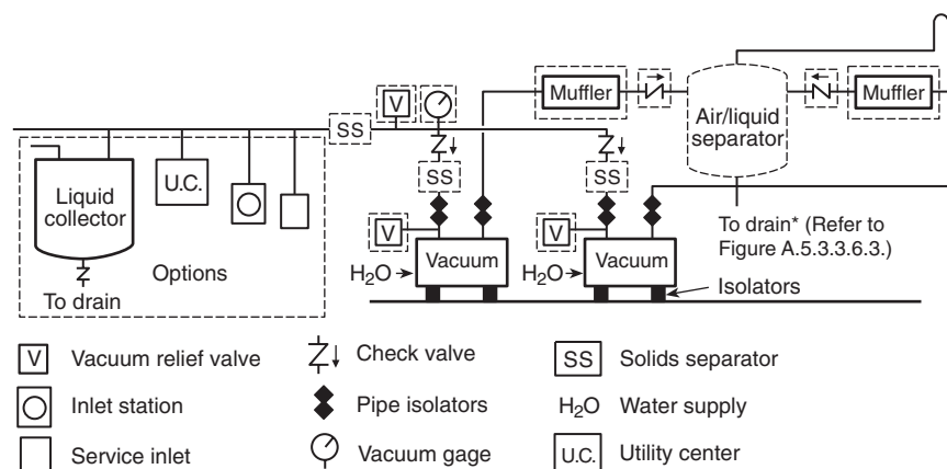
FIGURE A.5.3.3.6(b) Typical Level 3 Wet or Dry Piping System with Duplex Vacuum Source.
