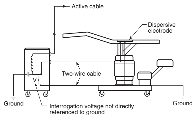
FIGURE D.3.3.1.4(b) Electrocautery Unit with a dc Isolated Patient Plate.
