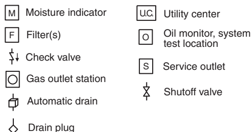
FIGURE A.5.3.3.5 Level 3 Gas-Powered Devices Supply System.
