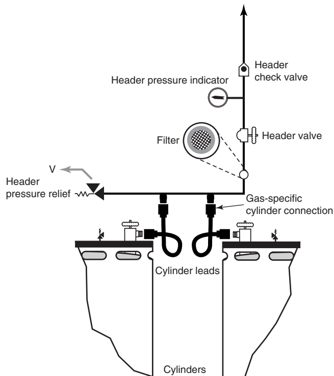
FIGURE A.5.1.3.4.8(b) Header for Cryogenic Gas in Containers.
