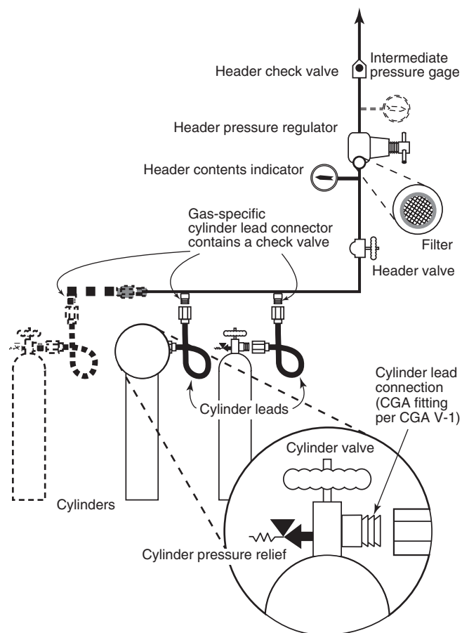
FIGURE A.5.1.3.4.8(a) Header for Gas in Cylinders.
