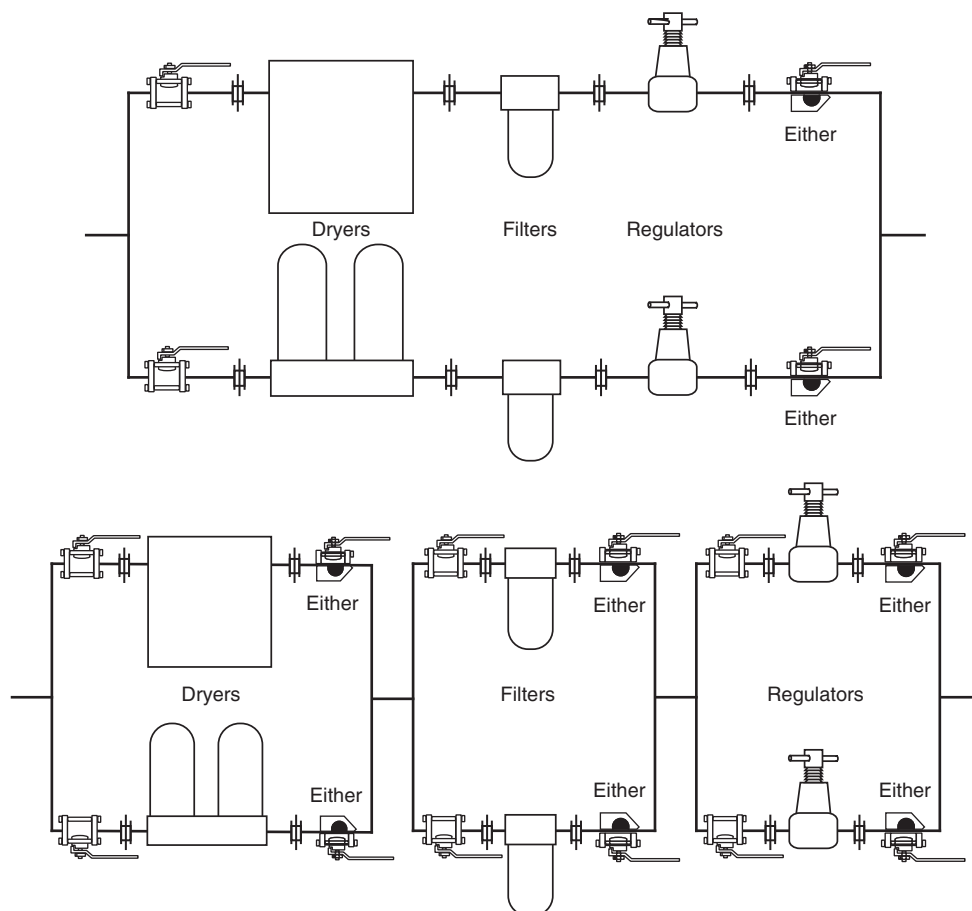
FIGURE A.5.1.3.5.11.6 Alternate Valving Sequences for Line Controls in Medical Air.
