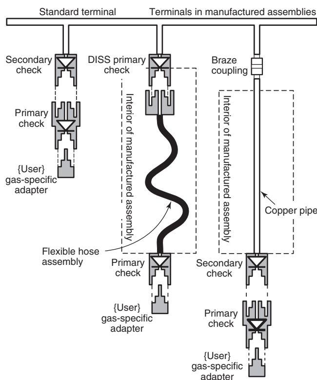
FIGURE A.5.1.6 Terminals in Manufactured Assemblies.
