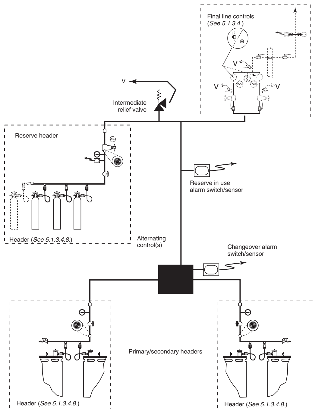
FIGURE A.5.1.3.4.10 Typical Source of Supply for Cryogenic Gas in Containers.
