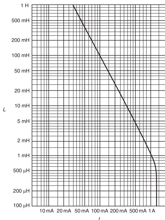
FIGURE 10.2.9.3(c) Inductance Circuits ( L > 1 \text{ mH} ). Minimum Igniting Currents at 24 V, Applicable to All Circuits Containing Cadmium, Zinc, or Magnesium.
