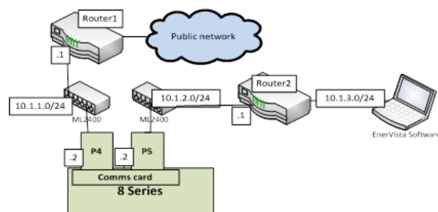
Figure 2-2: Topology Example
