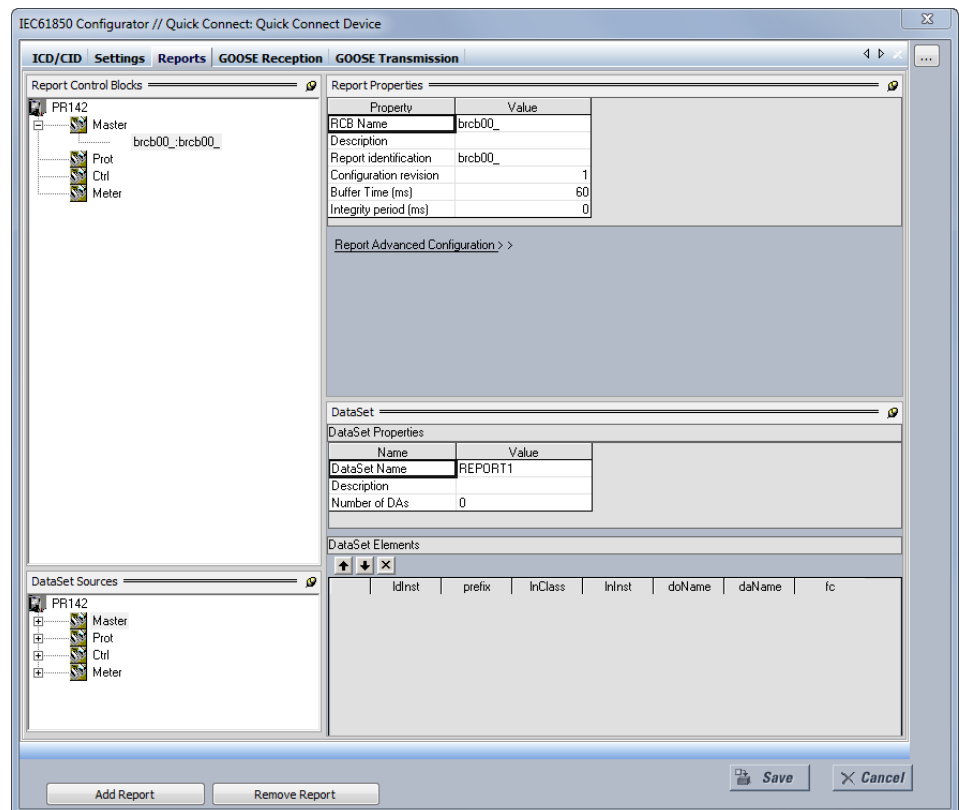
Figure 8-1: Reports Screen
