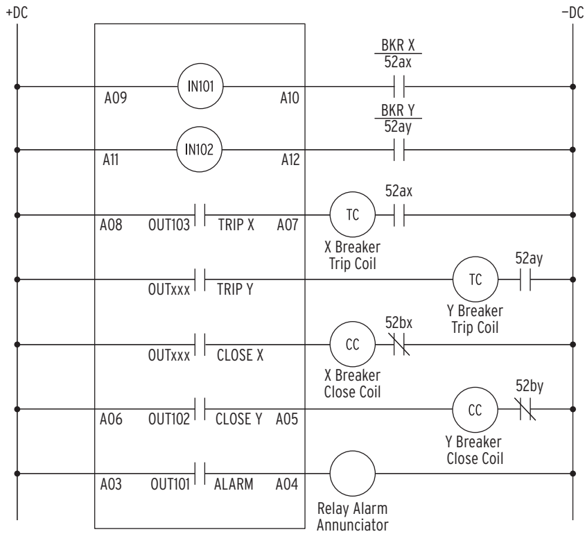
Figure 37 SEL-700GW Typical DC External Connections
