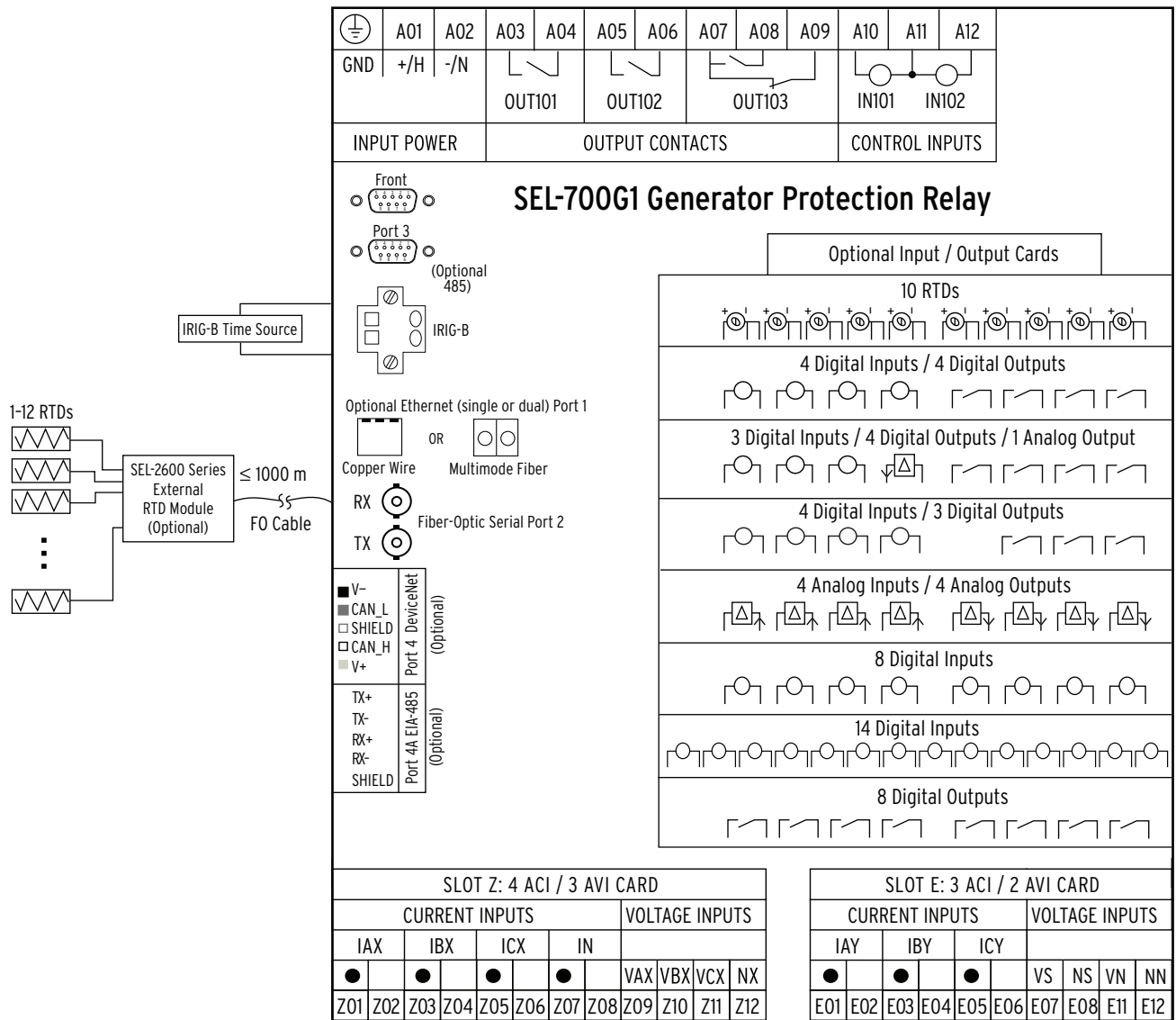
Figure 27 Typical Connection Diagram
