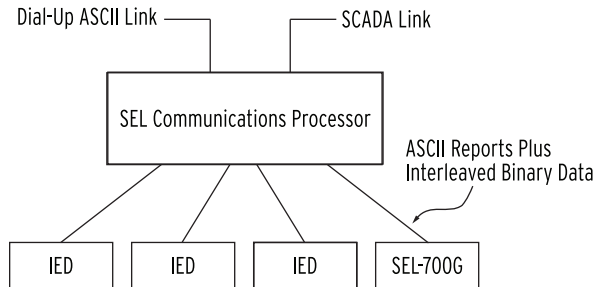
Figure 21 Example Communications System
