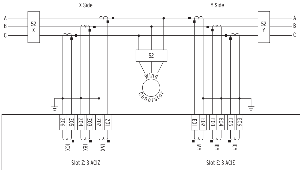
Figure 36 SEL-700GW Dual Feeder AC Current Connections
