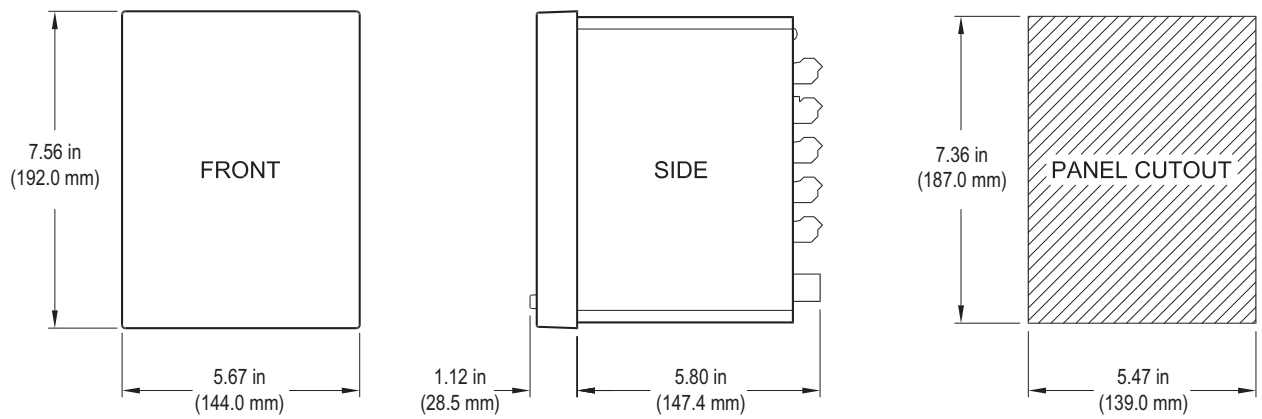
Figure 26 SEL-700G Dimensions for Rack- and Panel-Mount Models
