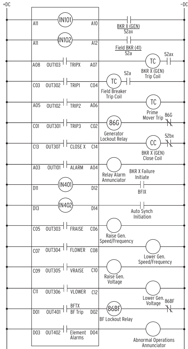
Figure 32 SEL-700G1 Typical DC External Connections
