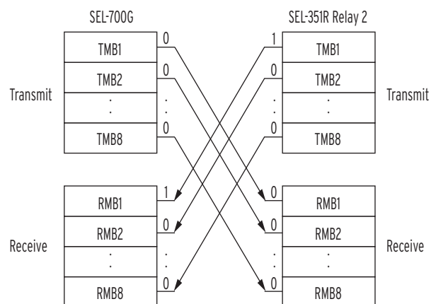
Figure 25 MIRRORED BITS Transmit and Receive Bits
