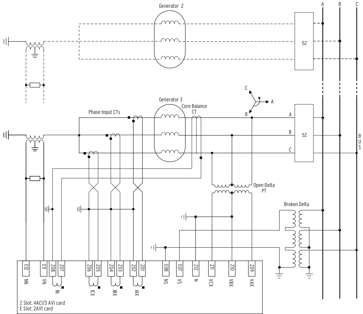
Figure 33 SEL-700G1+ Relay AC Connection Example, Multiple High-Impedance Grounded Generators Connected to a Common Bus, With 67N and Other Protection
