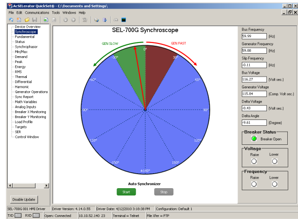
Figure 4 QuickSet Synchroscope
