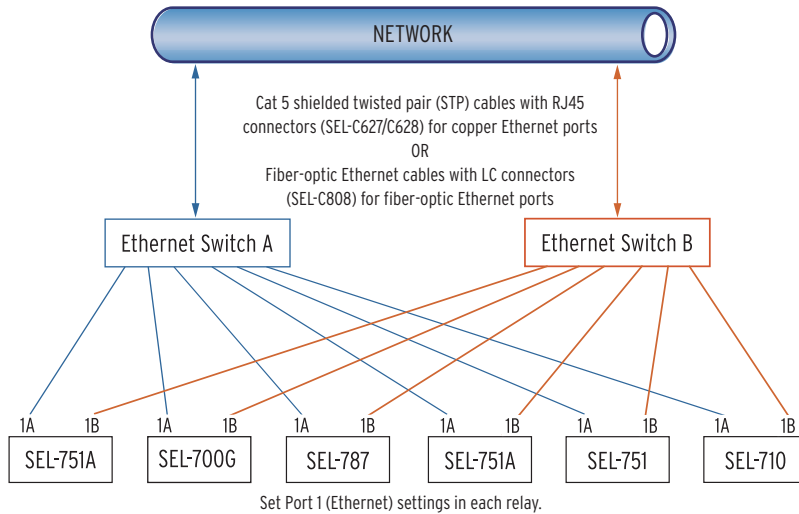
Figure 23 Ethernet Network Configuration With Dual Redundant Connections (Failover Mode)
