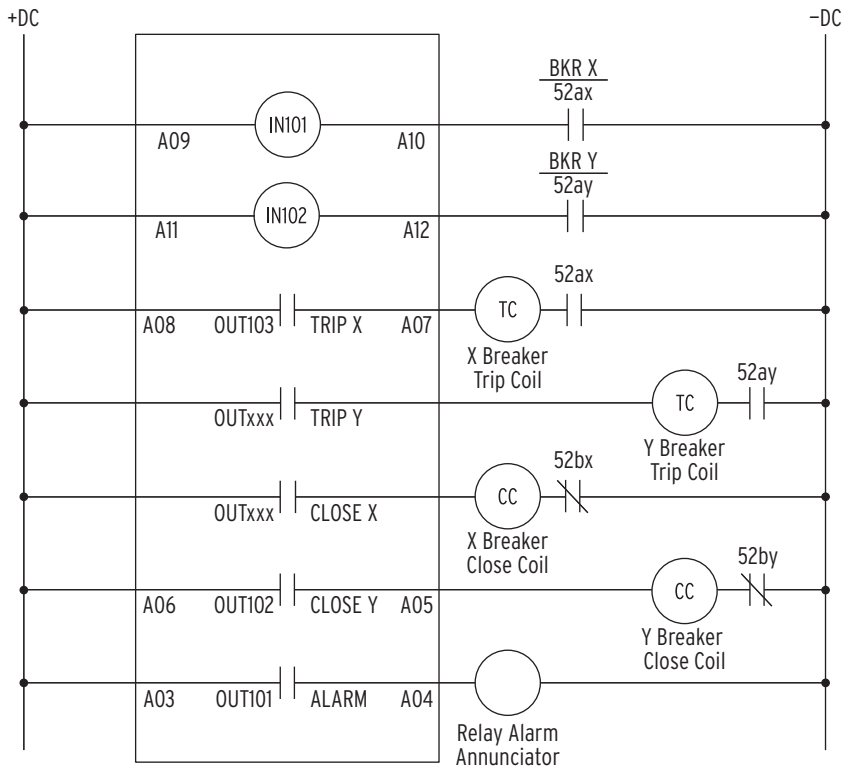
Figure 35 SEL-700GT Typical DC External Connections
