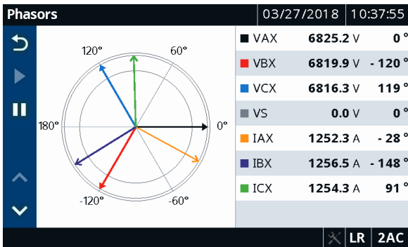
Figure 13 Meter Phasors
