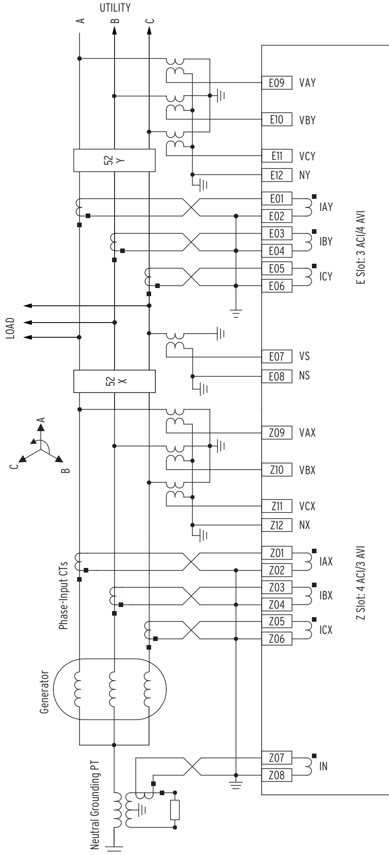
Figure 34 SEL-700GT Relay Typical AC Current and Four-Wire Wye Voltage Connection
