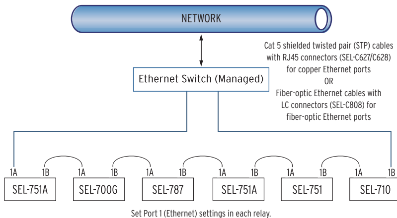
Figure 24 Ethernet Network Configuration With Ring Structure (Switched Mode)
