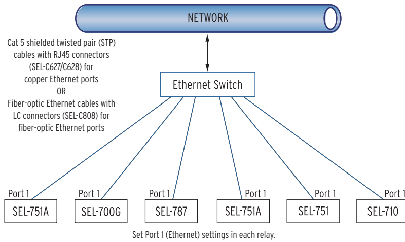
Figure 22 Simple Ethernet Network Configuration
