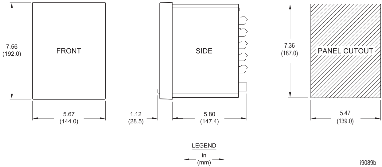
Figure 13 SEL-751A Dimensions for Rack- and Panel-Mount Models
