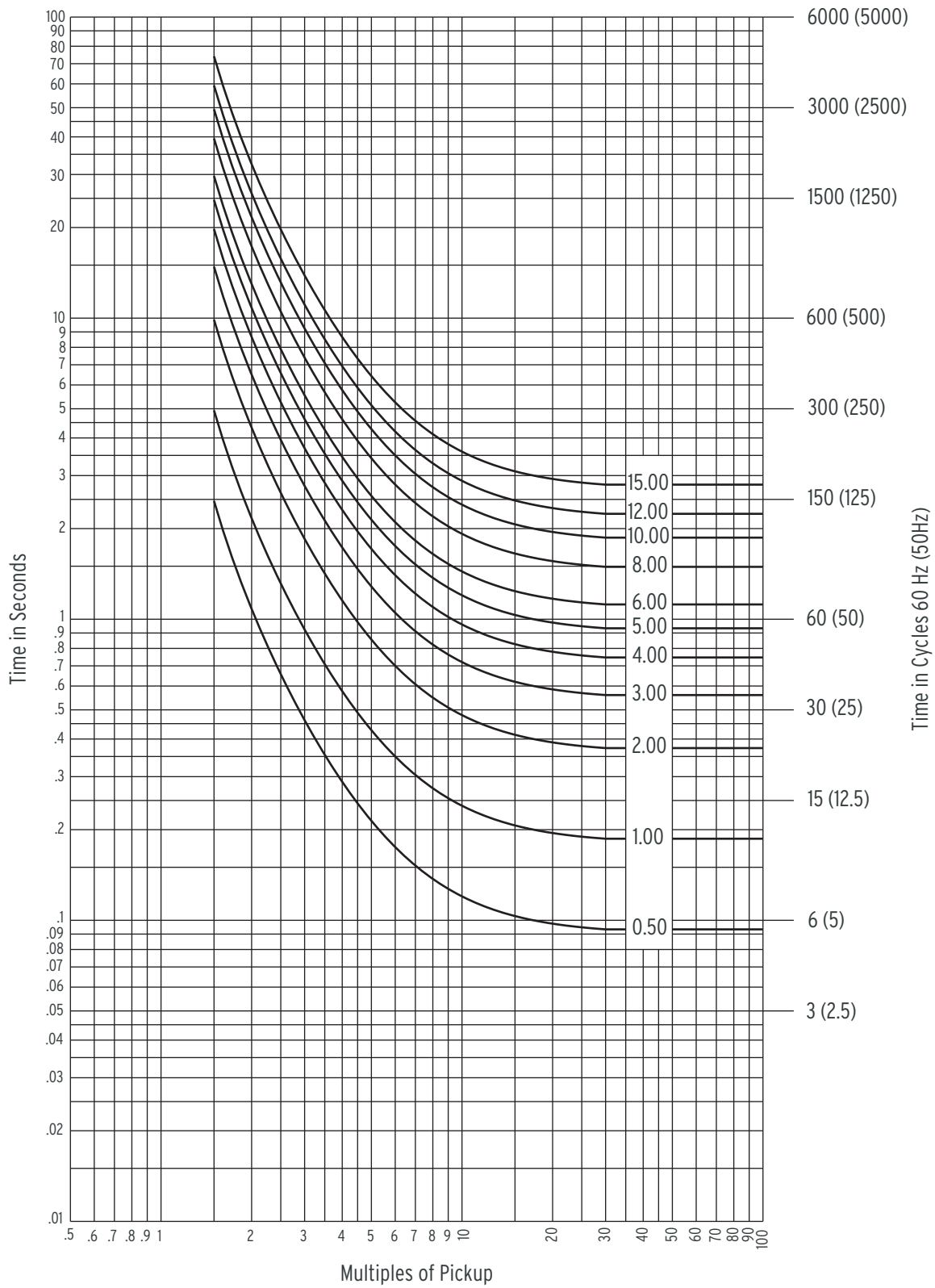
Figure 4.58 U.S. Inverse Curve: U2
