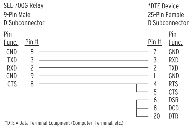
Figure 7.11 SEL Cable C227A–SEL-700G to DTE Device
