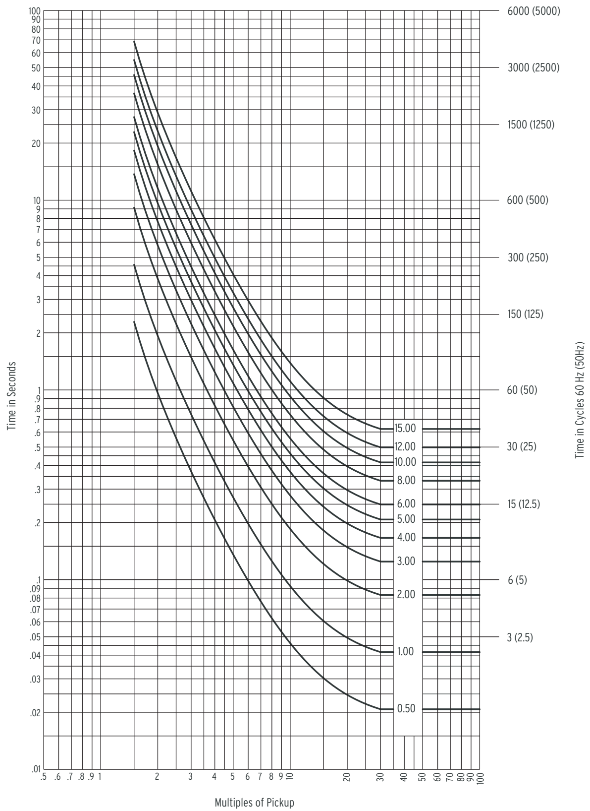
Figure 4.60 U.S. Extremely Inverse Curve: U4
