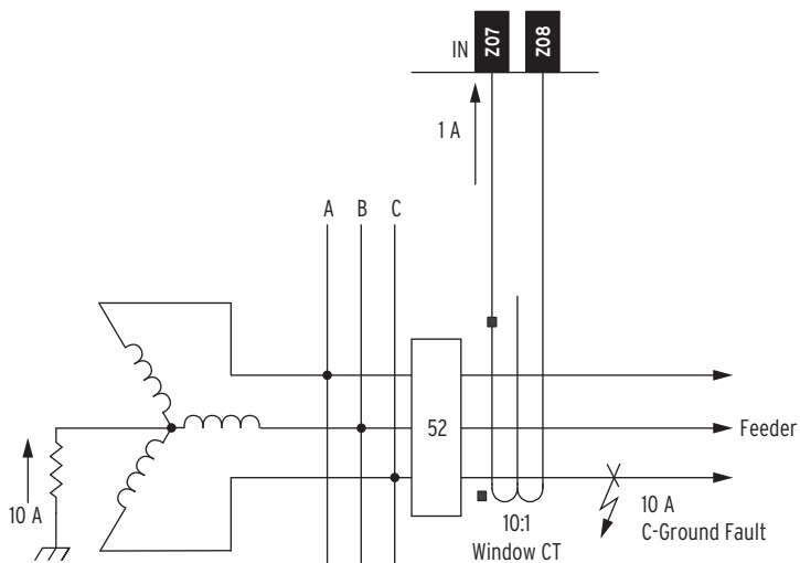
Figure 4.52 Ground Fault Protection Using Core-Balance CT
