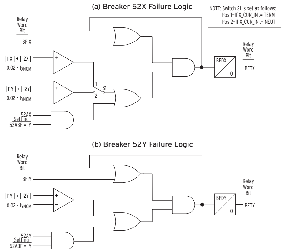
Figure 4.135 Breaker Failure Logic
