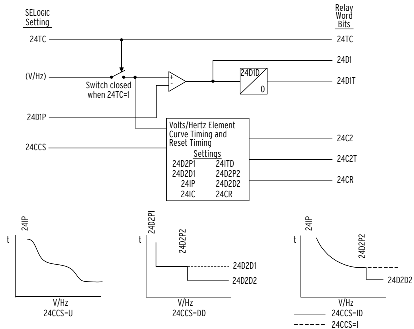
Figure 4.33 Volts/Hertz Element Logic
