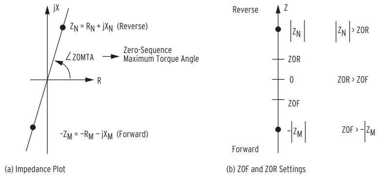
Figure 4.87 Zero-Sequence Impedance Plot for Solidly-Grounded, Mostly Inductive System
