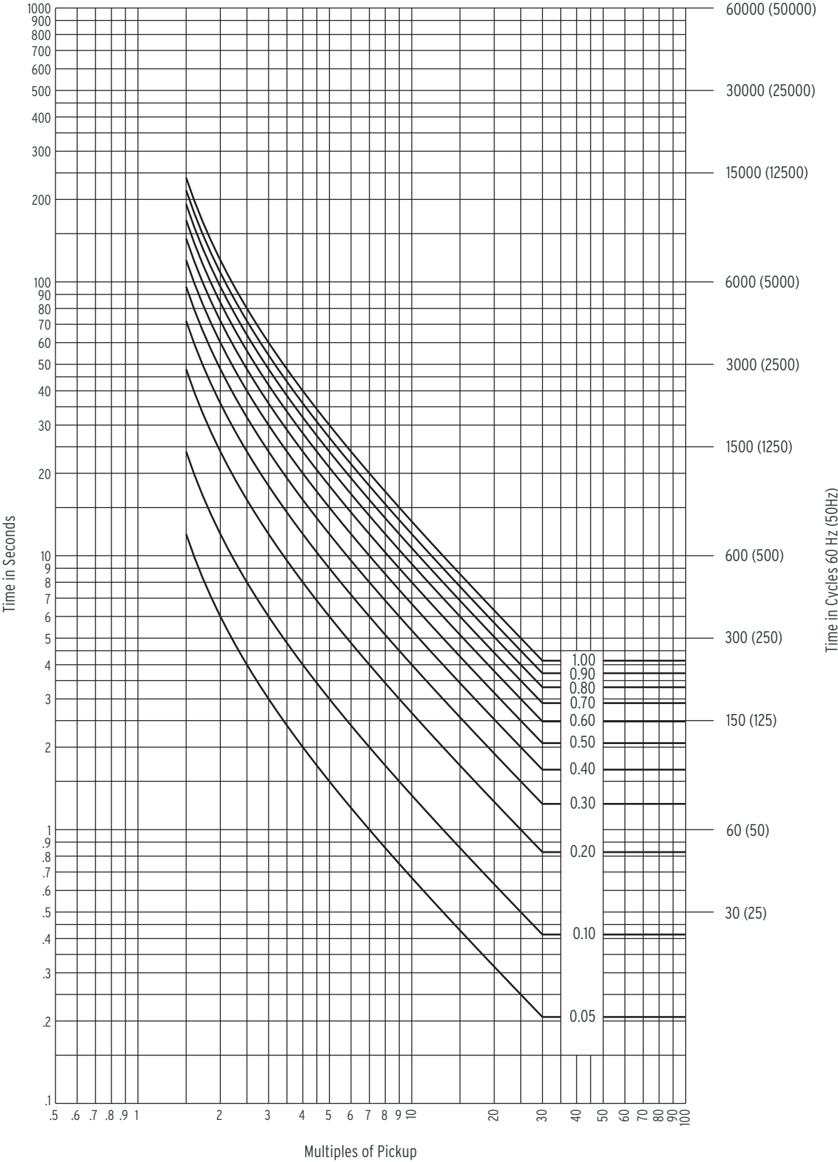
Figure 4.65 IEC Long-Time Inverse Curve: C4
