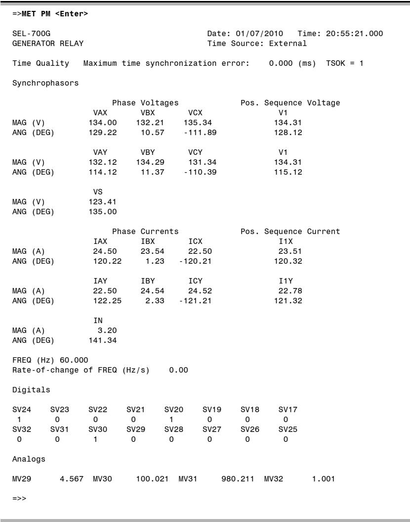
Figure H.4 Sample MET PM Command Response
