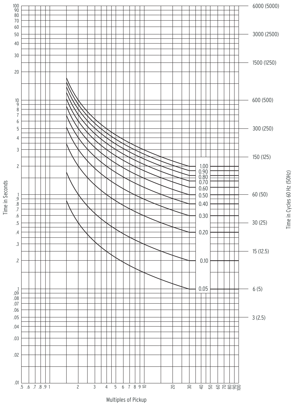
Figure 4.62 IEC Class A Curve (Standard Inverse): C1
