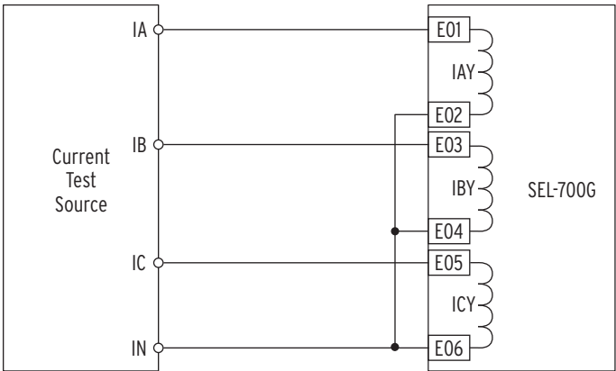
Figure 10.6 CTRY Current Source Connections
