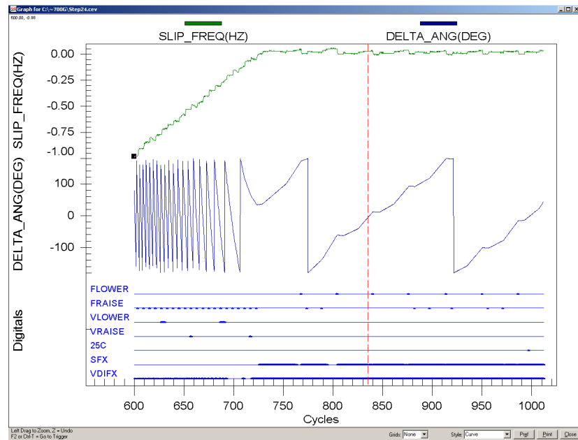
Figure 4.114 Graphical Display of Generator Autosynchronization Report
