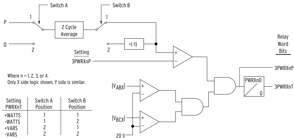
Figure 4.91 Three-Phase Power Elements Logic
