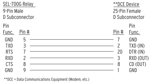
Figure 7.12 SEL Cable C222–SEL-700G to Modem
