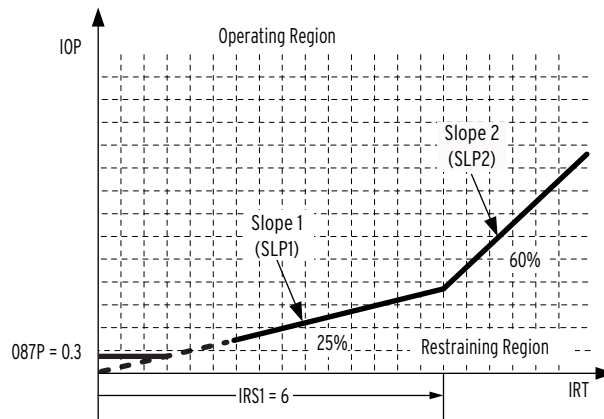
Figure 4.2 Percentage Restraint Differential Characteristic
