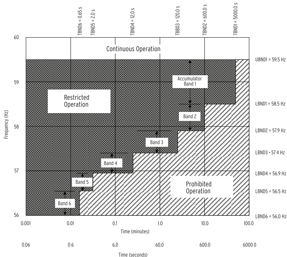
Figure 4.39 Example Turbine Operating Limitations During Abnormal Frequency
