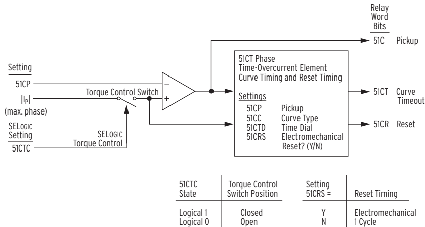
Figure 4.23 Voltage-Controlled Phase Time-Overcurrent Element 51CT
