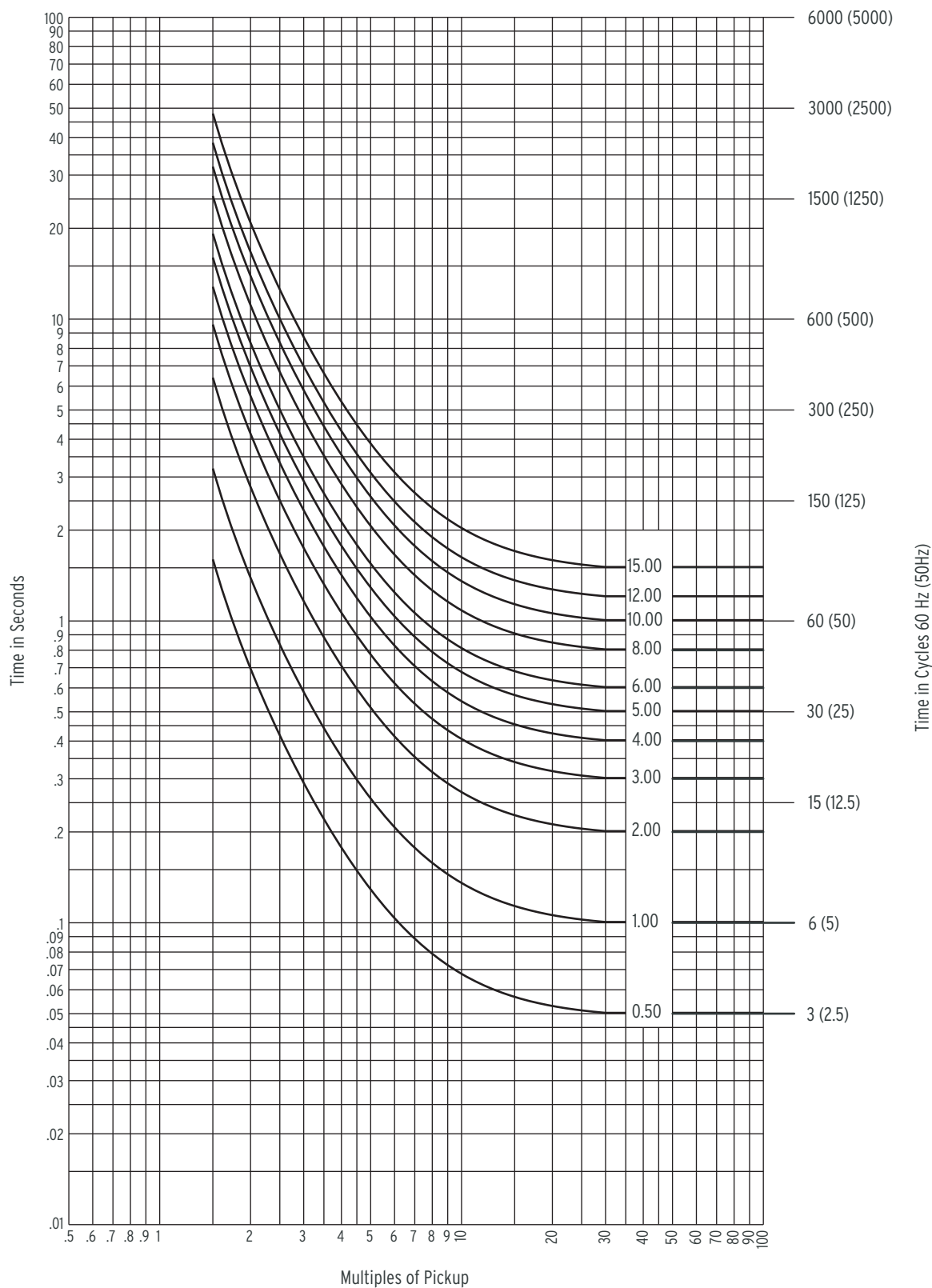
Figure 4.59 U.S. Very Inverse Curve: U3
