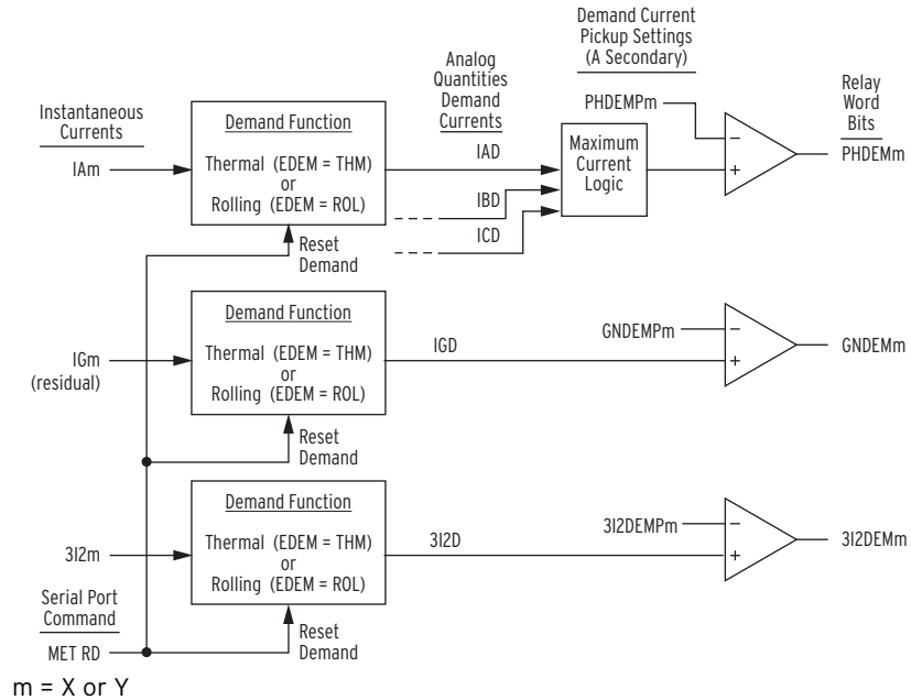
Figure 4.116 Demand Current Logic Outputs
