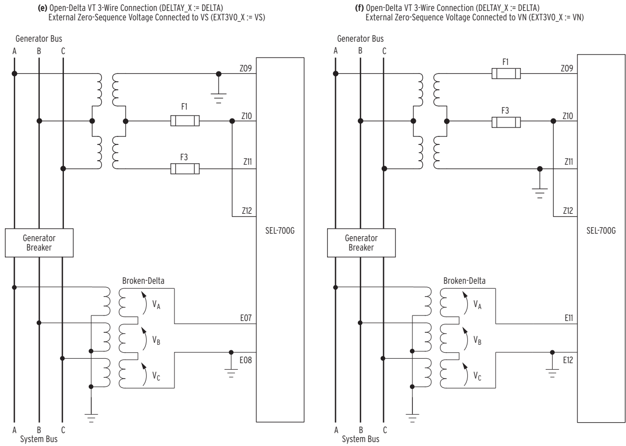
Figure 2.16 Voltage Connections
