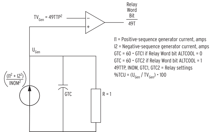
Figure 4.31 Simplified Thermal Model, Generator
