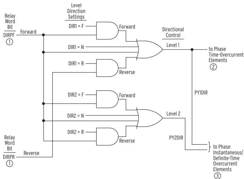
Figure 4.85 Direction Forward/Reverse Logic for Phase Overcurrent Elements
