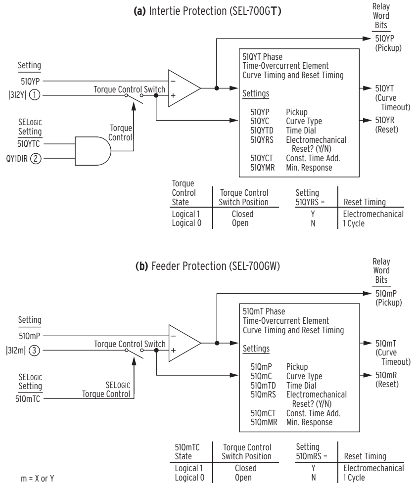
Figure 4.54 Negative-Sequence Time-Overcurrent Elements
