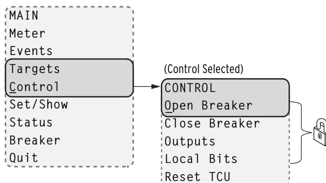
Figure 8.17 MAIN Menu and CONTROL Submenu
