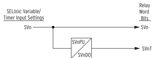
Figure 4.130 SELOGIC Control Equation Variable/Timers SV01/SV01T–SV32T
