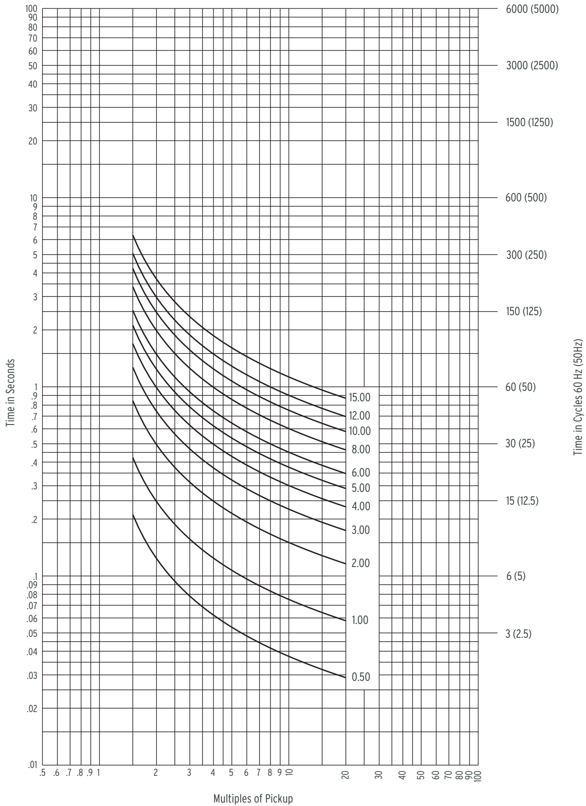
Figure 4.61 U.S. Short-Time Inverse Curve: U5
