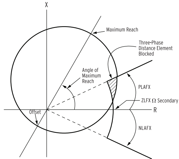
Figure 4.19 Three-Phase Distance Element Operating Characteristics
