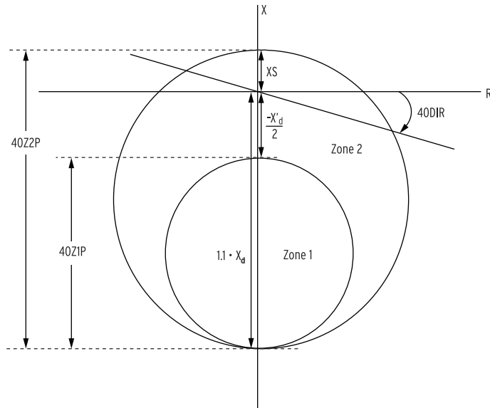
Figure 4.28 Loss-of-Field Element Operating Characteristic, Positive Zone 2 Offset
