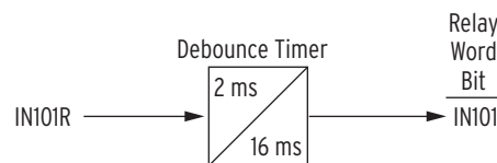
Figure 4.141 AC Mode Processing
