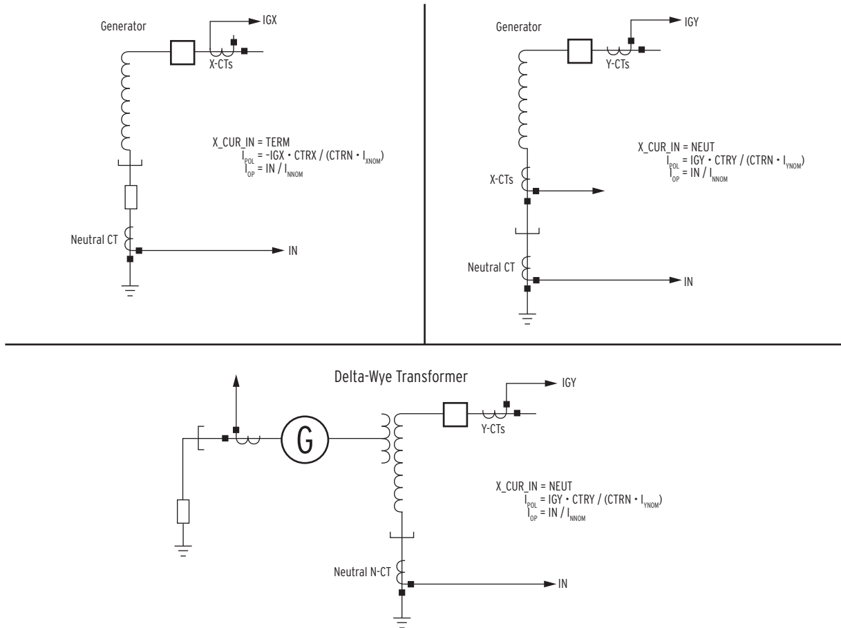
Figure 4.15 Effect of X_CUR_IN Setting on Polarizing Current
