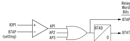
Figure 4.7 Differential Current Alarm Logic Diagram
