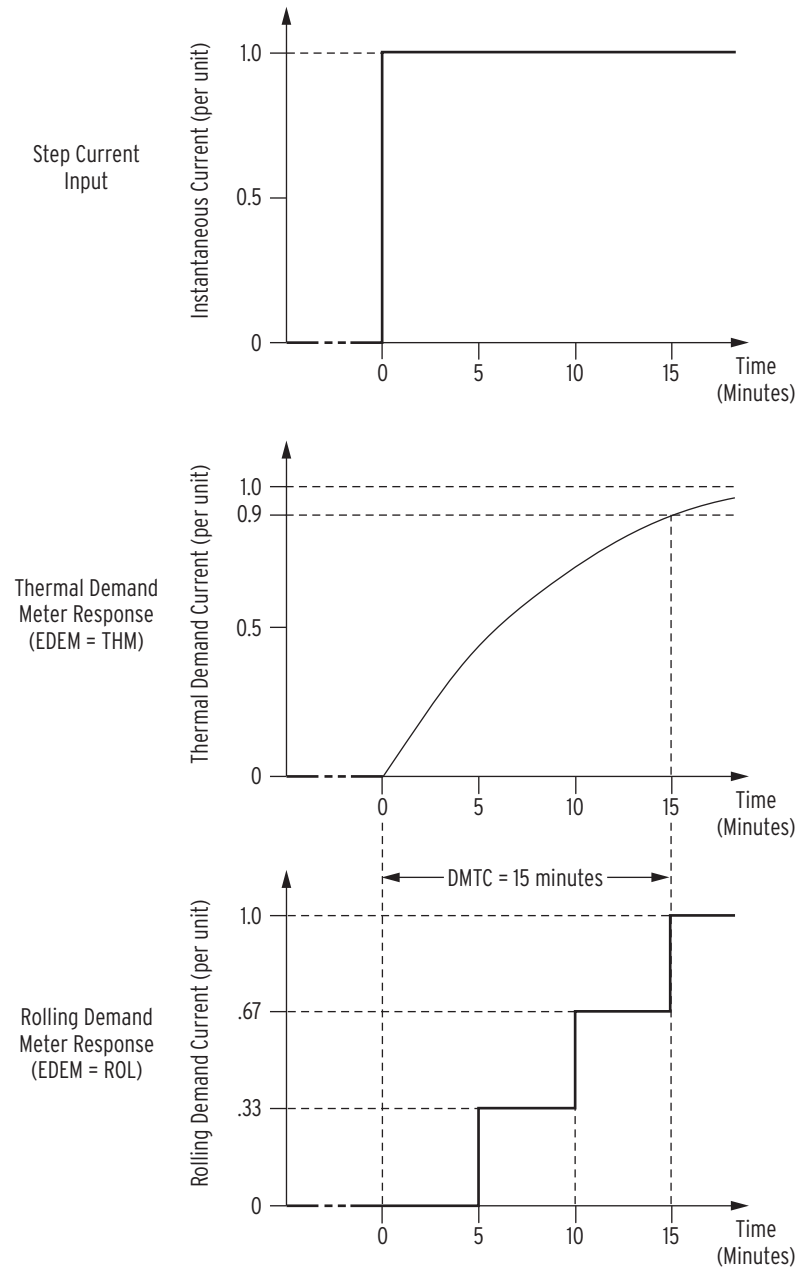
Figure 4.117 Response of Thermal and Rolling Demand Meters to a Step Input (Setting DMTC = 15 minutes)
