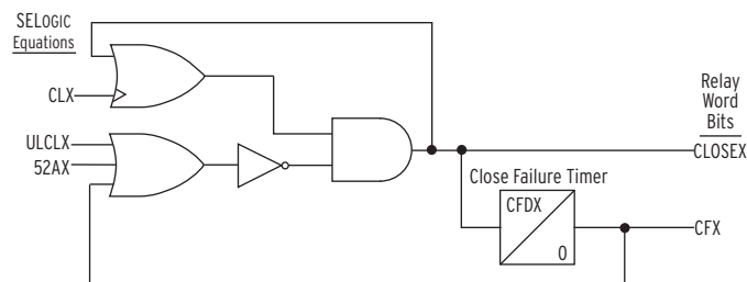
Figure 4.125 Close Logic
