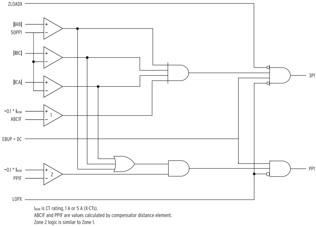
Figure 4.21 Zone 1 Compensator Element Logic
