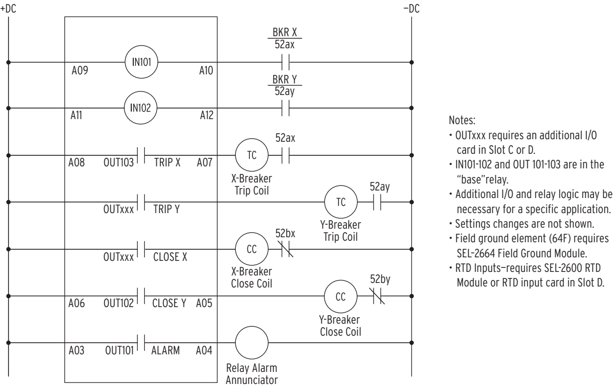
Figure 2.29 SEL-700GW Typical DC External Connections
