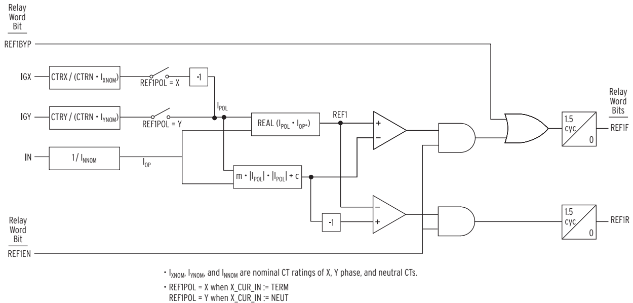
Figure 4.13 REF Directional Element
