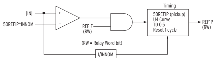
Figure 4.14 REF Protection Output (Extremely Inverse-Time O/C)
