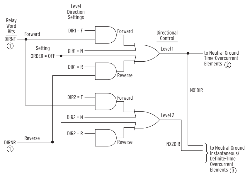
Figure 4.79 Direction Forward/Reverse Logic for Neutral-Ground Overcurrent Elements
