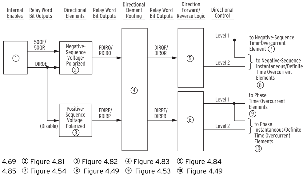
Figure 4.80 General Logic Flow of Directional Control for Negative-Sequence and Phase Overcurrent Elements
