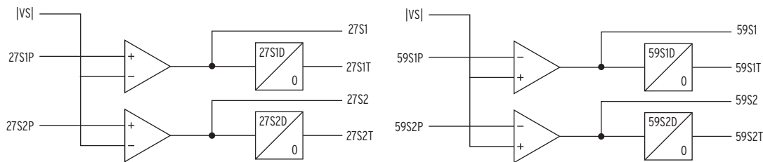
Figure 4.98 Zero-Sequence Overvoltage Elements (59G)
