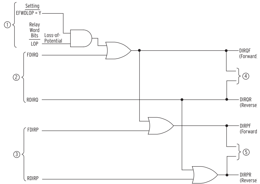
Figure 4.83 Routing of Directional Elements to Negative-Sequence and Phase Overcurrent Elements
