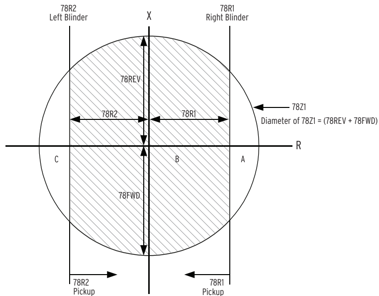
Figure 4.41 Single-Blinder Scheme Operating Characteristics
