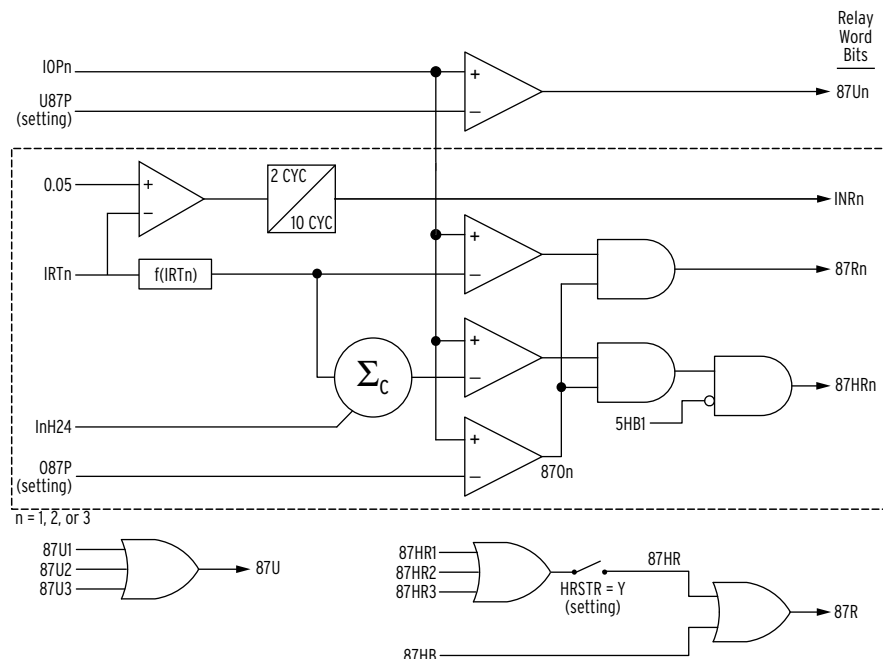
Figure 4.5 Differential Element Decision Logic
