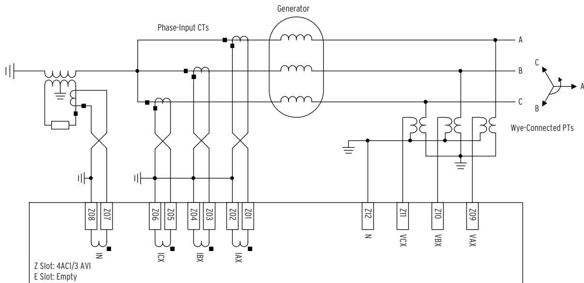
Figure 2.17 SEL-700G0 Relay AC Connection Example—High-Impedance Grounded Generator Without Current Differential Protection
