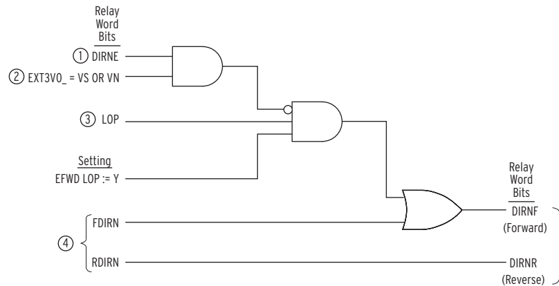
Figure 4.76 Routing of Directional Elements to Residual-Ground Overcurrent Elements
