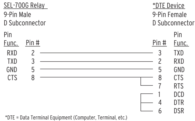
Figure 7.10 SEL Cable C234A–SEL-700G to DTE Device
