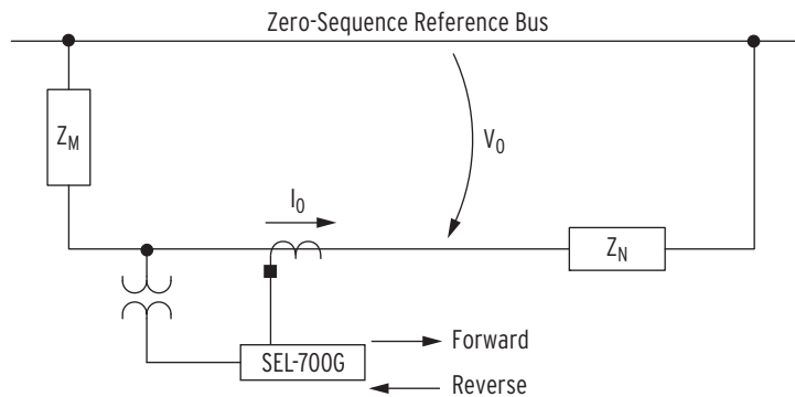
Figure 4.86 Zero-Sequence Impedance Network and Relay Polarity
