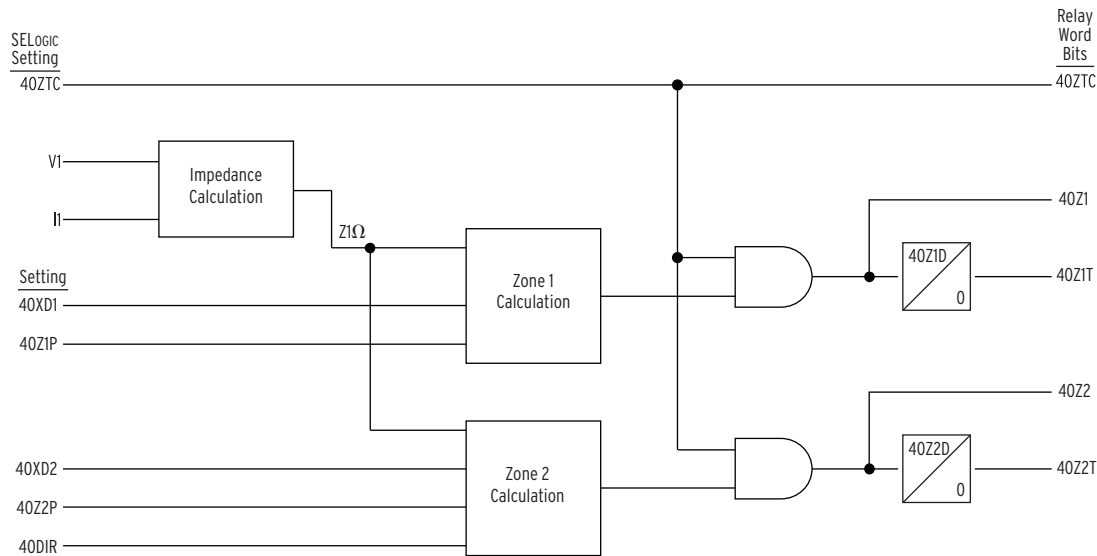
Figure 4.26 Loss-of-Field Logic Diagram
