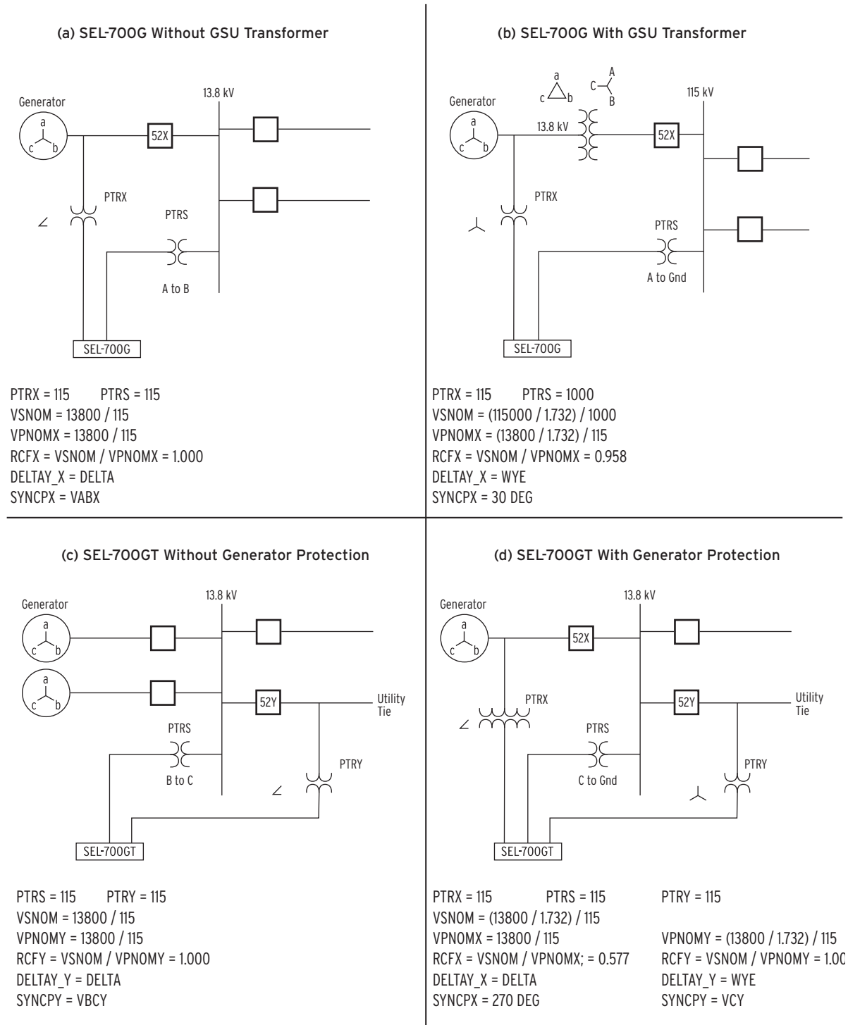
Figure 4.102 Synchronism-Check Function 25RCFX and SYNCPX/SYNCPY Setting Examples
