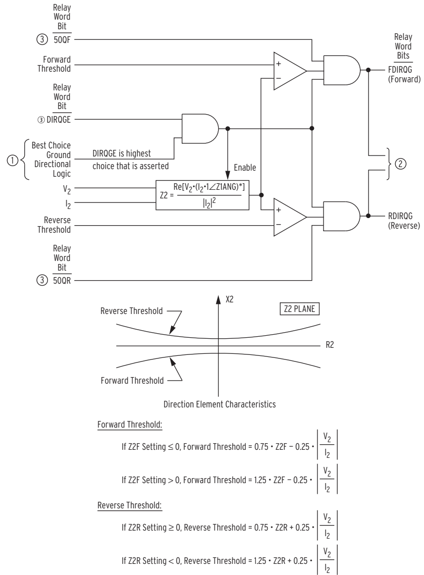
Figure 4.72 Negative-Sequence Voltage-Polarized Directional Element for Residual-Ground Overcurrent Elements
