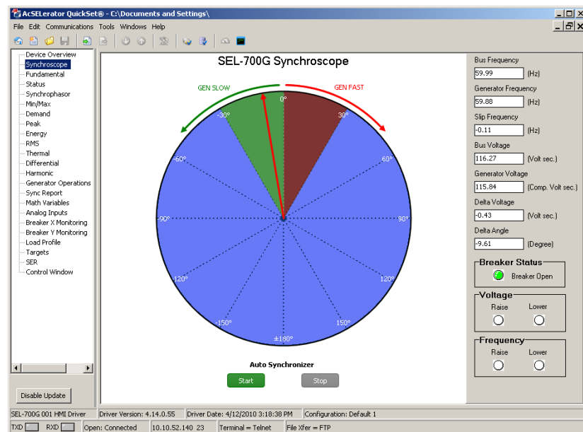
Figure 4.113 Synchroscope
