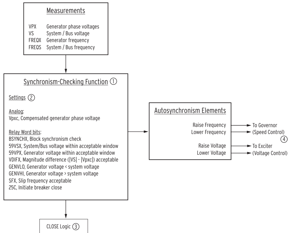
Figure 4.110 Overall Functional Block Diagram
