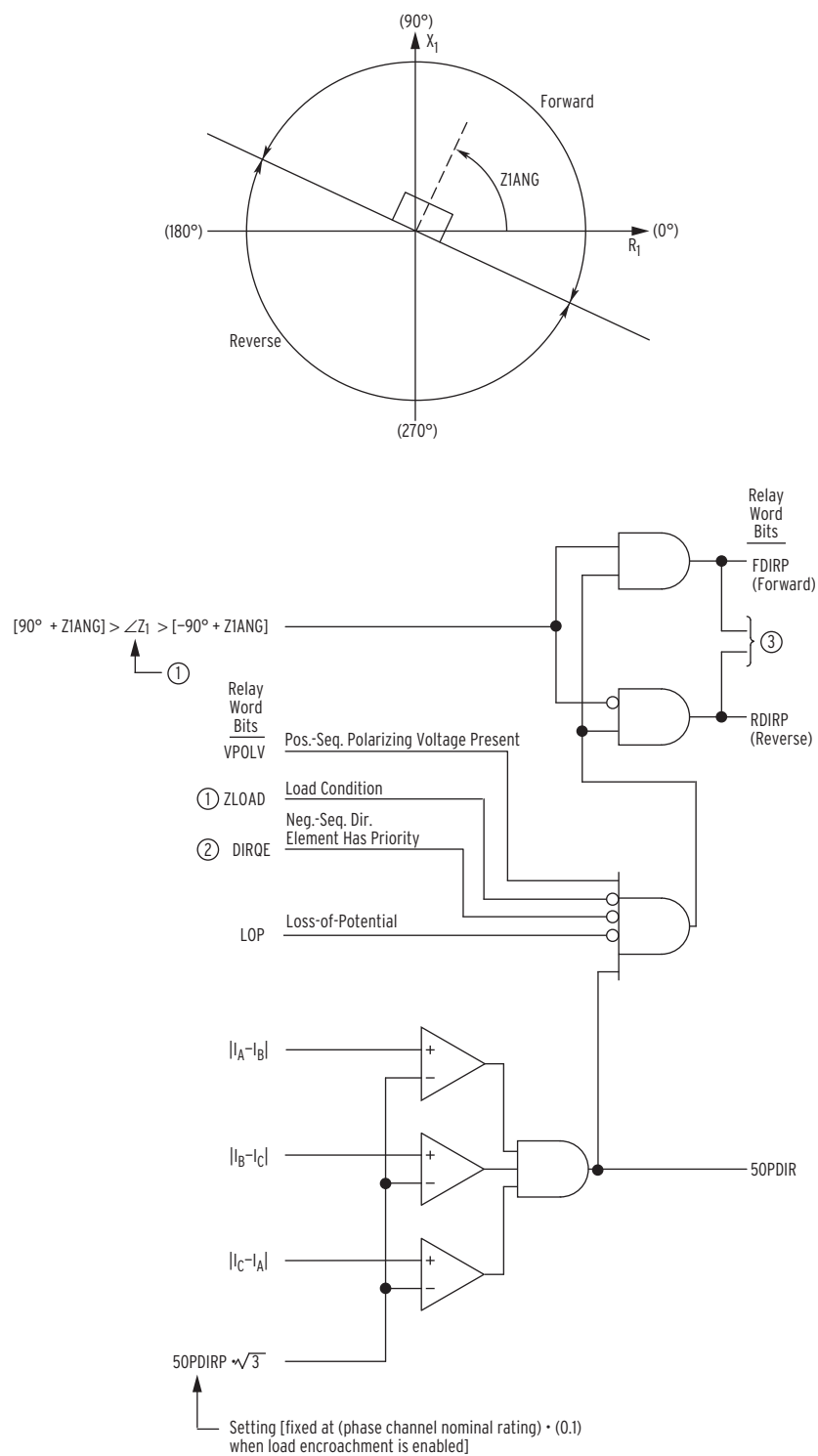
Figure 4.82 Positive-Sequence Voltage-Polarized Directional Element for Phase Overcurrent Elements
