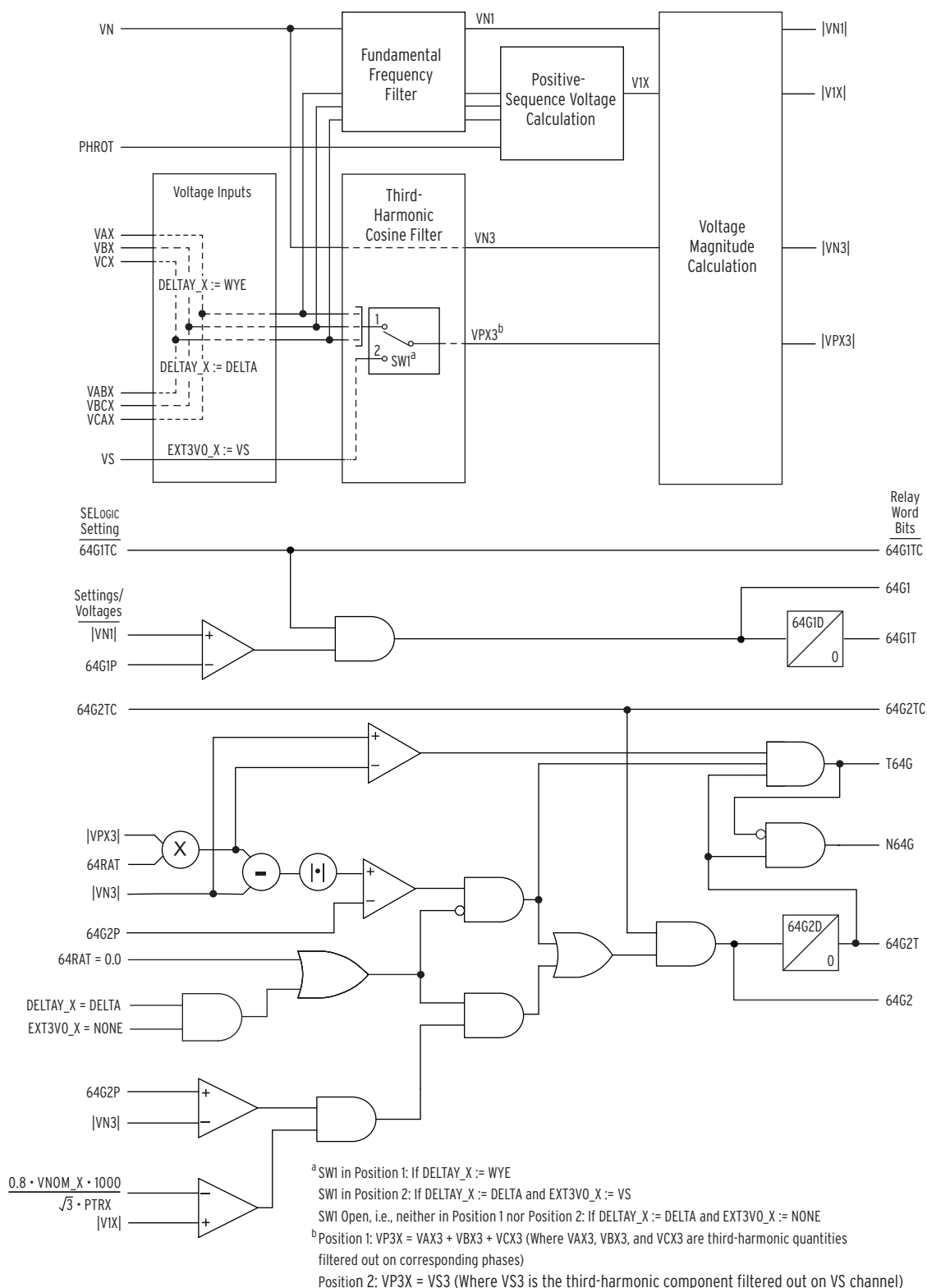
Figure 4.17 64G Logic Diagram
