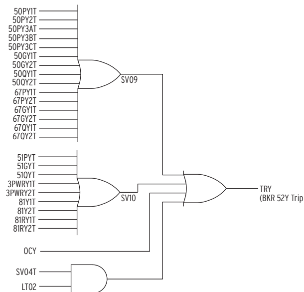
Figure 4.123 Typical Intertie Trip TR Logic (SEL-700GT)
