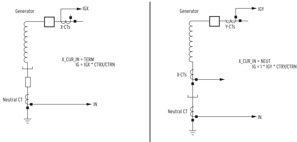
Figure 4.10 Effect of X\_CUR\_IN Setting on Residual Current ( IG )
