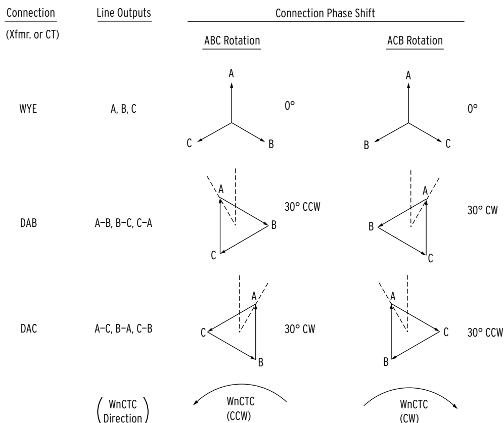
Figure 4.8 Winding Connections, Phase Shifts, and Compensation Direction
