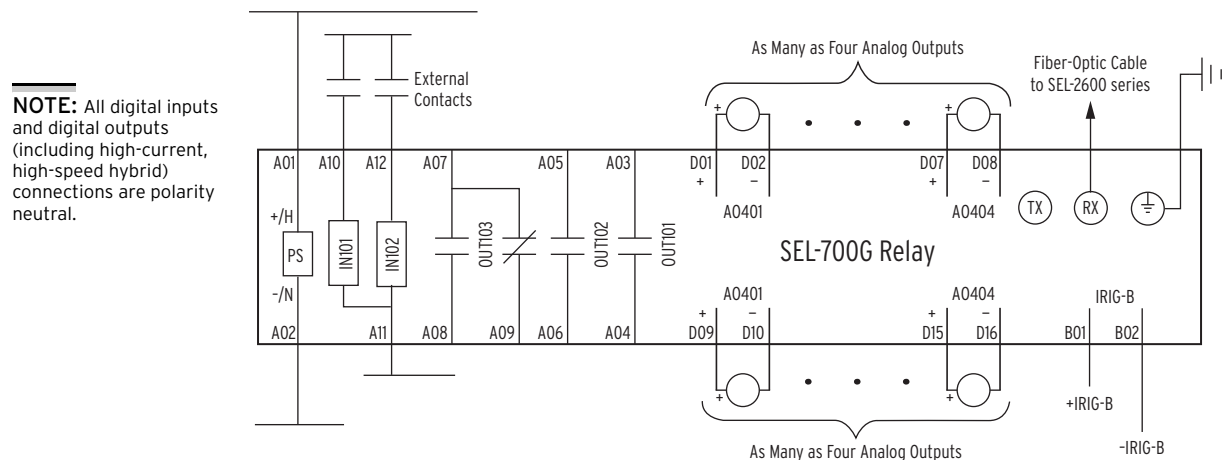
Figure 2.11 Control I/O Connections—4 AI/4 AO Option in Slot D
