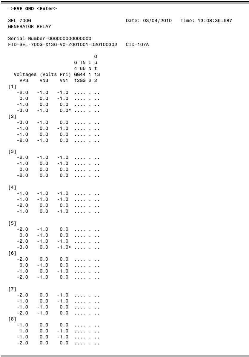
Figure 9.7 Example 15-cycle Stator Ground Event Report (EVE GND) 1/4 Cycle Resolution (Sheet 1 of 2)
