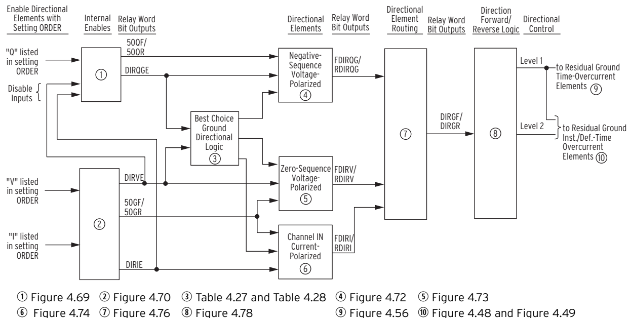
Figure 4.67 General Logic Flow of Directional Control for Residual Ground Overcurrent Elements
