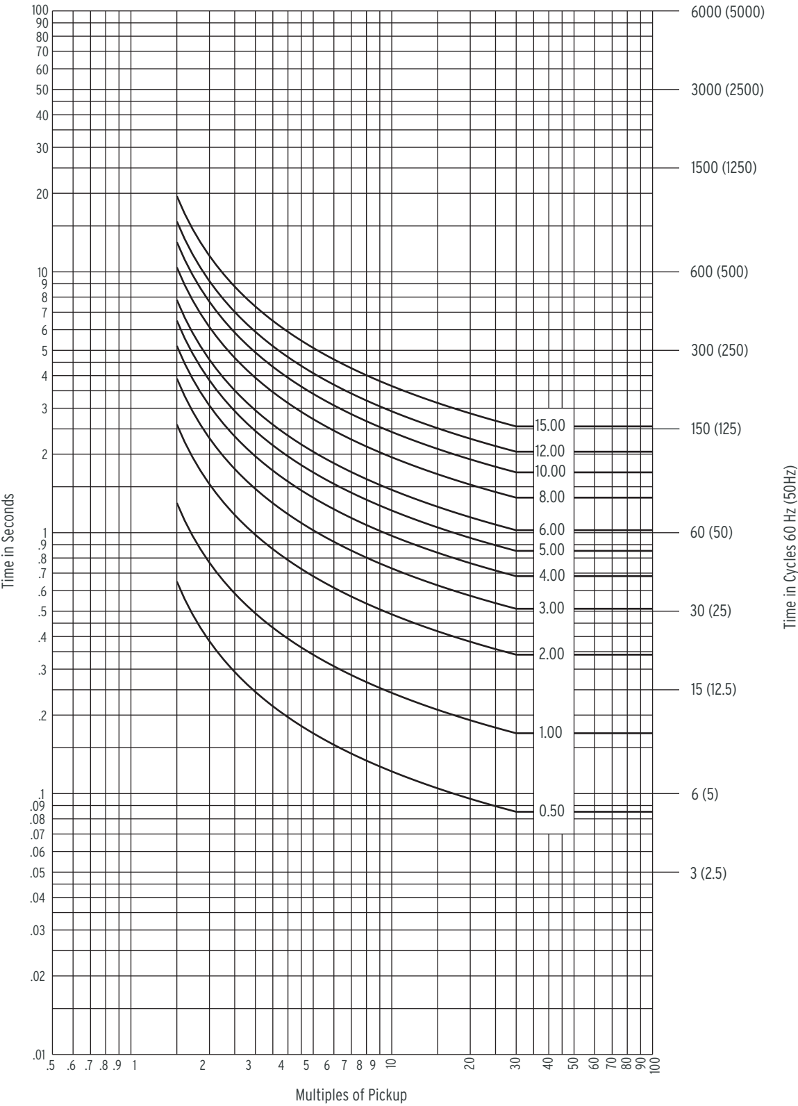
Figure 4.57 U.S. Moderately Inverse Curve: U1
