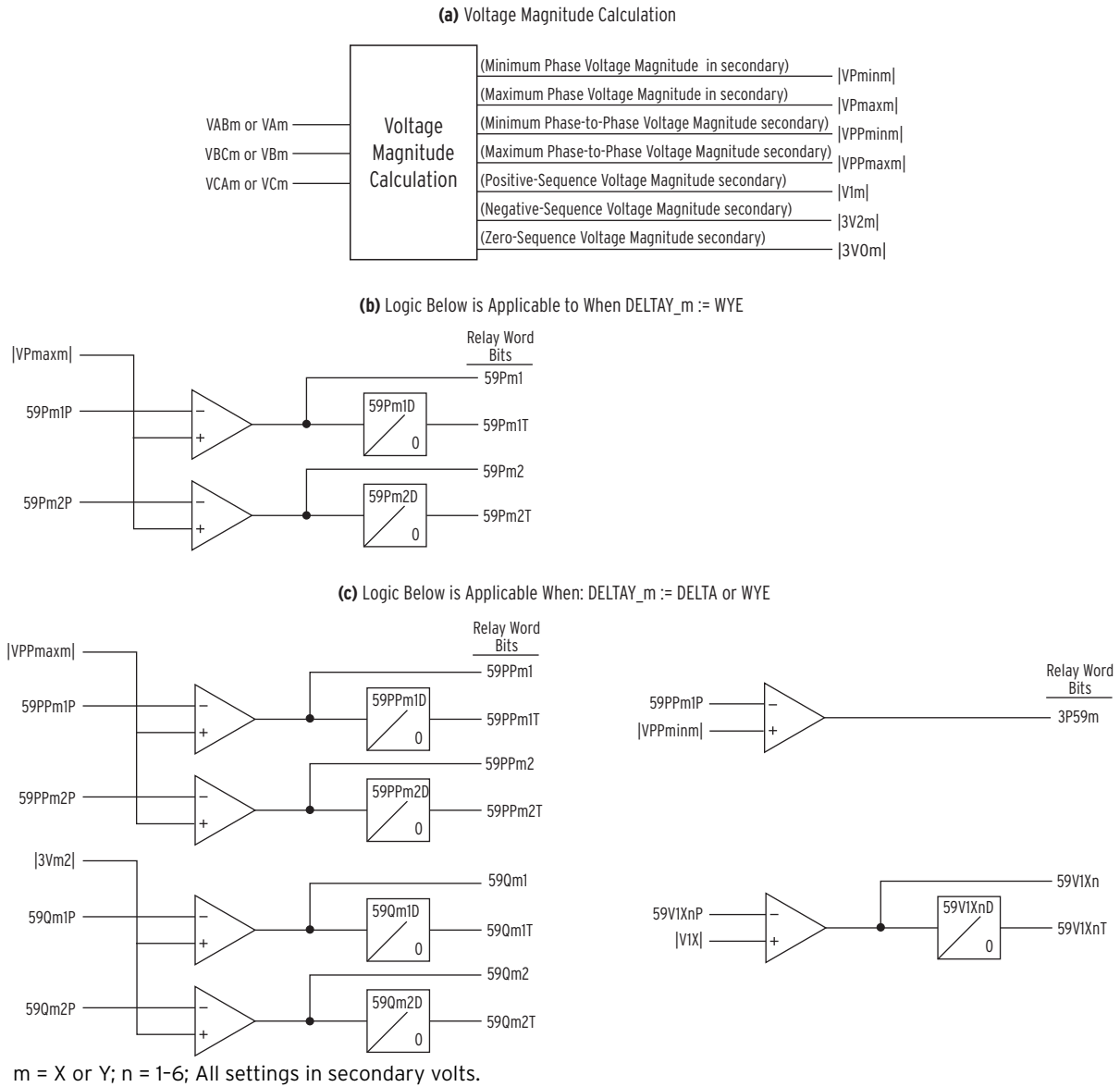
Figure 4.97 Overvoltage Element Logic
