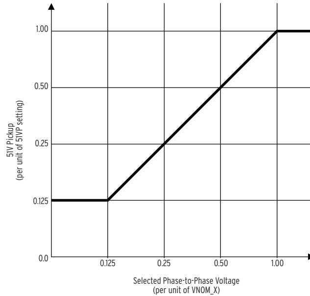
Figure 4.25 51V Element Voltage Restraint Characteristic
