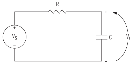
Figure 4.118 Voltage V_S Applied to Series RC Circuit
