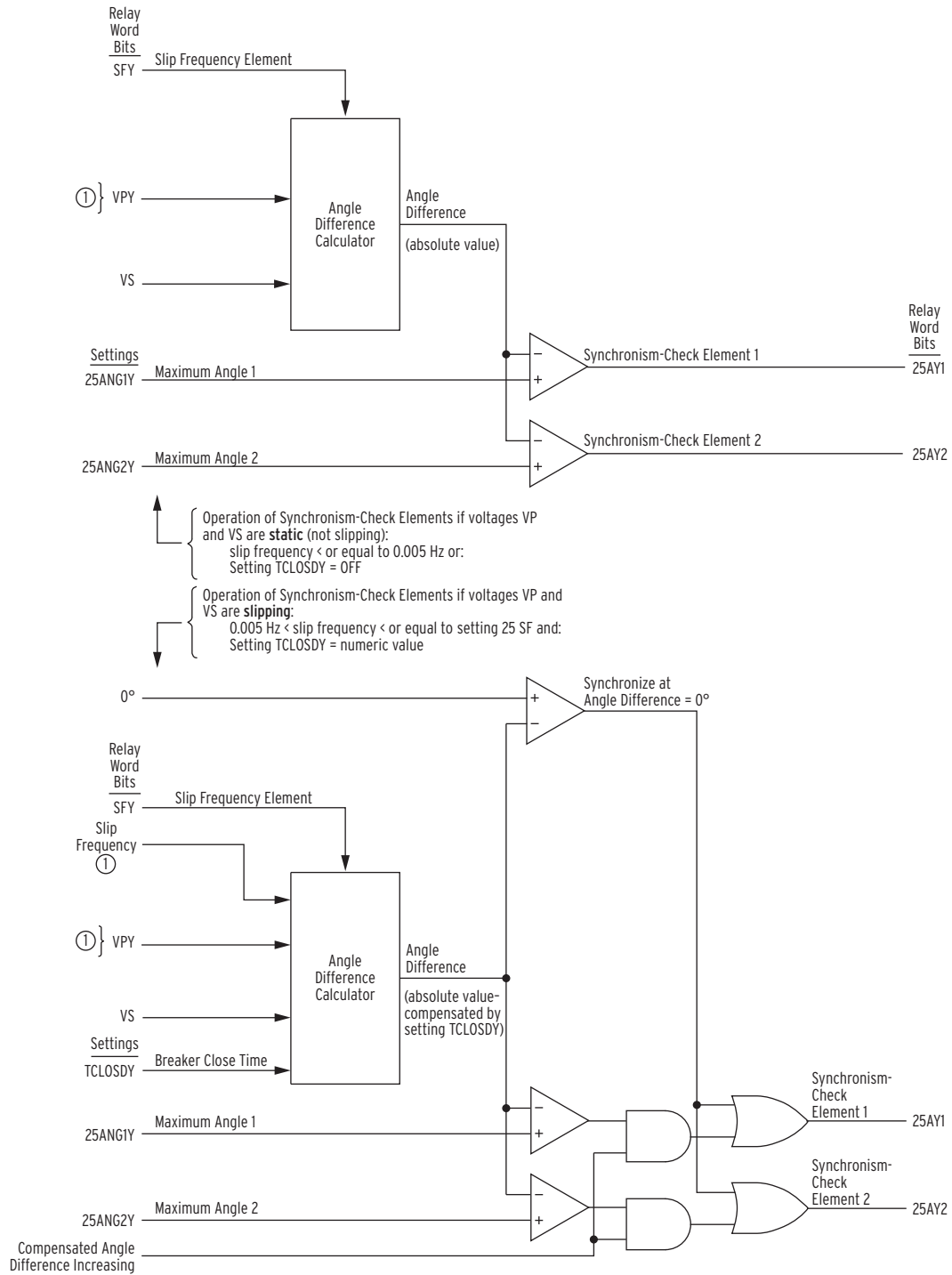
Figure 4.108 Synchronism-Check Elements
