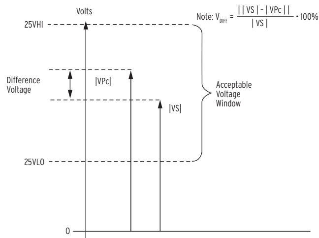
Figure 4.101 Synchronism-Check Function Voltage Element Characteristic
