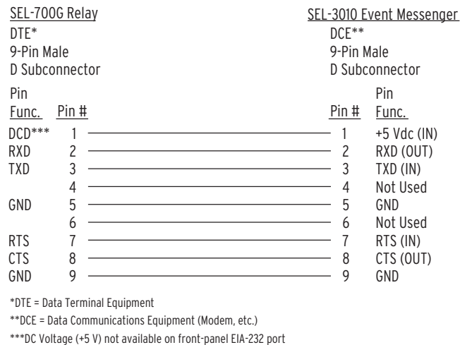
Figure 7.15 SEL Cable C387–SEL-700G to SEL-3010
