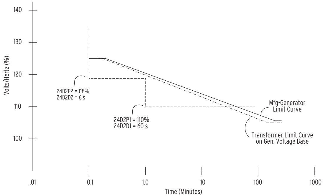
Figure 4.34 Dual-Level Volts/Hertz Time-Delay Characteristic 24CCS = DD
