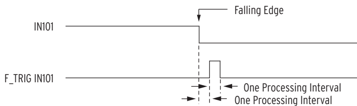
Figure 4.131 Result of Falling-Edge Operator on a Deasserting Input
