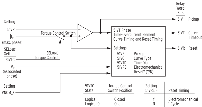
Figure 4.24 Voltage-Restrained Phase Time-Overcurrent Element 51VT
