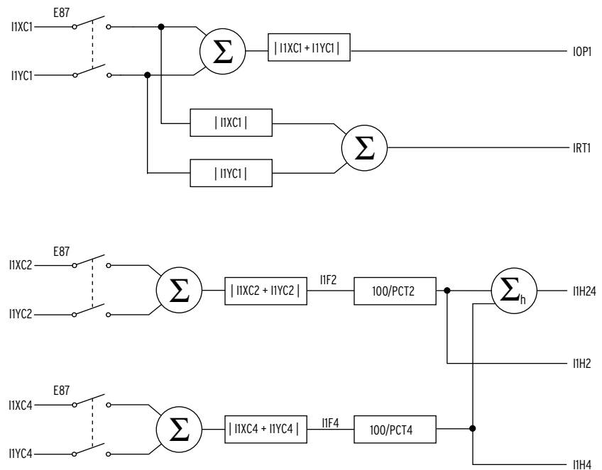
Figure 4.4 Differential Element (87-1) Quantities
