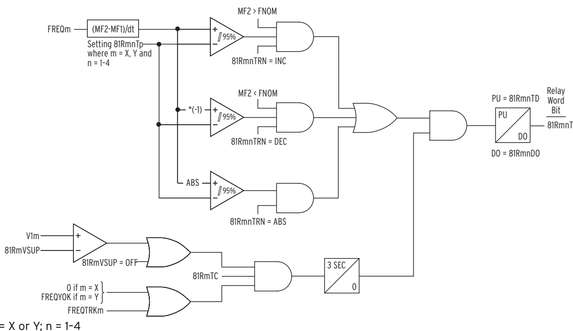
Figure 4.95 81R Frequency Rate-of-Change Scheme Logic
