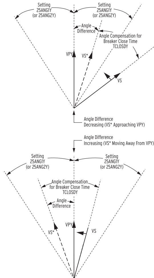
Figure 4.109 Angle Difference Between VPY and VS Compensated by Breaker Close Time ( f_{PY} < f_S and VPY Shown as Reference in This Example)
