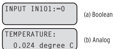
Figure 4.152 Front-Panel Display for an Entry in (a) Boolean Name and Alias Strings and (b) Analog Name, User Text and Formatting Strings, and Engineering Units
