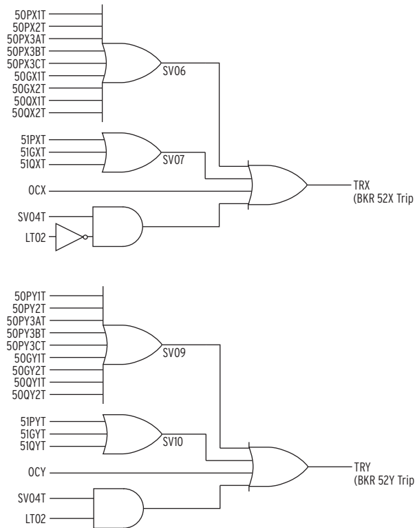
Figure 4.124 Typical Feeder Trip TR Logic (SEL-700GW)
