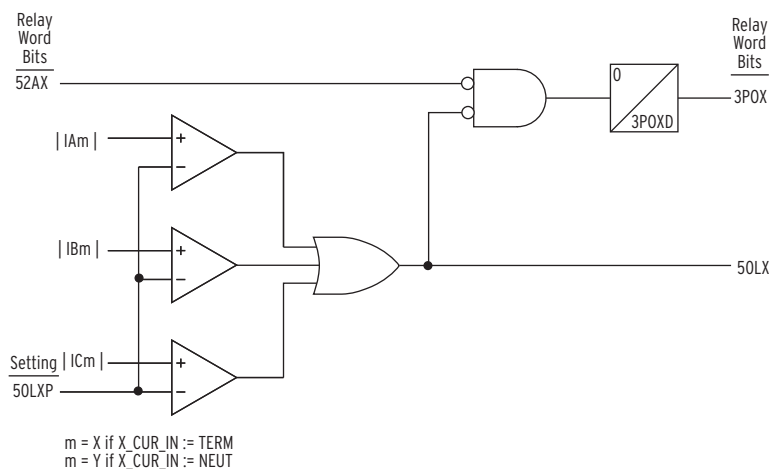
Figure 4.119 Pole Open Logic Diagram, Breaker 52X
