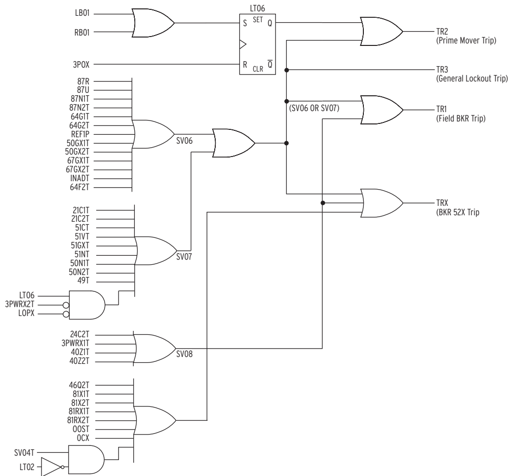
Figure 4.122 Typical Generator Trip TR Logic (SEL-700GO, SEL-700G1, SEL-700GT)
