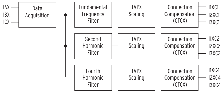
Figure 4.3 Winding X Compensated Currents
