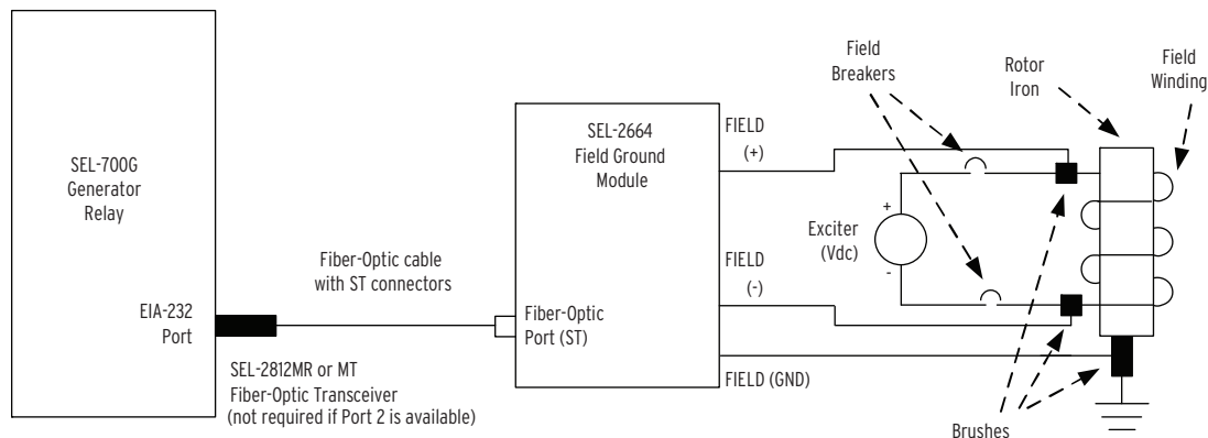
Figure 2.31 Field Ground Protection With an SEL-700G Relay
