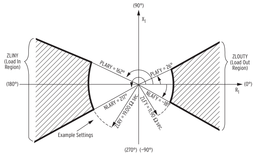
Figure 4.90 Load-Encroachment Logic for Y Side
