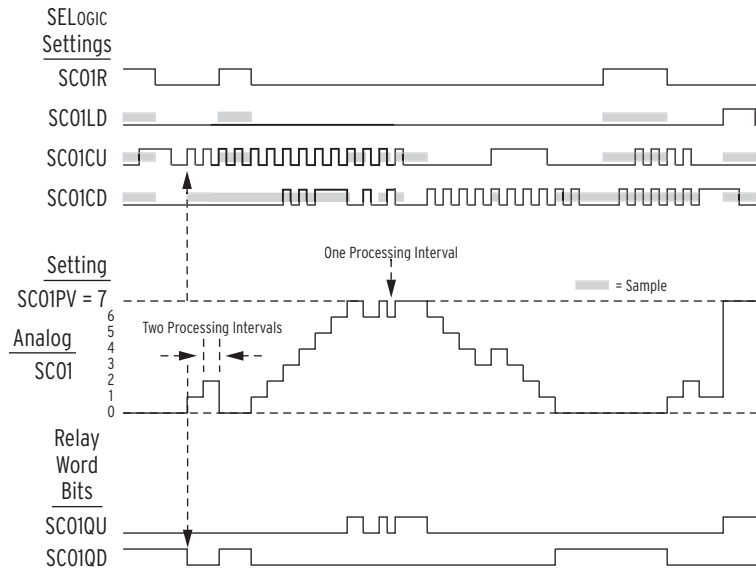
Figure 4.134 Example of the Effects of the Input Precedence
