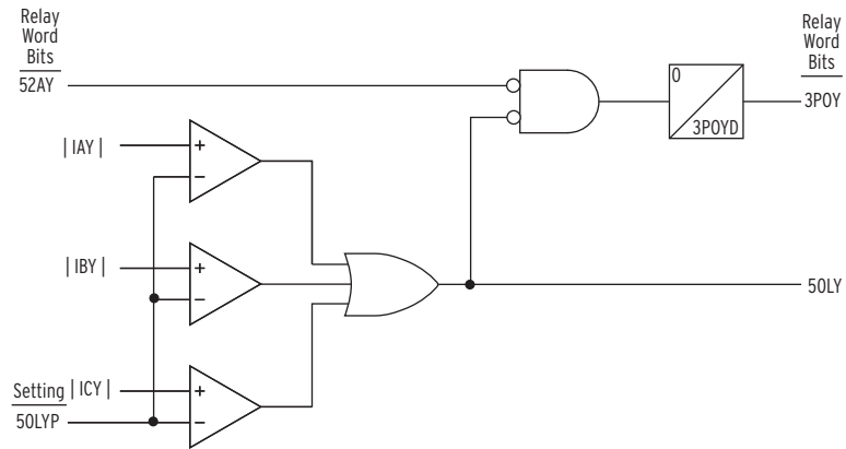
Figure 4.120 Pole Open Logic Diagram, Breaker 52Y
