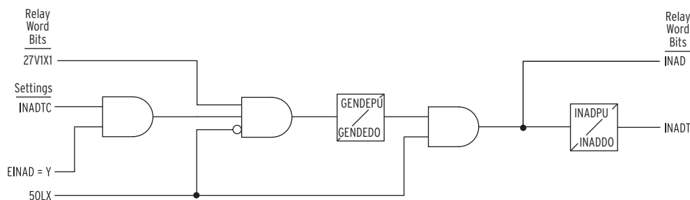
Figure 4.47 Inadvertent Energization Logic Diagram
