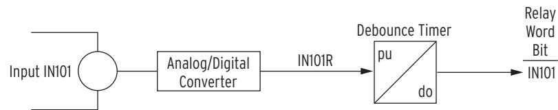
Figure 4.140 DC Mode Processing
