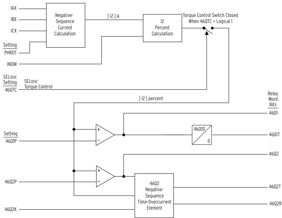
Figure 4.29 Negative-Sequence Overcurrent Element Logic Diagram
