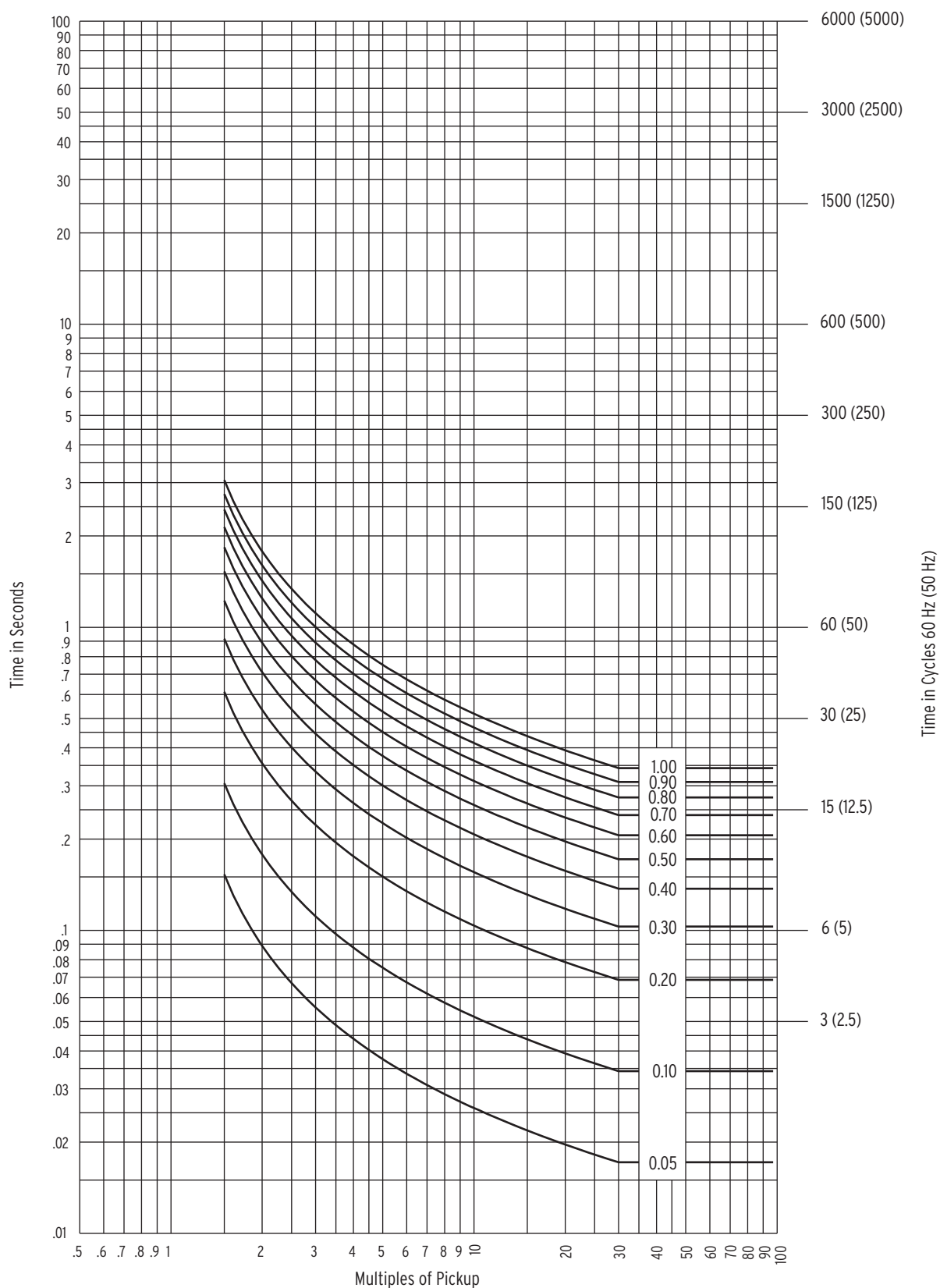
Figure 4.66 IEC Short-Time Inverse Curve: C5
