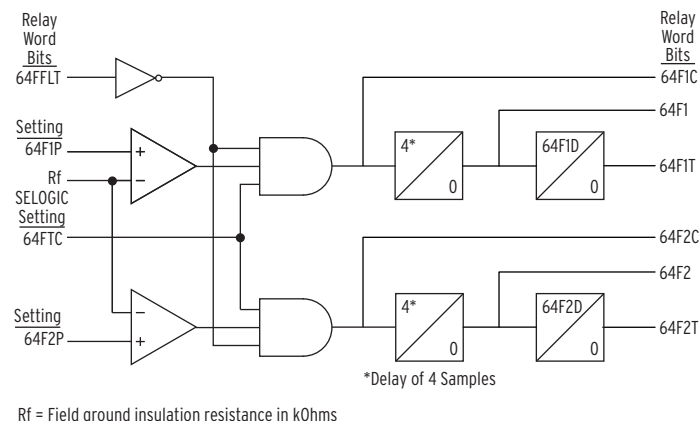
Figure 4.18 Field Ground Protection (64F) Elements Logic
