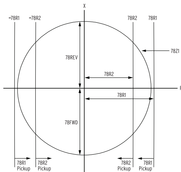
Figure 4.44 Double-Blinder Scheme Operating Characteristics
