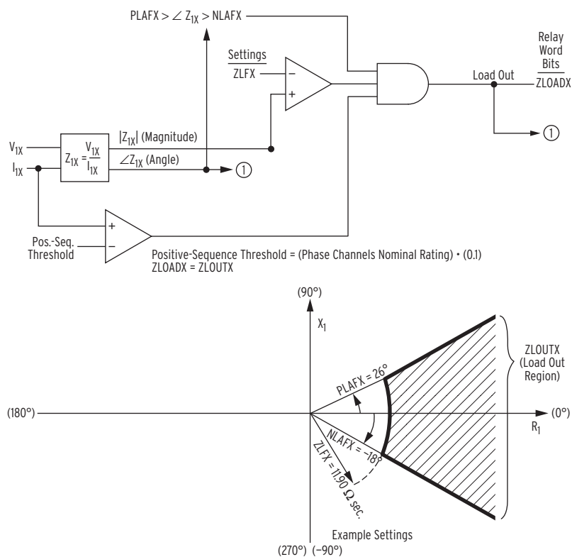
Figure 4.89 Load-Encroachment Logic for X Side
