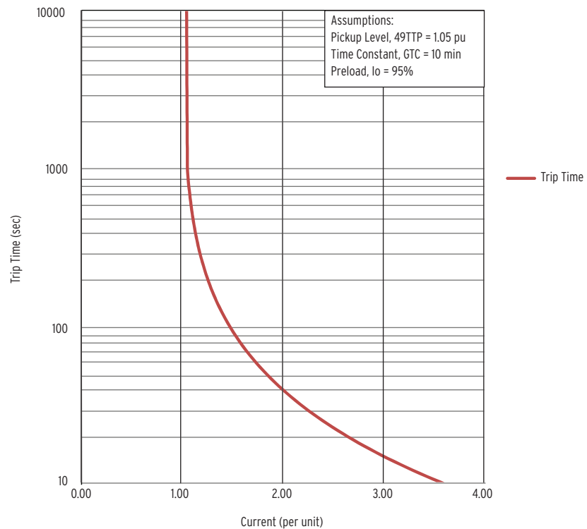
Figure 4.32 Generator Overload Curve
