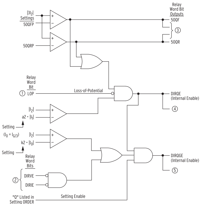
Figure 4.69 Internal Enables (DIRQE and DIRQGE) Logic for Negative-Sequence Voltage-Polarized Directional Elements
