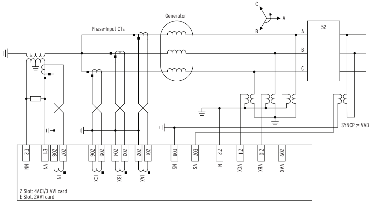
Figure 2.19 SEL-700G0+ Relay High-Impedance Grounded Generator With Synchronism Check and Without Current Differential Protection
