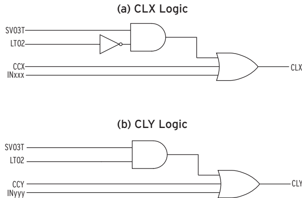
Figure 4.127 Typical Feeder Close CL Logic (SEL-700GW)
