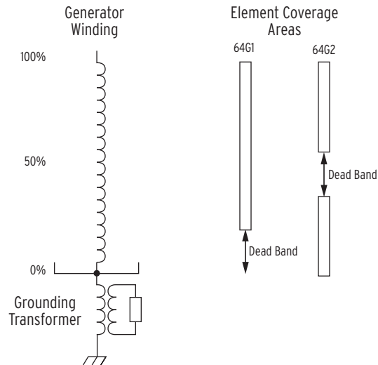
Figure 4.16 64G Element Operating Characteristic
