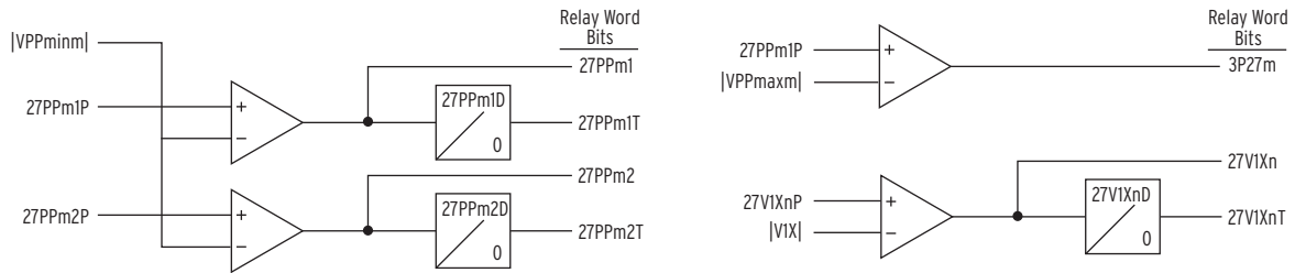
Figure 4.96 Undervoltage Element Logic
