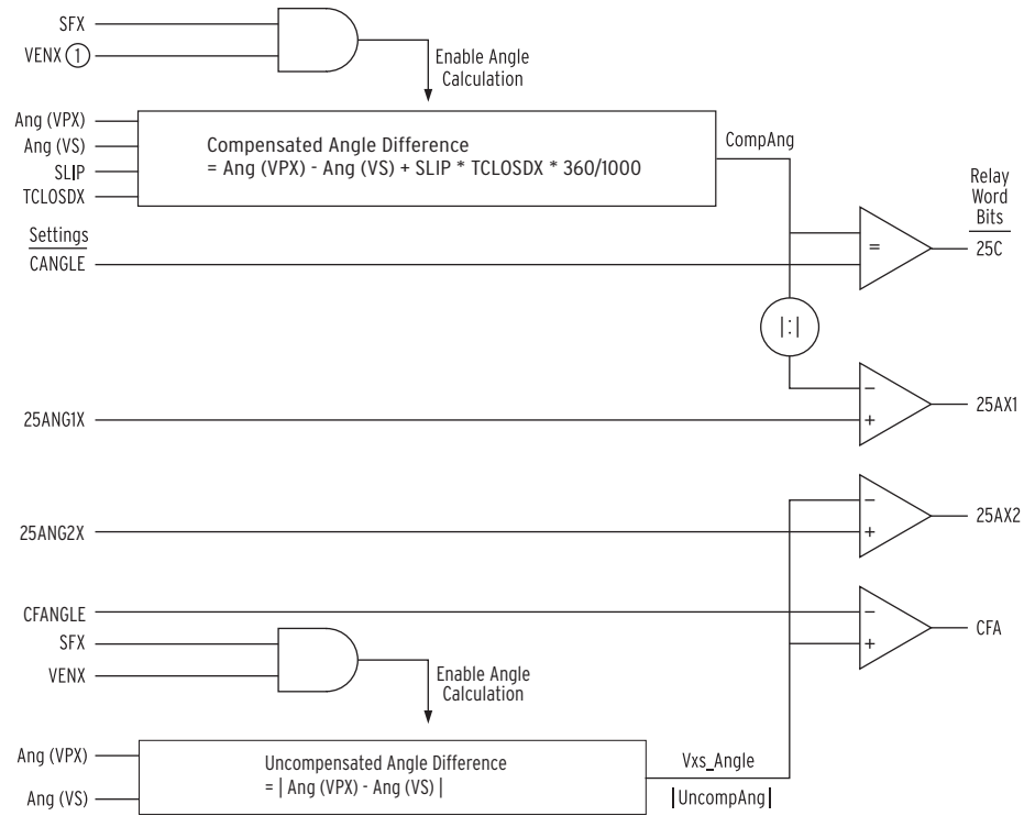
Figure 4.104 Synchronism-Check Function Angle Elements
