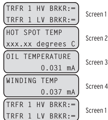
Figure 4.154 Rotating Display
