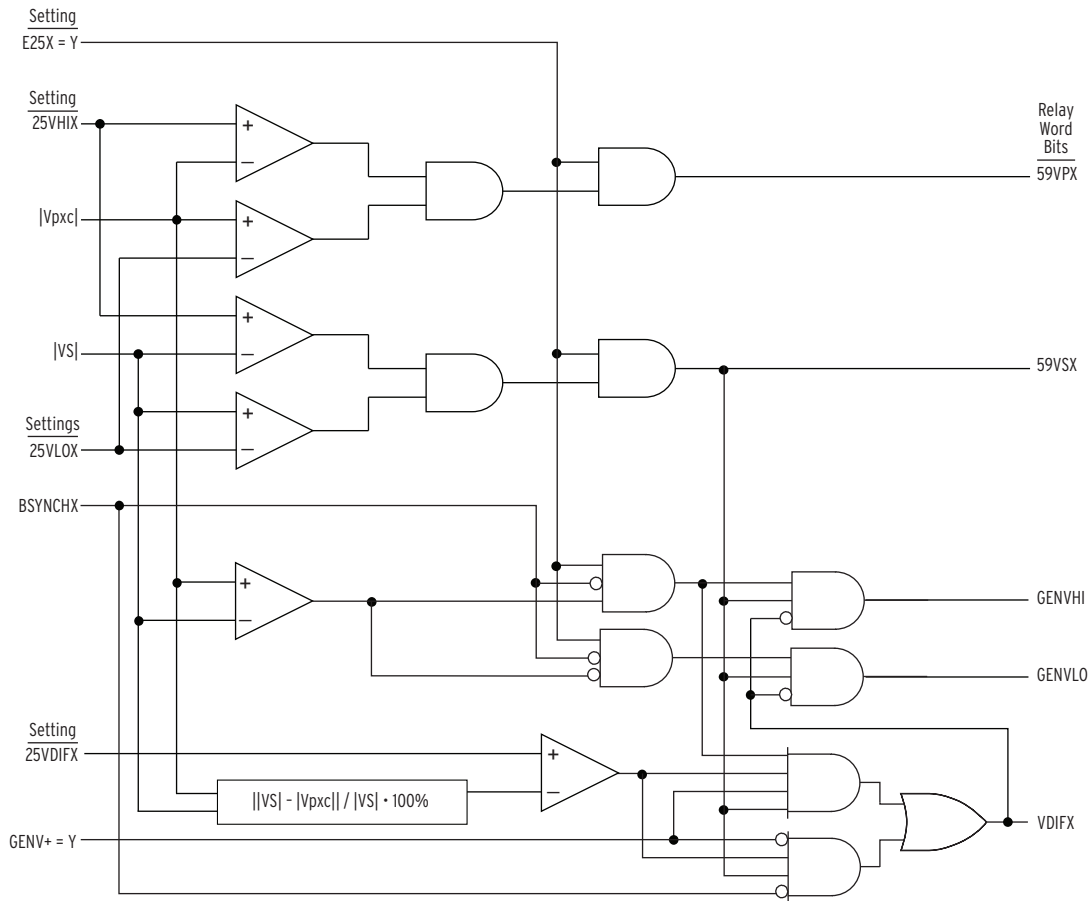
Figure 4.100 Synchronism-Check Function Voltage Elements
