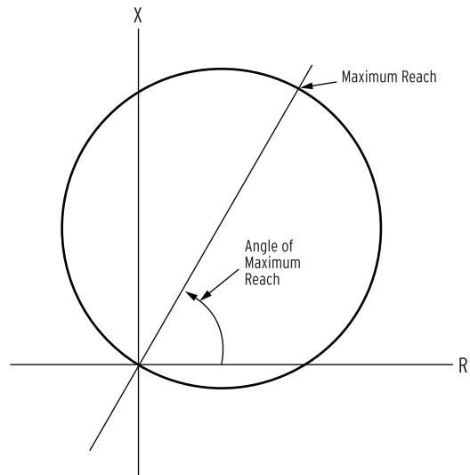
Figure 4.20 Phase-to-Phase Distance Element Operating Characteristics
