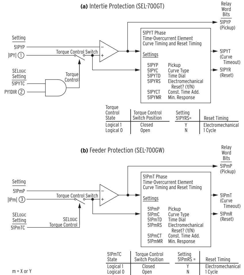
Figure 4.53 Maximum Phase Time-Overcurrent Elements
