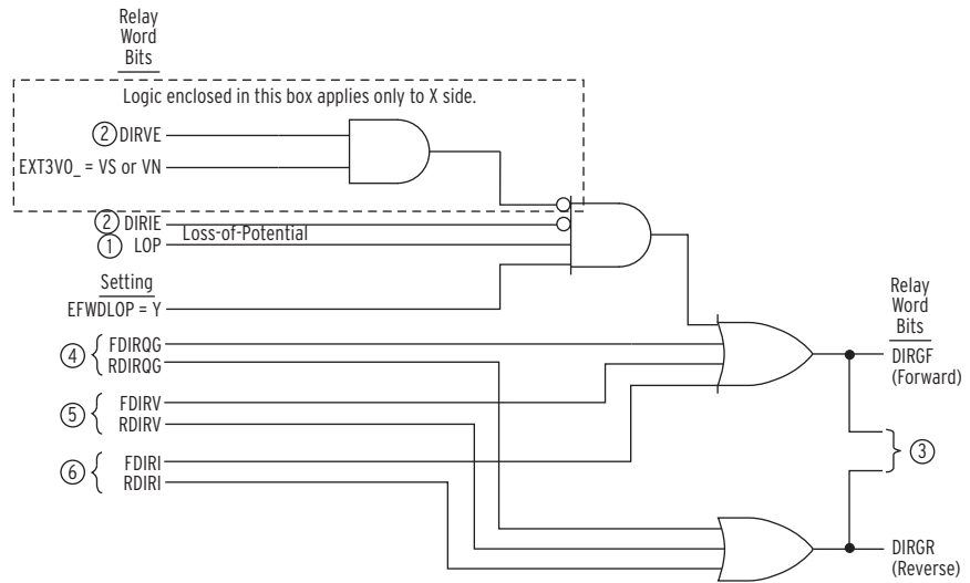
Figure 4.76 Routing of Directional Elements to Residual-Ground Overcurrent Elements
