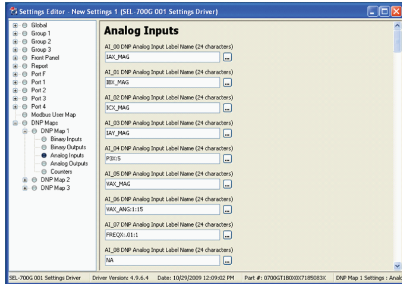
Figure D.6 Analog Input Map Entry in acSELEATOR QuickSet Software
