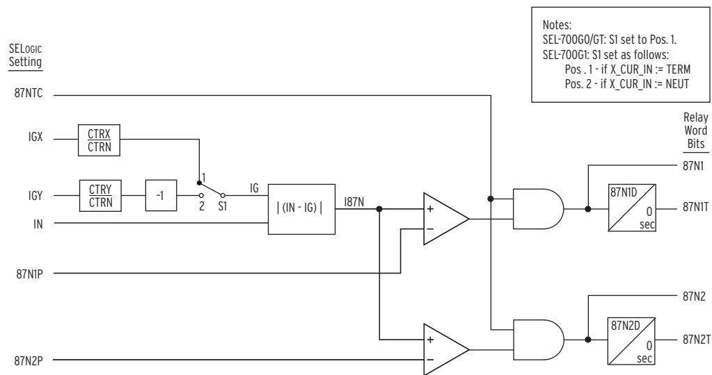
Figure 4.11 87N Element Logic Diagram
