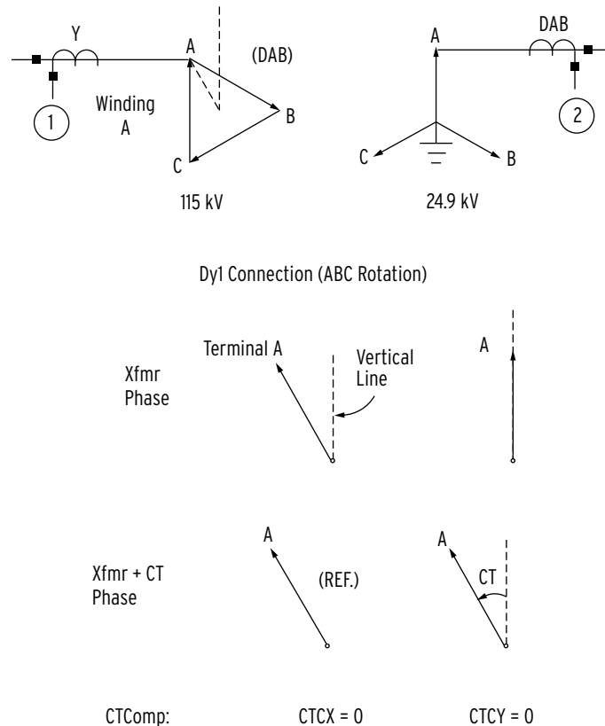
Figure 4.9 Example for CTCn Selection
