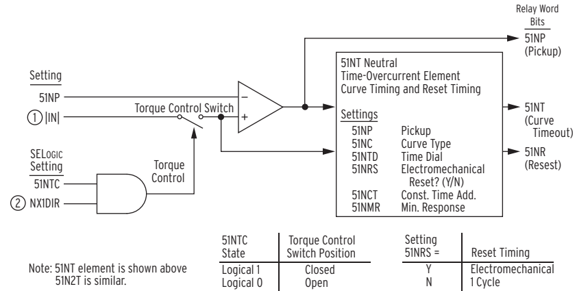
Figure 4.55 Neutral Time-Overcurrent Element 51NT
