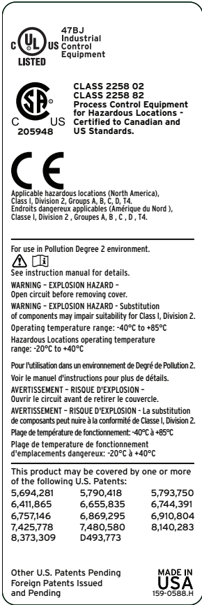
Product Compliance Label for the SEL-700G
