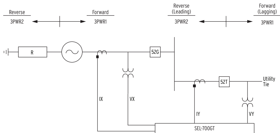
Figure 4.92 Power Elements Operation in the Real/Reactive Power Plane
