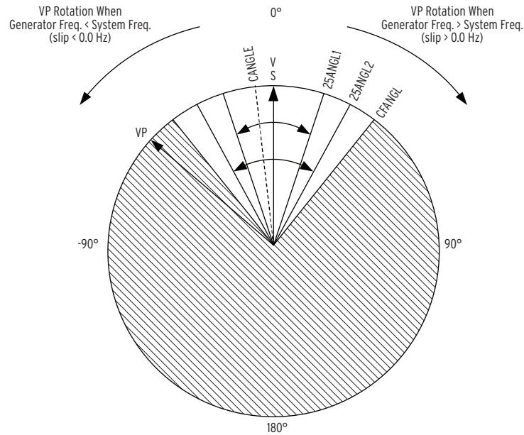
Figure 4.106 Synchronism-Check Function Angle Characteristics
