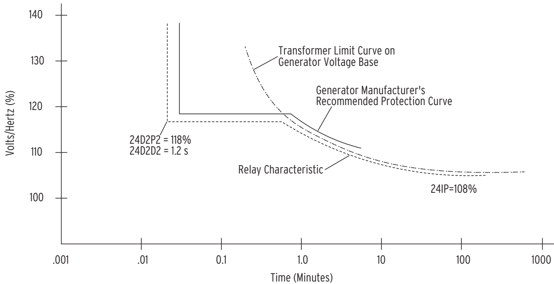
Figure 4.35 Composite Inverse/Definite-Time Overexcitation Characteristic, 24CCS = ID
