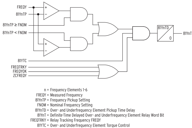
Figure 4.94 Y-Side Over- and Underfrequency Element Logic
