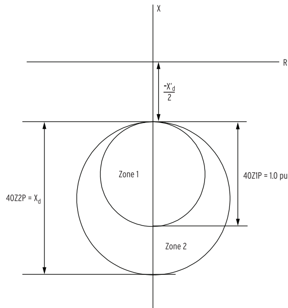
Figure 4.27 Loss-of-Field Element Operating Characteristic, Negative Zone 2 Offset
