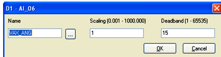
Figure D.7 AI Point Label, Scaling, and Dead Band in acSELEATOR QuickSet
