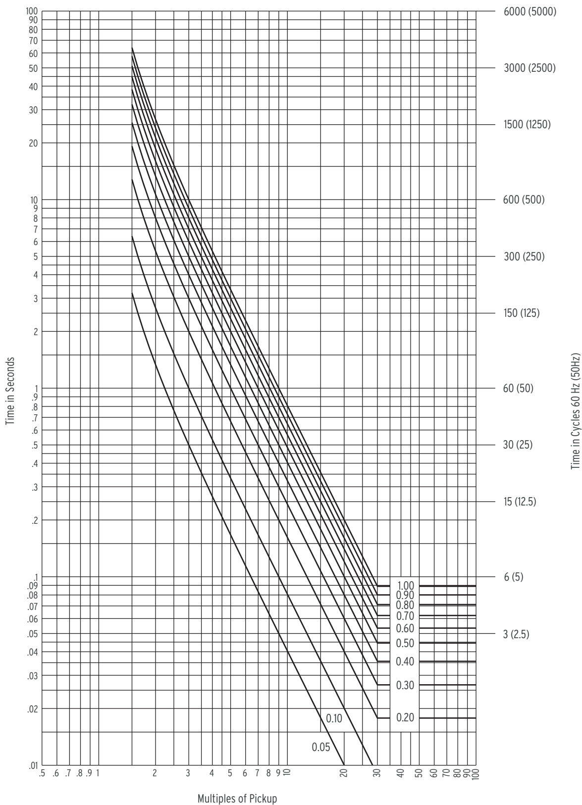
Figure 4.64 IEC Class C Curve (Extremely Inverse): C3
