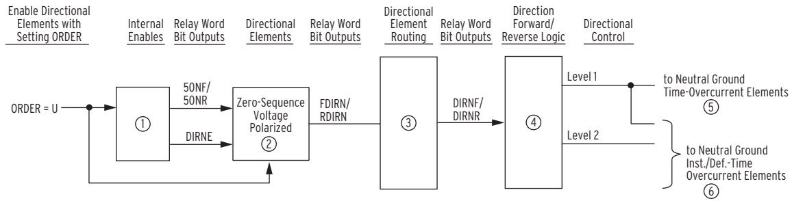
Figure 4.68 General Logic Flow of Directional Control for Neutral-Ground Overcurrent Elements
