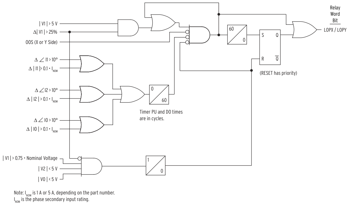
Figure 4.115 Loss-of-Potential Generic Logic (Applies to both X and Y Sides)
