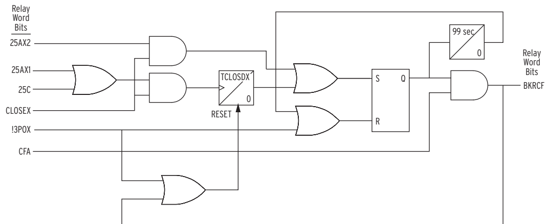
Figure 4.105 Breaker Close Failure Logic Diagram
