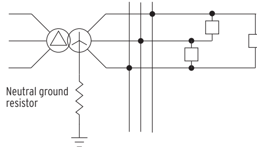
Figure 4.88 Hybrid Power System With Neutral-Ground Resistor
