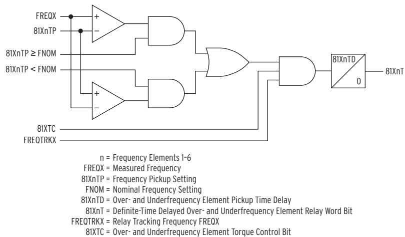
Figure 4.93 X-Side Over- and Underfrequency Element Logic
