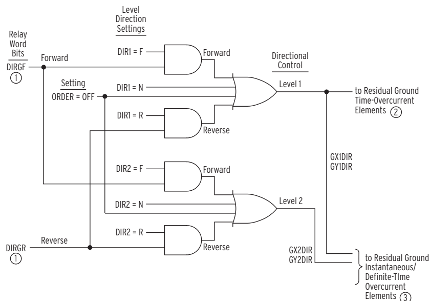
Figure 4.78 Direction Forward/Reverse Logic for Residual-Ground Overcurrent Elements
