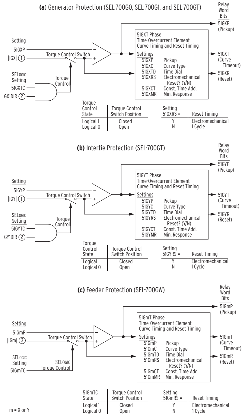
Figure 4.56 Residual Time-Overcurrent Elements
