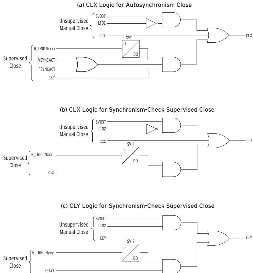
Figure 4.126 Typical Generator or Intertie Close CL Logic (SEL-700G or GT)
