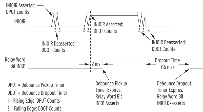
Figure 4.142 Timing Diagram for Debounce Timer Operation When Operating in AC Mode
