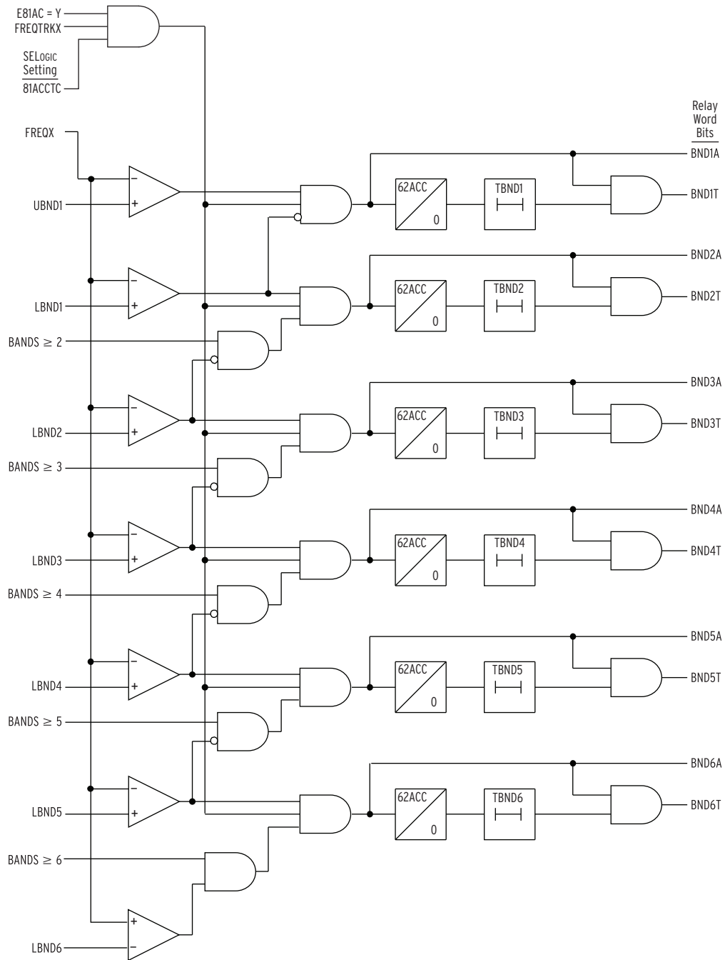
Figure 4.40 Abnormal Frequency Protection Logic Diagram
