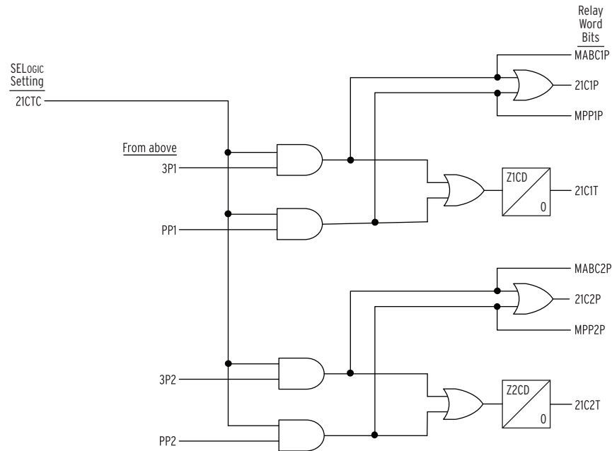
Figure 4.22 Compensator Distance Element Logic
