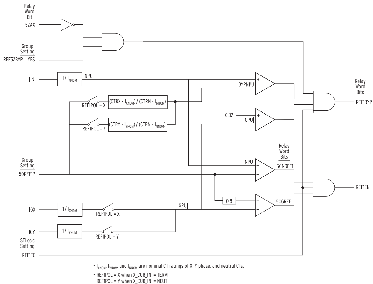
Figure 4.12 REF Enable Logic
