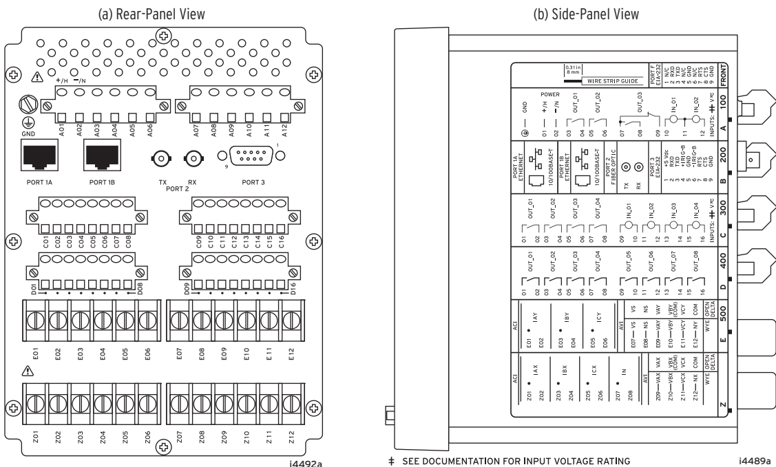
Figure 2.9 SEL-700GT+ With Dual Copper Ethernet, 4 DI/4 DO, 8 DO, 3 ACI/4 AVI, 4 ACI/3 AVI (MOT 0700GT1A2X75850630)
