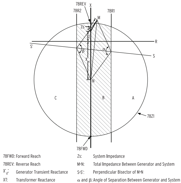
Figure 4.43 Single-Blinder Typical Settings
