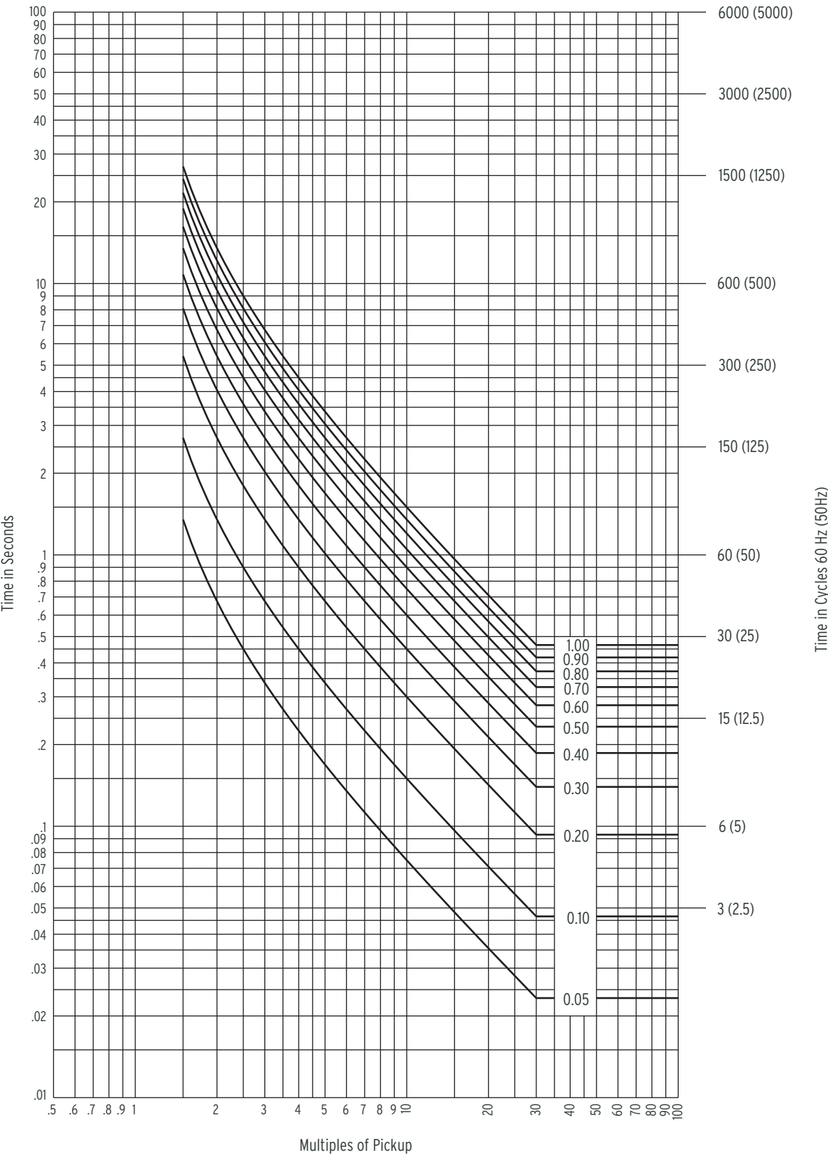
Figure 4.63 IEC Class B Curve (Very Inverse): C2
