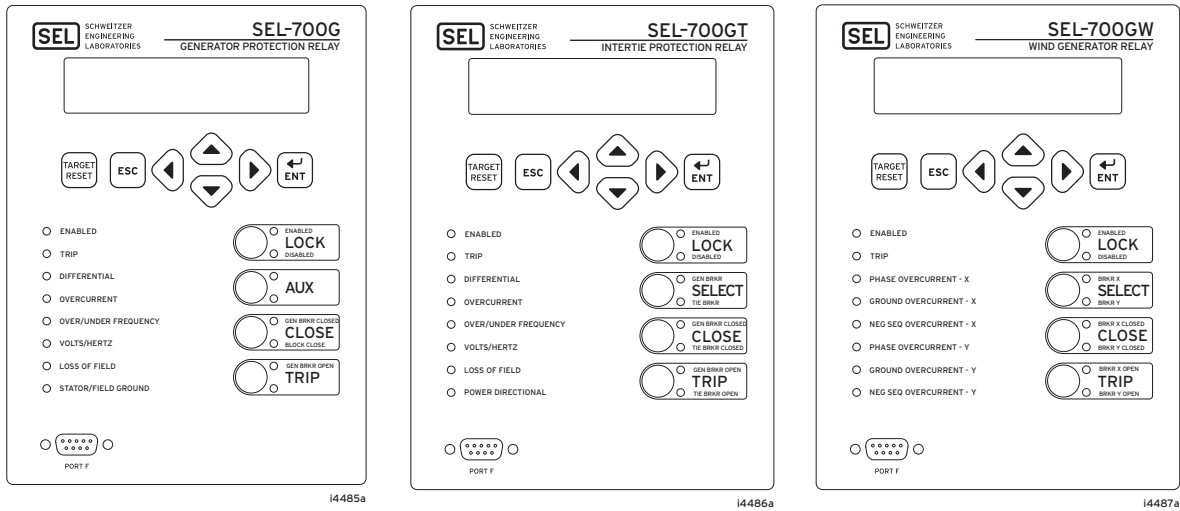
Figure 8.1 Front-Panel Overview
