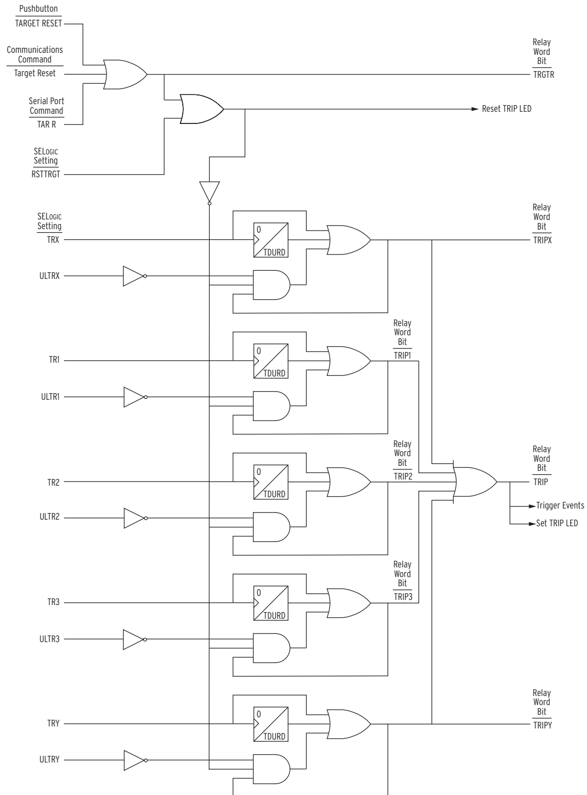
Figure 4.121 Trip Logic
