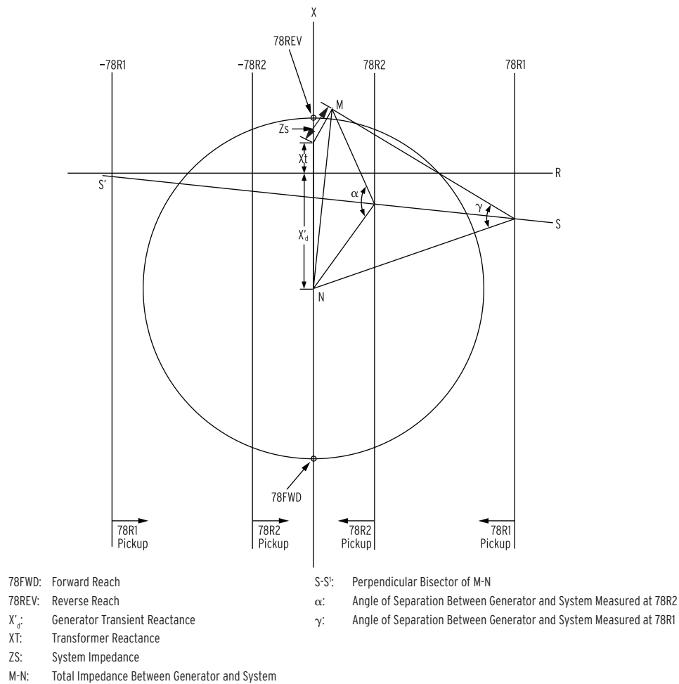
Figure 4.46 Double-Blinder Typical Settings
