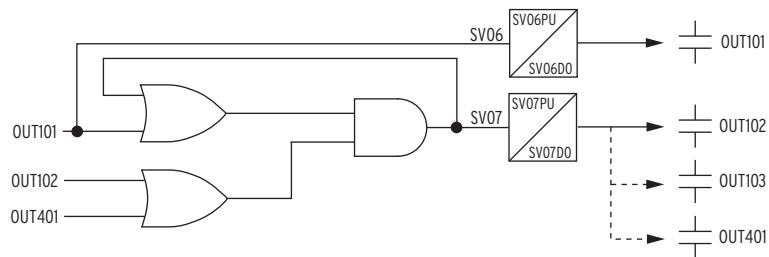
Figure 4.132 Example Use of SELogic Variables/Timers
