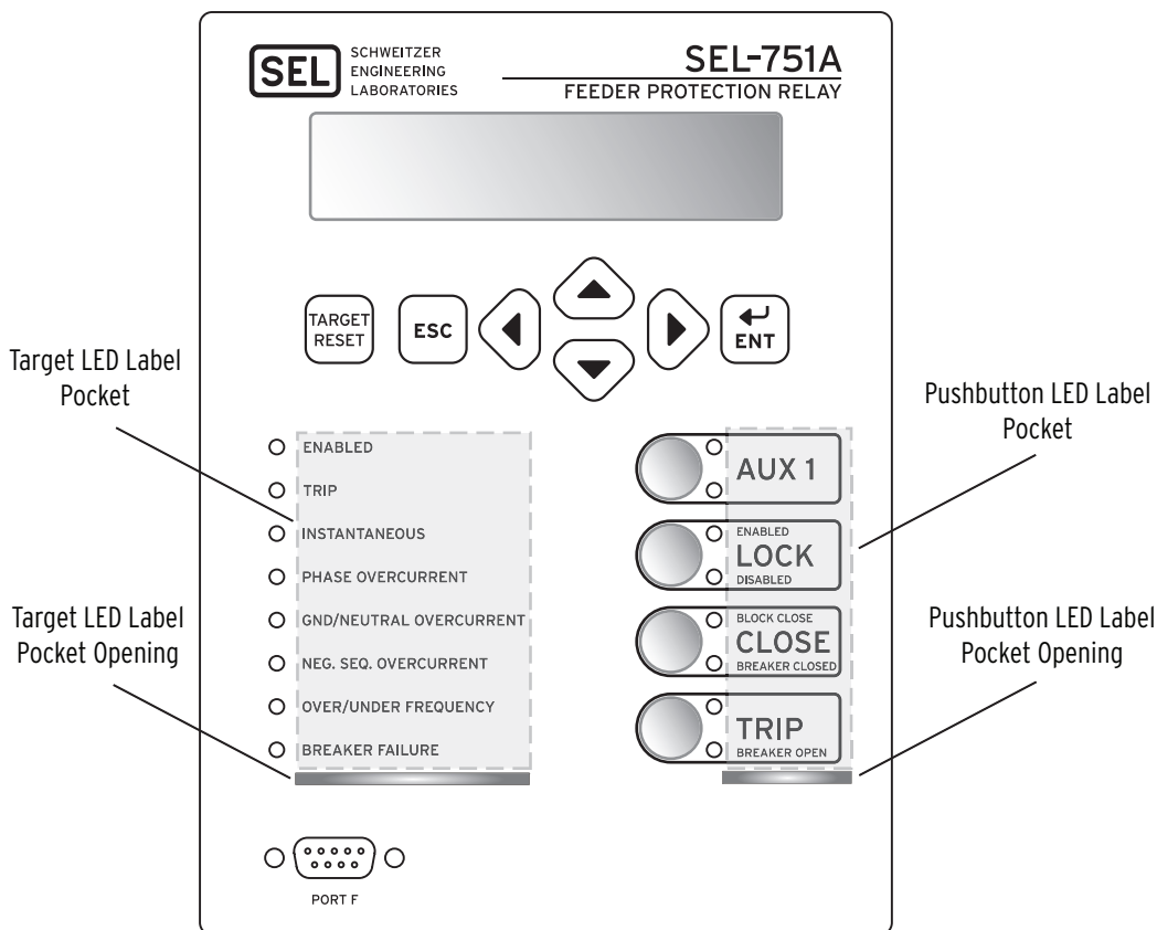
Figure 1 Typical SEL-751A Configurable Label Areas
