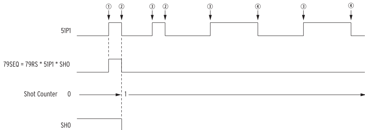
① Fault occurs beyond line recloser; ② fault cleared by line recloser fast curve; ③ line recloser recloses into fault; ④ fault cleared by line recloser slow curve.
