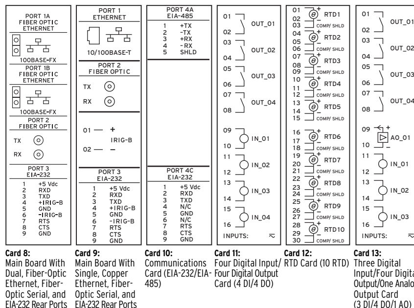
Figure 2.8 Rear-Panel Connections of Selected Cards
