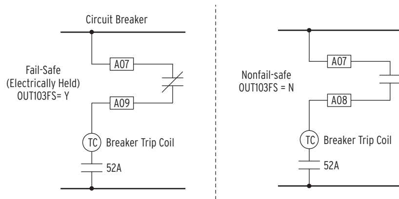
Figure 2.16 OUT103 Contact Fail-Safe and Nonfail-Safe Options
