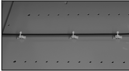
Figure 2.26 Black-Jacketed Fiber Installation Example
