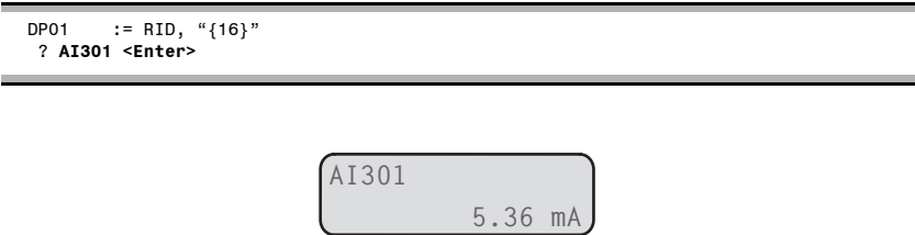
Figure 4.73 Front-Panel Display for an Analog Entry in the Name String Only
