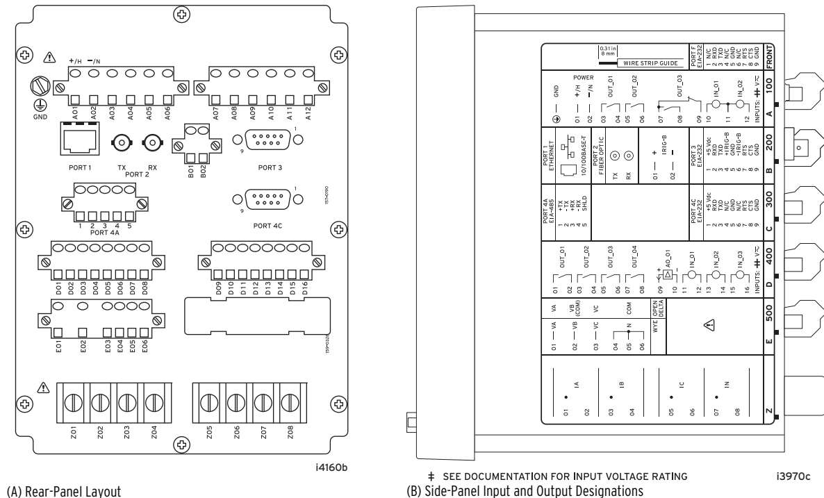
Figure 2.9 Fiber-Optic Serial, Ethernet, EIA-232 Communication, 3 DI/4 DO/1 AO, and 3 AVI Voltage Option
