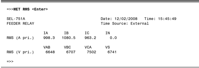
Figure 5.9 Device Response to the METER RMS Command
