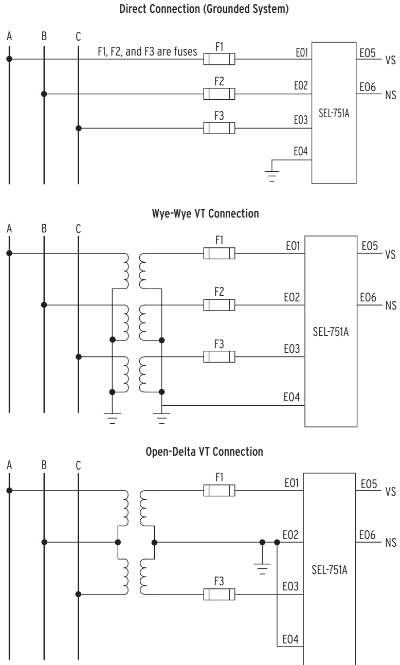
Figure 2.18 Voltage Connections
