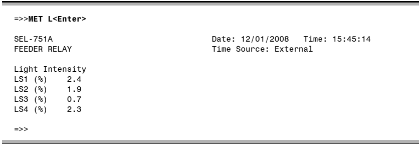
Figure 5.11 Device Response to the METER L (Light) Command
