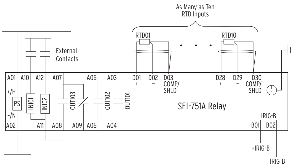
Figure 2.14 Control I/O Connections—Internal RTD Option
