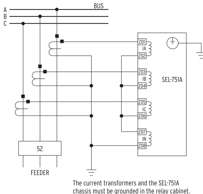
Figure 2.19 Typical Current Connections
