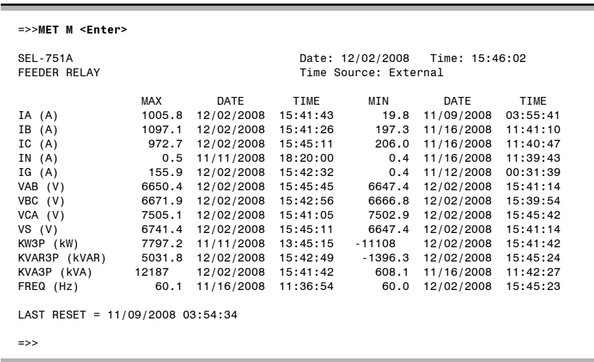
Figure 5.6 Device Response to the METER M Command
