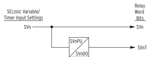
Figure 4.49 SELOGIC Control Equation Variable/Timer SV01/SV01T–SV32T
