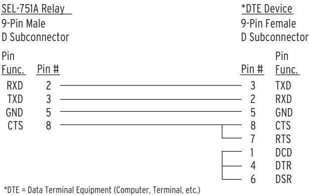
Figure 7.10 SEL Cable C234A–SEL-751A to DTE Device
