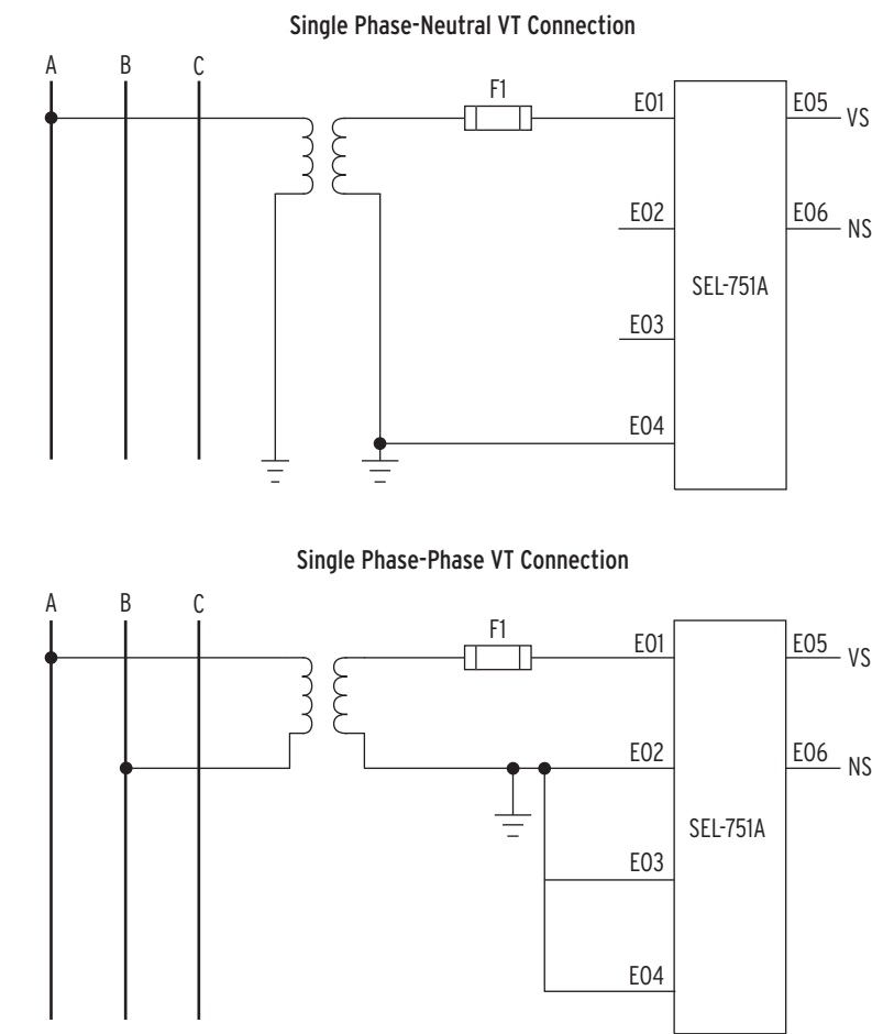
Figure 2.17 Single-Phase Voltage Connections
