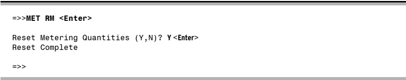
Figure 5.7 Device Response to the METER RM Command
