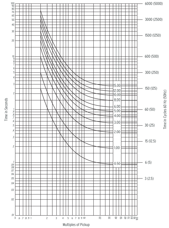
Figure 4.11 U.S. Inverse Curve: U2
