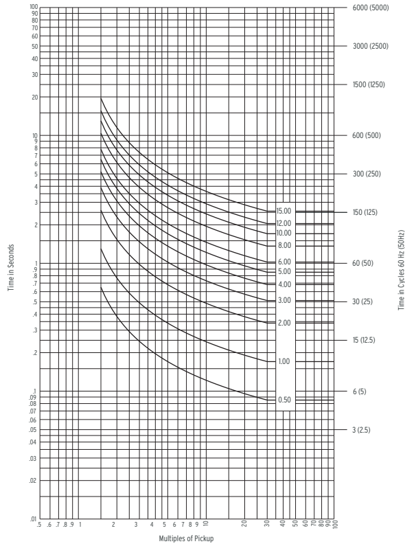
Figure 4.10 U.S. Moderately Inverse Curve: U1
