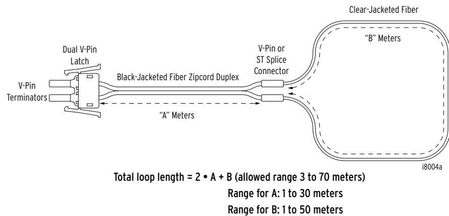
Figure 2.33 Clear-Jacketed Fiber Sensor Assembly
