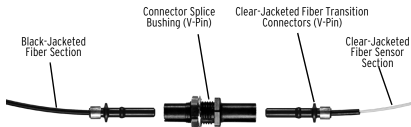
Figure 2.35 Clear-Jacketed Fiber Sensor Components (V-Pin Style)
