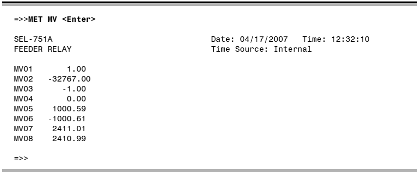
Figure 5.8 Device Response to the METER MV Command
