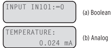
Figure 4.74 Front-Panel Display for an Entry in (a) Boolean Name and Alias Strings and (b) Analog Name and User Text and Formatting Strings
