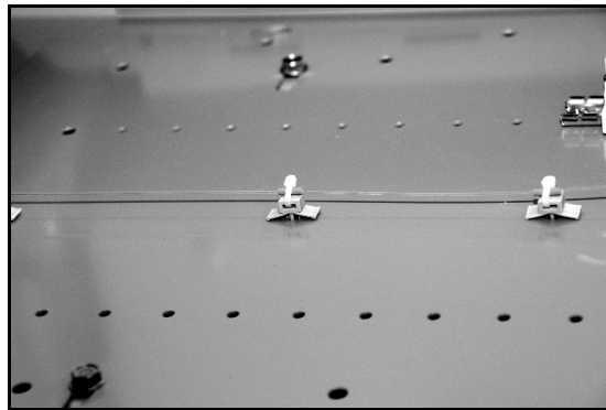
Figure 2.34 Clear-Jacketed Fiber Sensor Mounting Example
