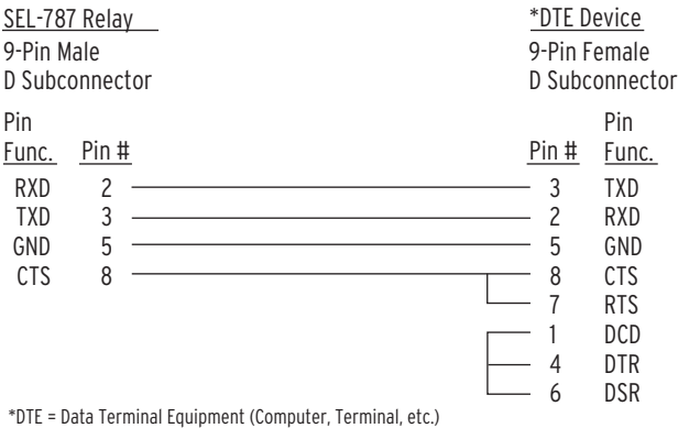
Figure 7.10 SEL Cable C234A–SEL-787 to DTE Device
