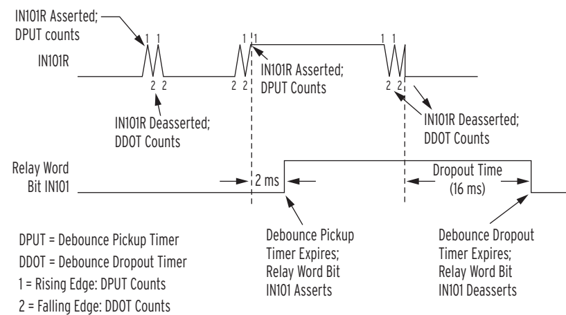
Figure 4.66 Timing Diagram for Debounce Timer Operation When Operating in AC Mode
