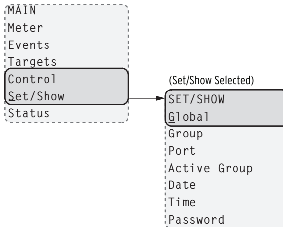
Figure 8.20 MAIN Menu and SET/SHOW Submenu
