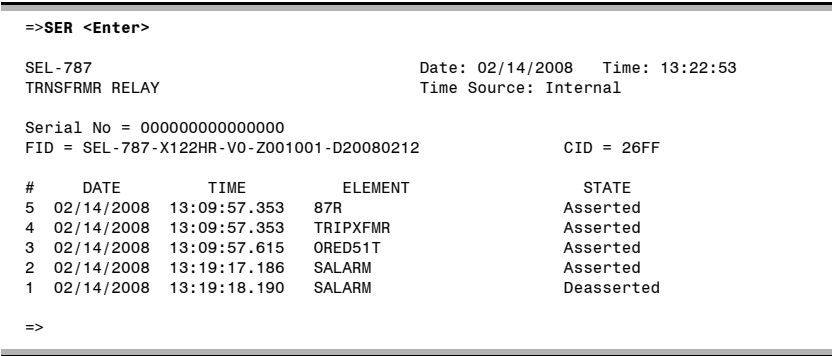
Figure 9.8 Example Sequential Events Recorder (SER) Event Report
