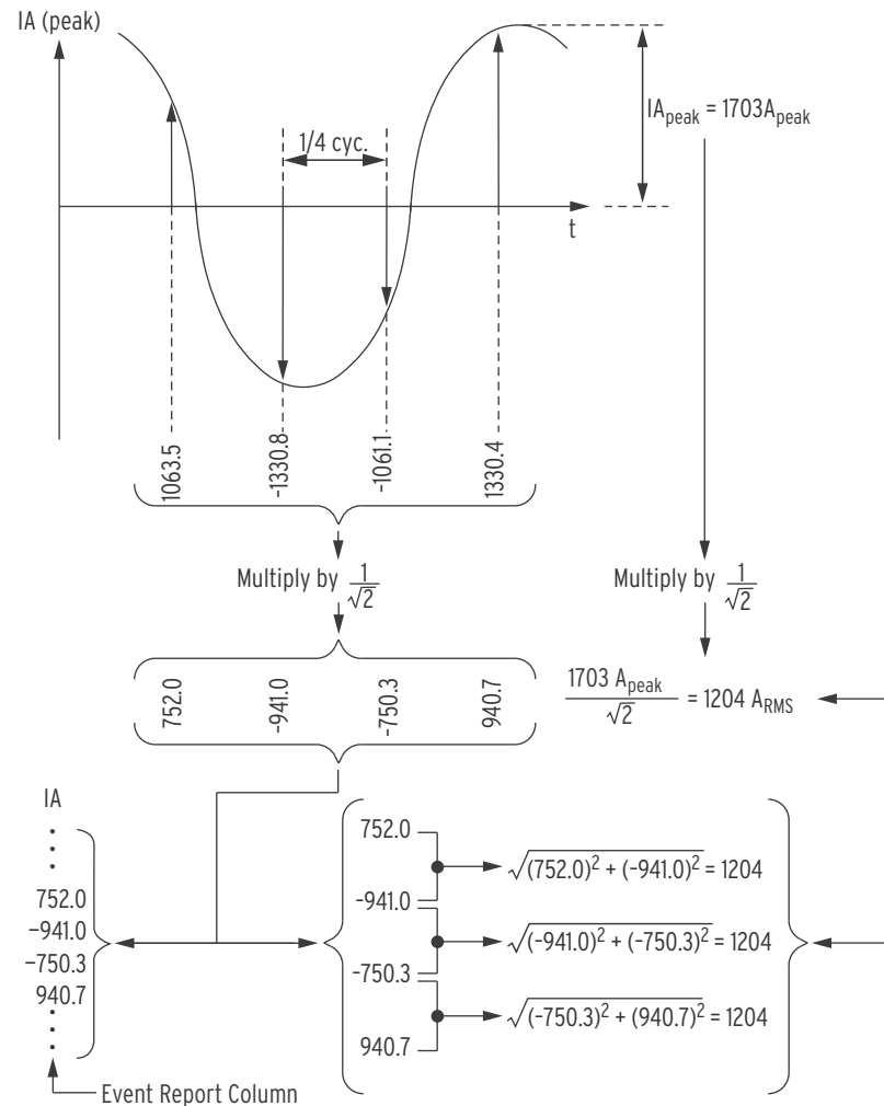
Figure 9.4 Derivation of Analog Event Report Current Values and RMS Current Values From Sampled Current Waveform
