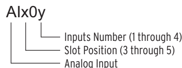
Figure 4.60 Analog Input Card Adaptive Name
