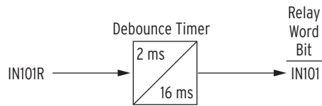
Figure 4.65 AC Mode Processing
