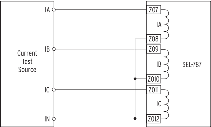
Figure 10.5 CTR2 Current Source Connections
