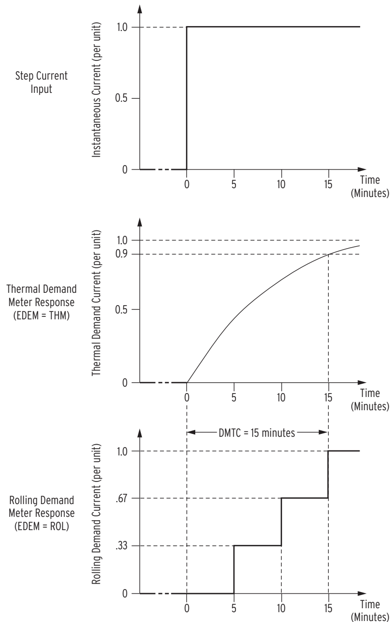
Figure 4.47 Response of Thermal and Rolling Demand Meters to a Step Input (Setting DMTC = 15 minutes)
