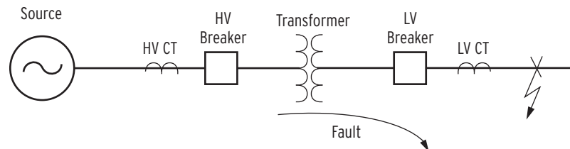
Figure 5.16 Transformer Bank Subjected to Through Fault
