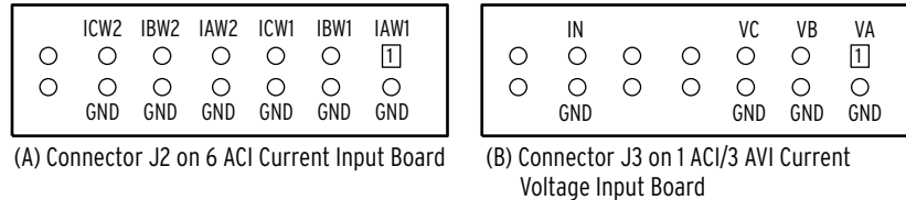
Figure 10.1 Low-Level Test Interface (J2 and J3)
