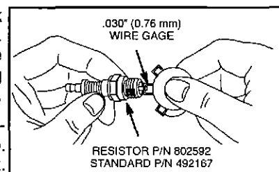
Spark plug
