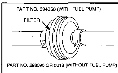
Fuel filter
