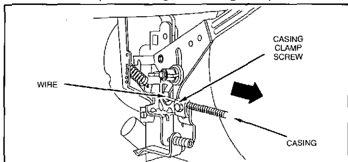
Remote throttle control
