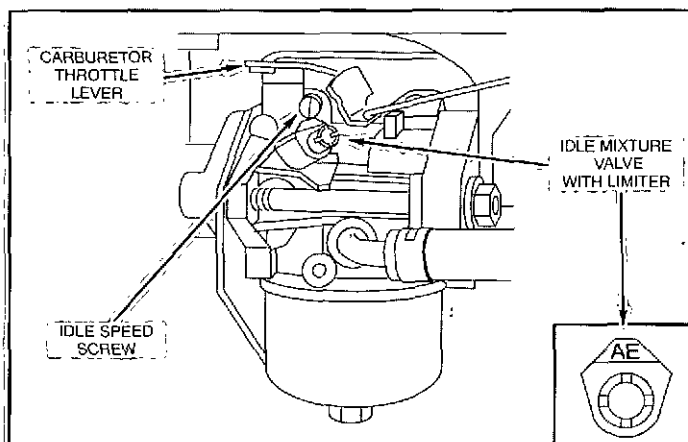
Carburetor adjustments
