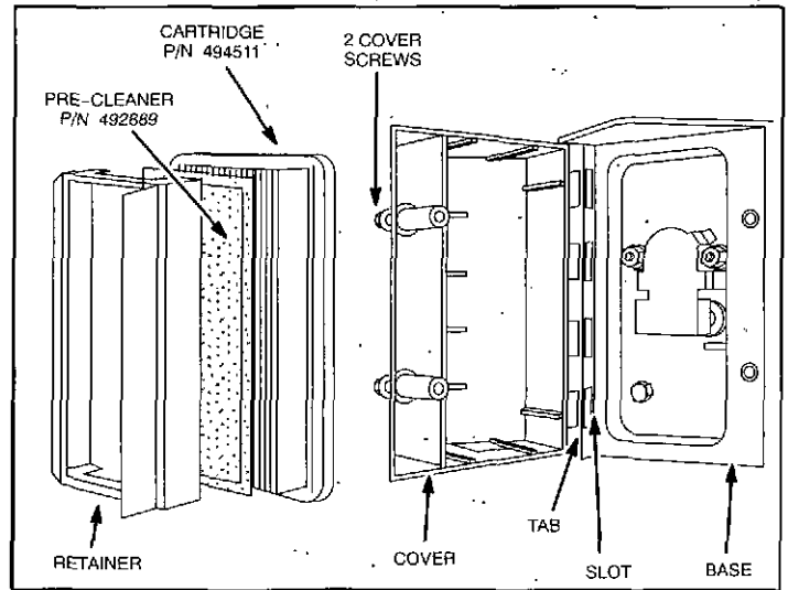
Dual element air cleaner
