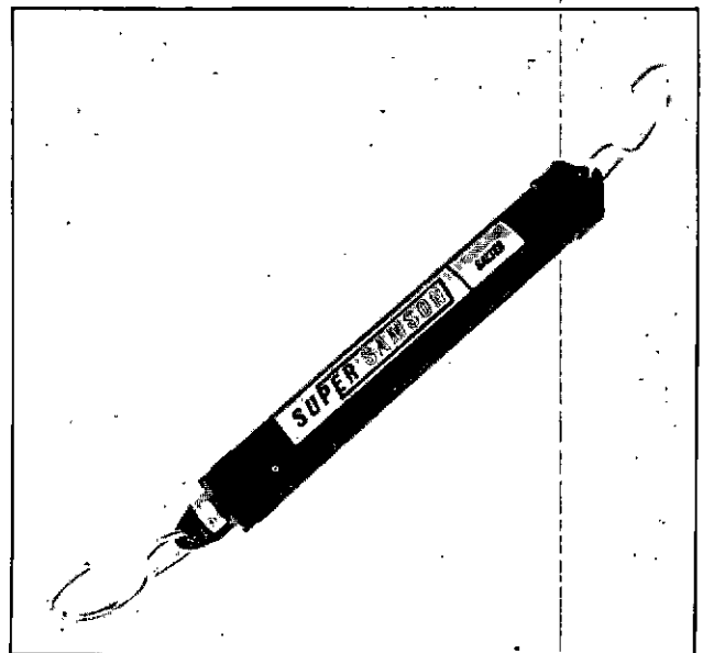
9953840-7 SPRING TENSION GAUGE (For AQ and gear preload)
