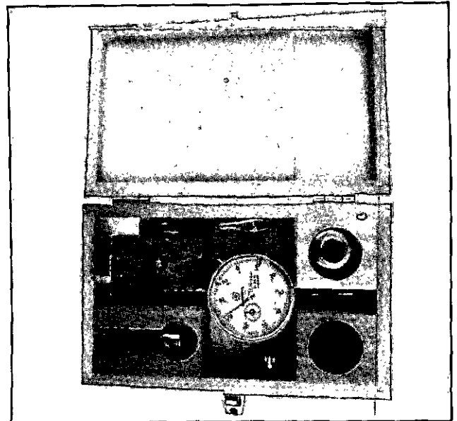
9996770-5 ADAPTORS FOR SETTING INJECTION ANGLE USING LIFT MEASUREMENT 9989876-9 DIAL INDICATOR TO BE USED WITH 9996770-5
