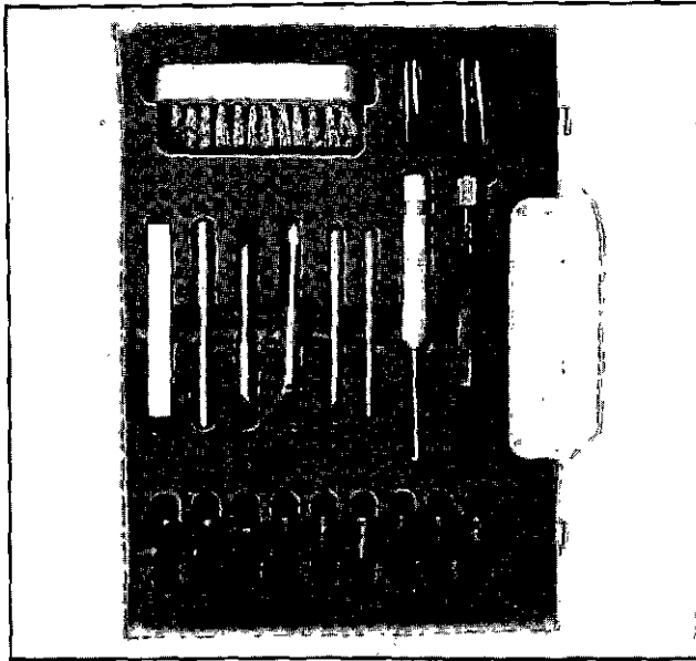
9022900-6 NOZZLE CLEANING KIT For use on all Volvo Penta Injectors
