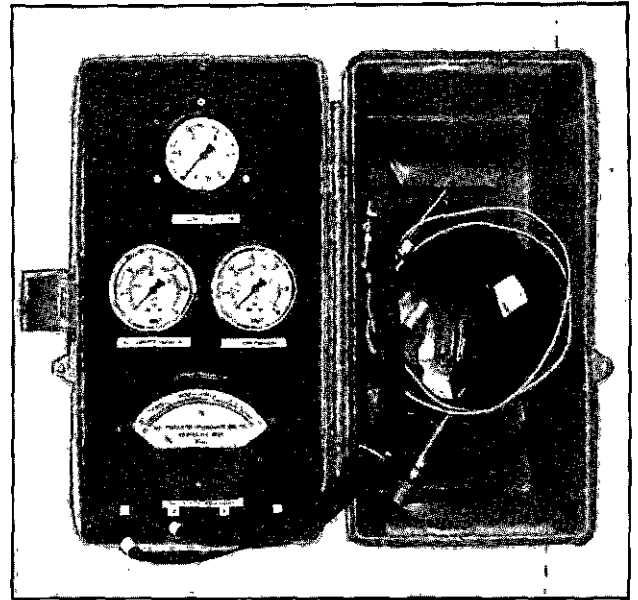
9991023-4 GAUGE BOX For use on all Volvo Penta 4 & 6 Cylinder Diesel Engines (Note: Adaptors for each engine are not included but are listed in the Work Shop Manual)
