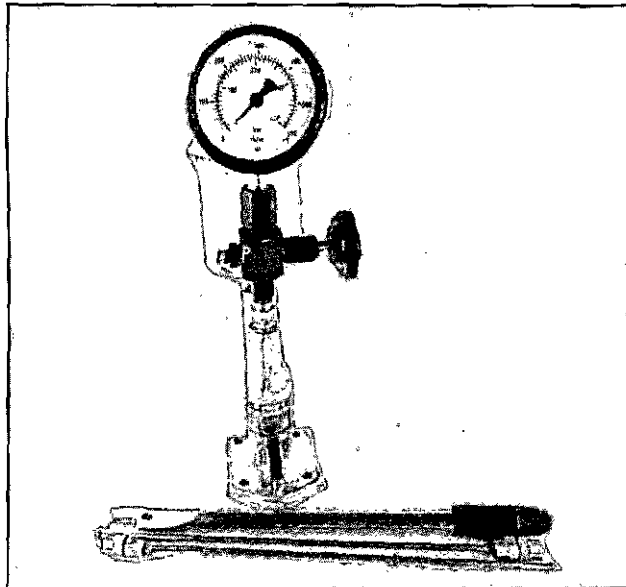
9020060-1 INJECTION (POP) TESTER For testing all Volvo Penta Injectors
