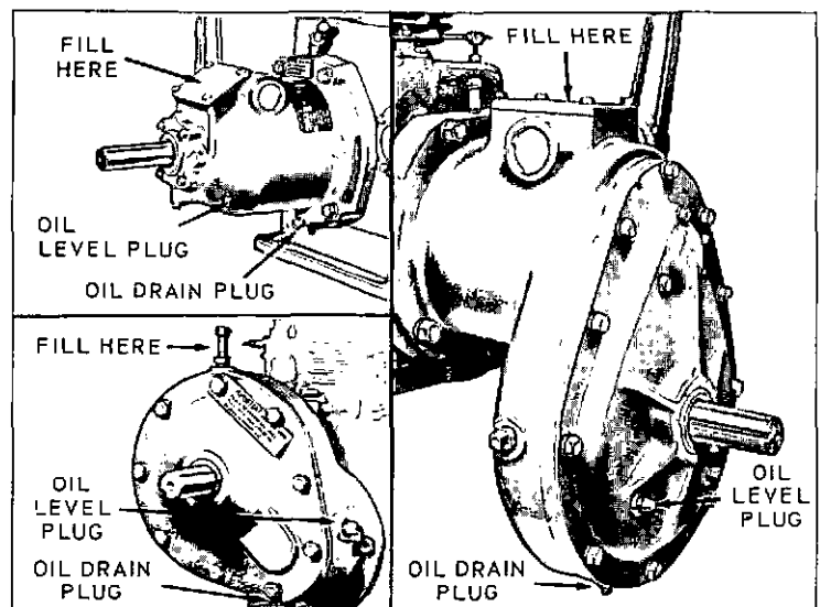
Fig. 2, USE SAME GRADE OIL IN THESE UNITS AS USED IN CRANKCASE - CHANGE EVERY 500 HOURS OF OPERATION
