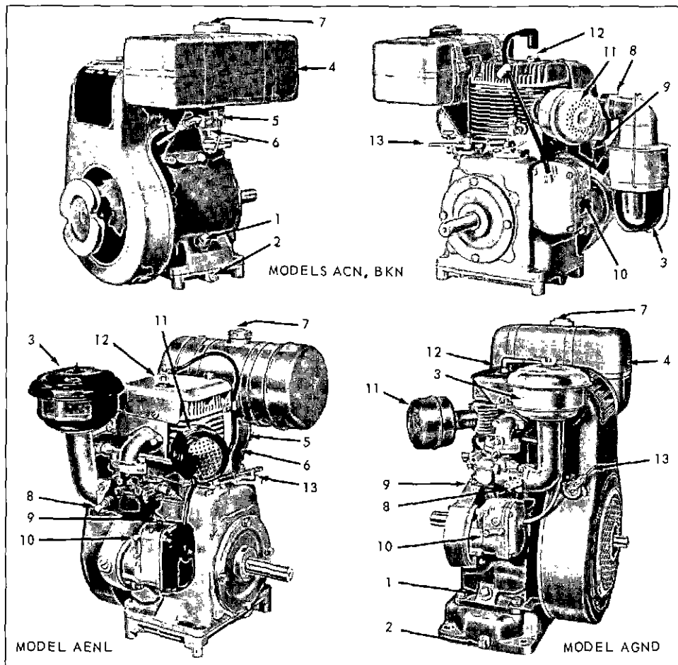
Fig. 3, ENGINE REFERENCE VIEWS
