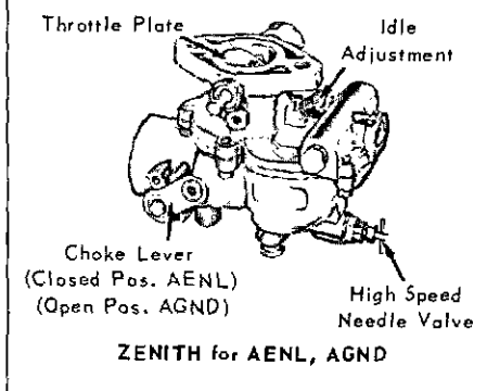
Fig. 5, CARBURETOR ADJUSTMENTS
