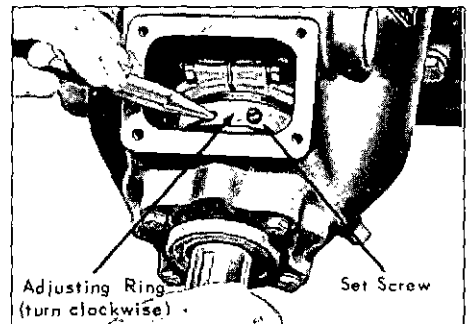
Fig. 15, TWIN DISC CLUTCH
