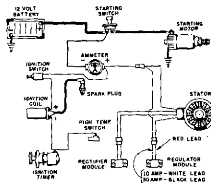
Fig. 14, FLYWHEEL ALTERNATOR
