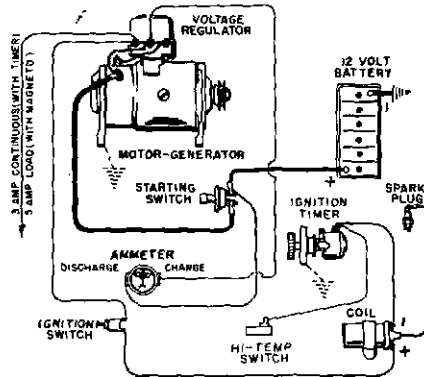
Fig. 13, MOTOR-GENERATOR WIRING
