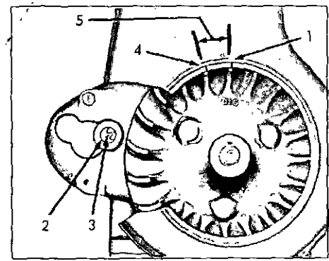
Fig. 9, ACN, BKN TIMING
