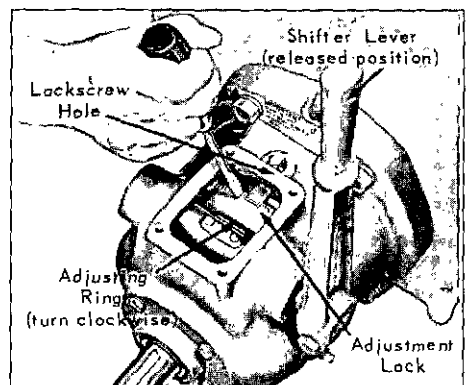
Fig. 16, ROCKFORD CLUTCH
