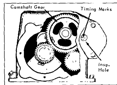
Fig. 11, AGND MAGNETO TIMING
