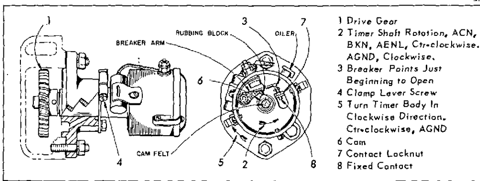
Fig. 12, IGNITION TIMER MOUNTING
