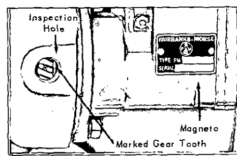
Fig. 10, AENL MAGNETO TIMING
