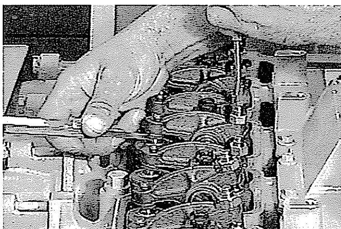
Photo #7-18 - Valve Lash Adjustment
