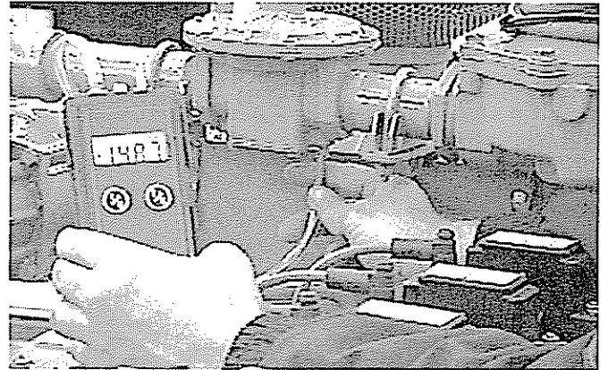
Photo #7-30 - Gas Pressure at Gas Regulator(On Engine) - Checking
