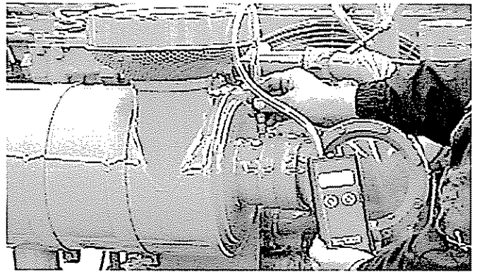
Photo #7-13 - Air Cleaner Restriction - Checking
