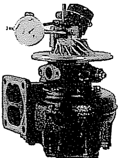
Photo #7-39 - Radial Clearance - Checking
