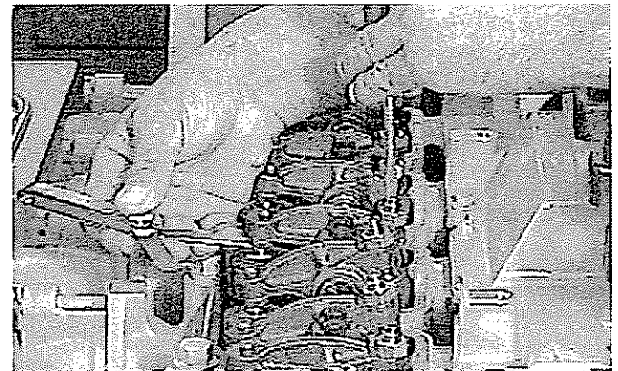
Photo #7-28 - Valve Lash Adjustment
