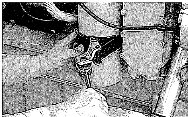
Photo #7-10 - Lube Oil & Lube Oil Filter Changing
