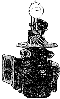
Photo #7-38 - Axial Clearance - Checking
