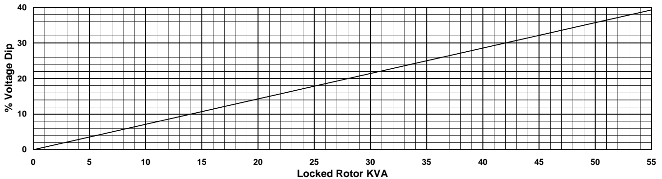
TYPICAL MOTOR STARTING CHARACTERISTICS
