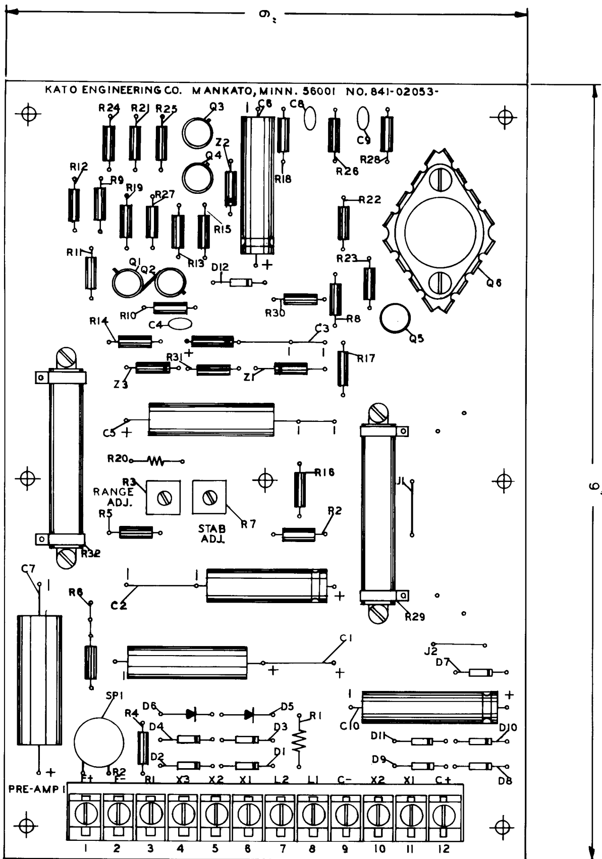
Fig. 5-4 Circuit Board Outline Drawing
