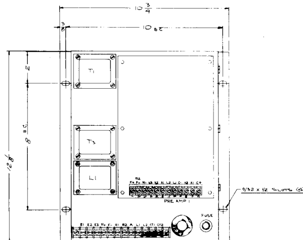
Fig. 5-1 Regulator Outline Drawing
