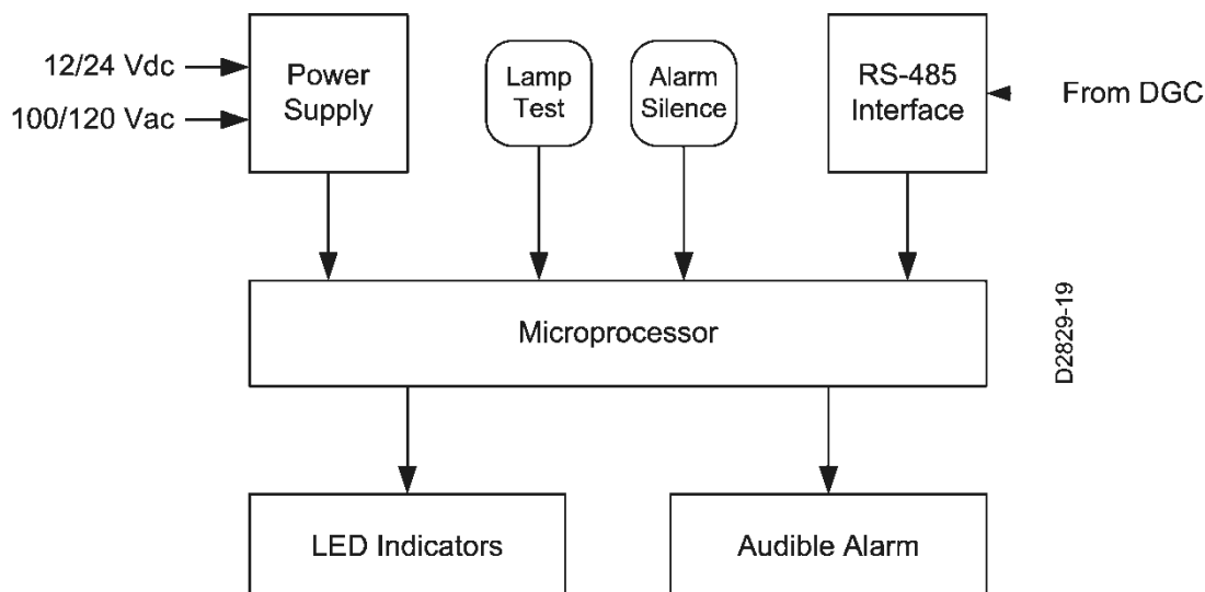
Figure 4. RDP-110 Function Blocks
