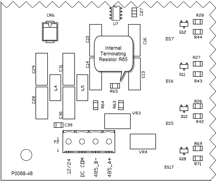
Figure 7. RS-485 Terminating Resistor Location
