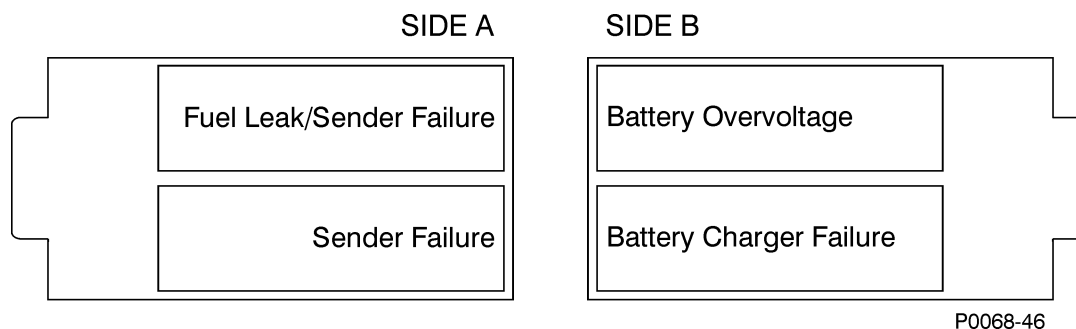
Figure 3. Programmable Alarm and Pre-Alarm Label Cards
