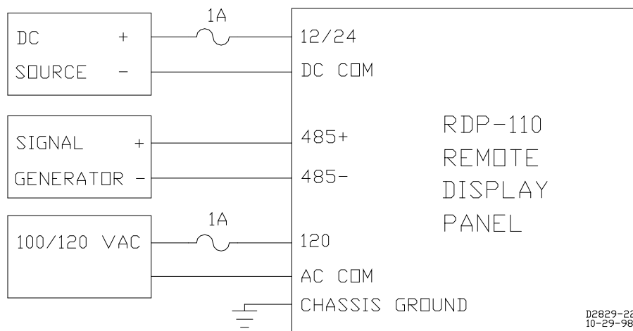
Figure 9. RDP-110 Test Setup
