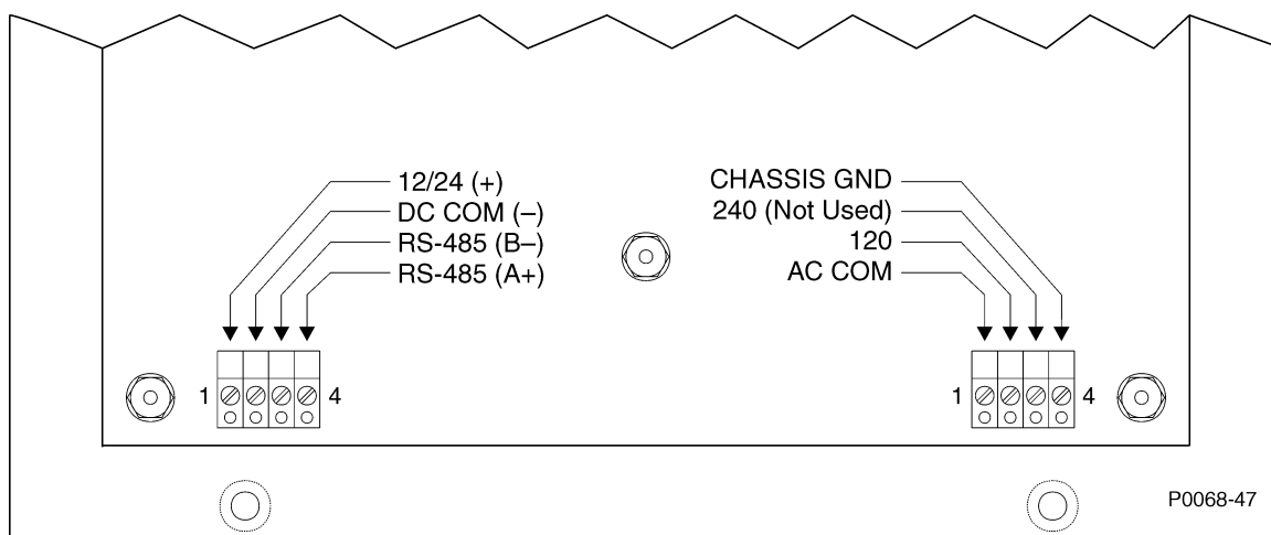
Figure 6. RDP-110 Circuit Board Connections
