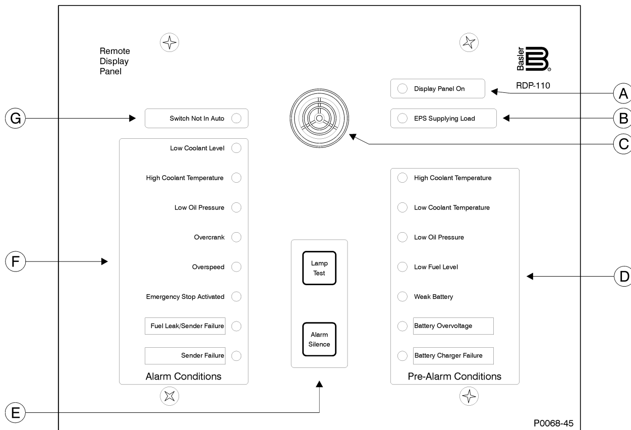
Figure 2. Controls and Indicators
