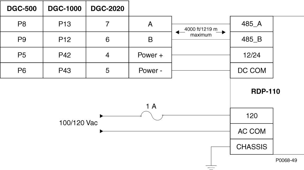
Figure 8. Typical RDP-110 Connections
