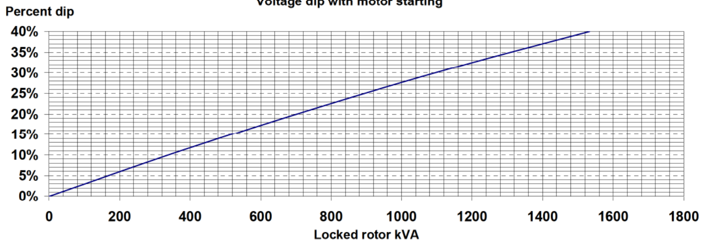
Voltage dip with motor starting
