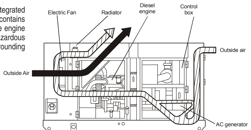
Flow of Cooling Air
