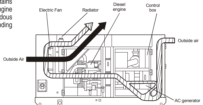
Flow of Cooling Air
