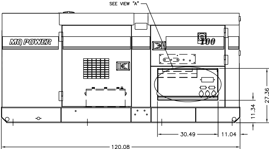
LEFTSIDE VIEW
