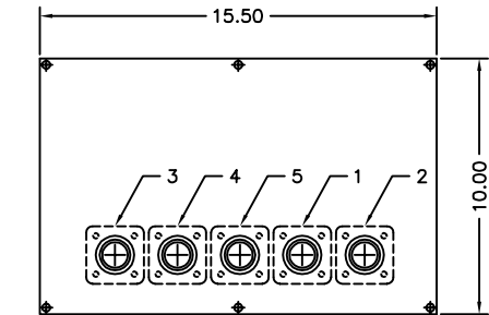
SINGLE CONDUCTOR CAMLOK PANEL (SCALE: 3=1)
