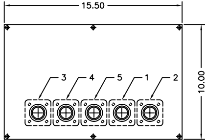
SINGLE CONDUCTOR CAMLOK PANEL (SCALE: 3=1)
