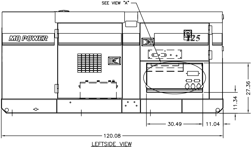
LEFTSIDE VIEW
