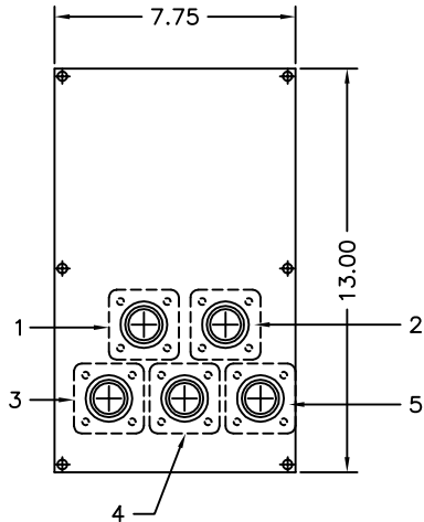
SINGLE CONDUCTOR CAMLOK PANEL (SCALE: 3=1)
