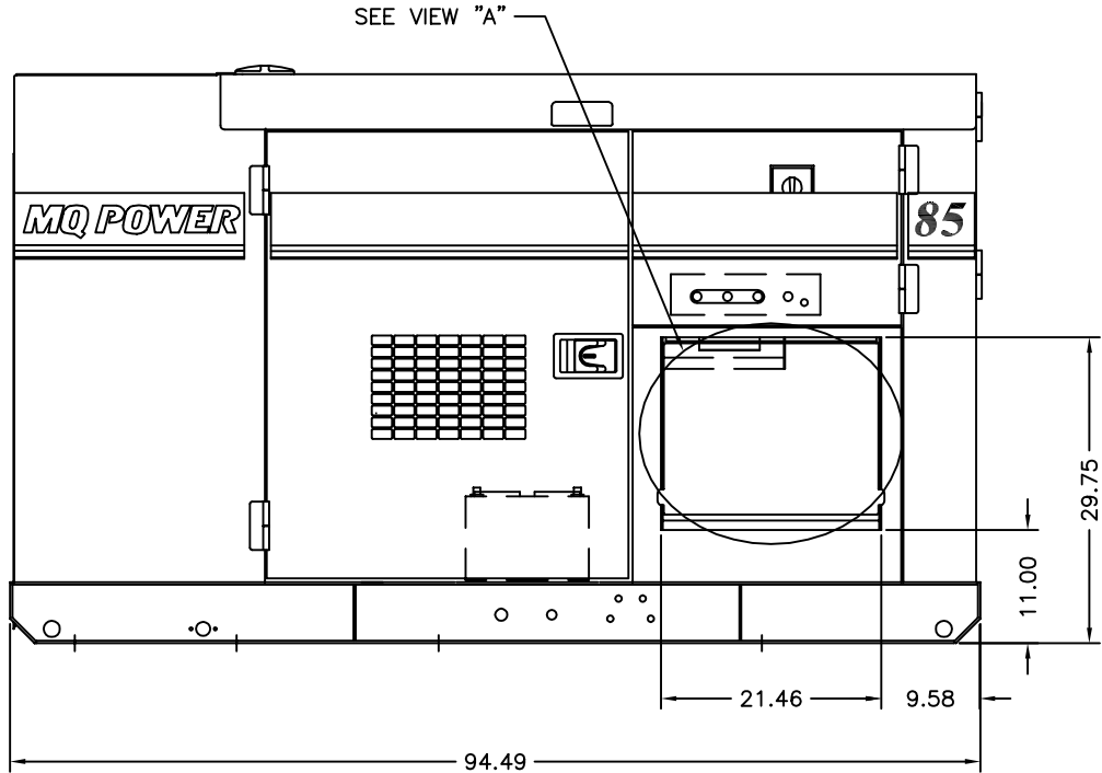
LEFTSIDE VIEW
