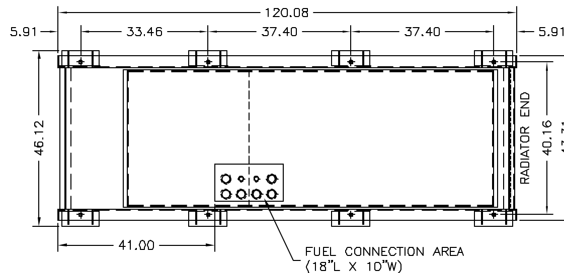
TOP VIEW OF 90GAL. SUBBASE TANK WITH RUPTURE BASIN & STUB-UP
