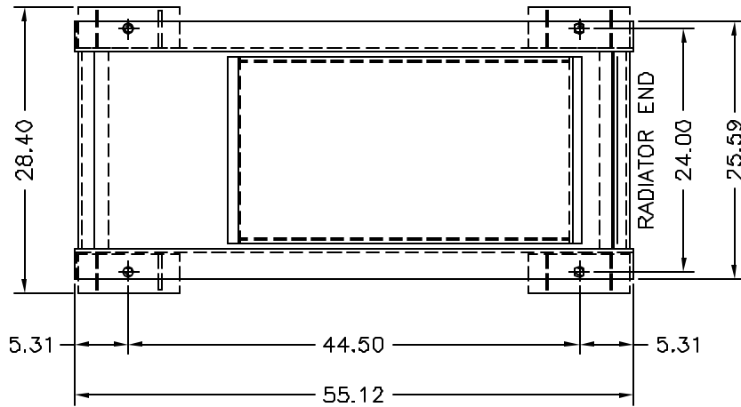
TOP VIEW OF 15GAL. SUBBASE TANK WITH RUPTURE BASIN & STUB-UP
