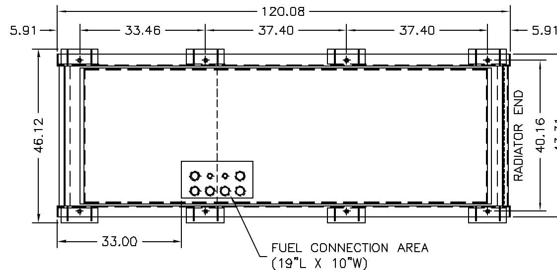
TOP VIEW OF 100GAL. SUBBASE TANK WITH RUPTURE BASIN & STUB-UP
