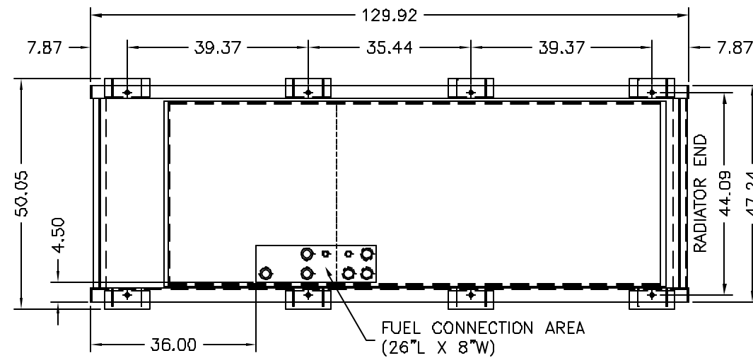
TOP VIEW OF 130GAL. SUBBASE TANK WITH RUPTURE BASIN & STUB-UP
