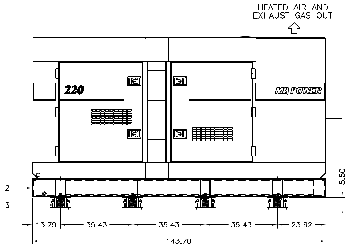
SIDE VIEW
