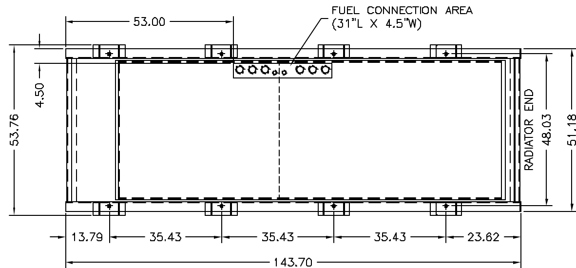
TOP VIEW OF 165GAL. SUBBASE TANK WITH RUPTURE BASIN & STUB-UP
