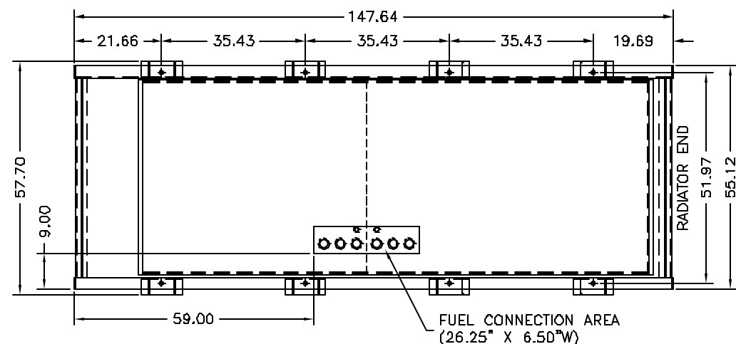
TOP VIEW OF 235GAL. SUBBASE TANK WITH RUPTURE BASIN & STUB-UP
