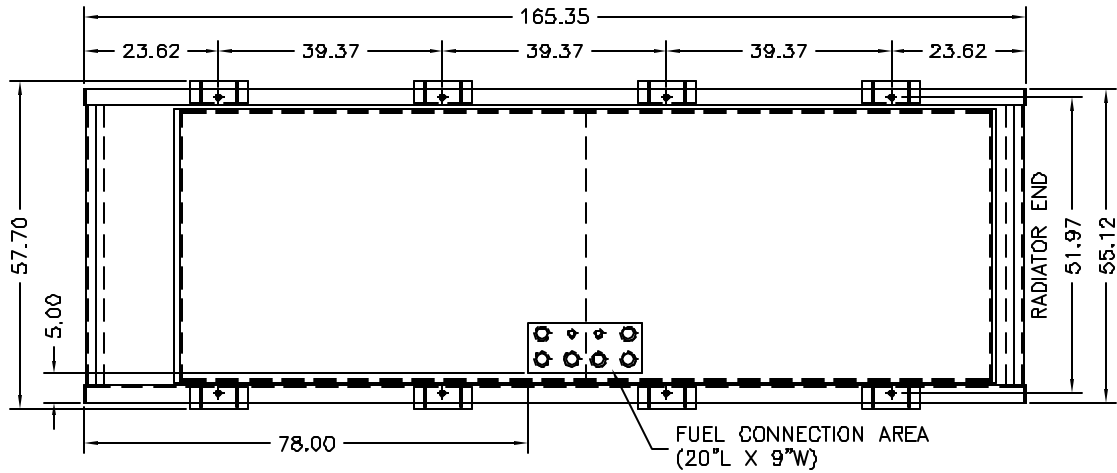
TOP VIEW OF 270GAL. SUBBASE TANK WITH RUPTURE BASIN & STUB-UP
