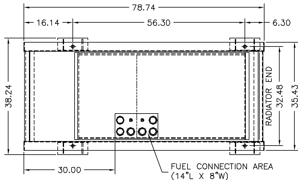
TOP VIEW OF 40GAL. SUBBASE TANK WITH RUPTURE BASIN & STUB-UP
