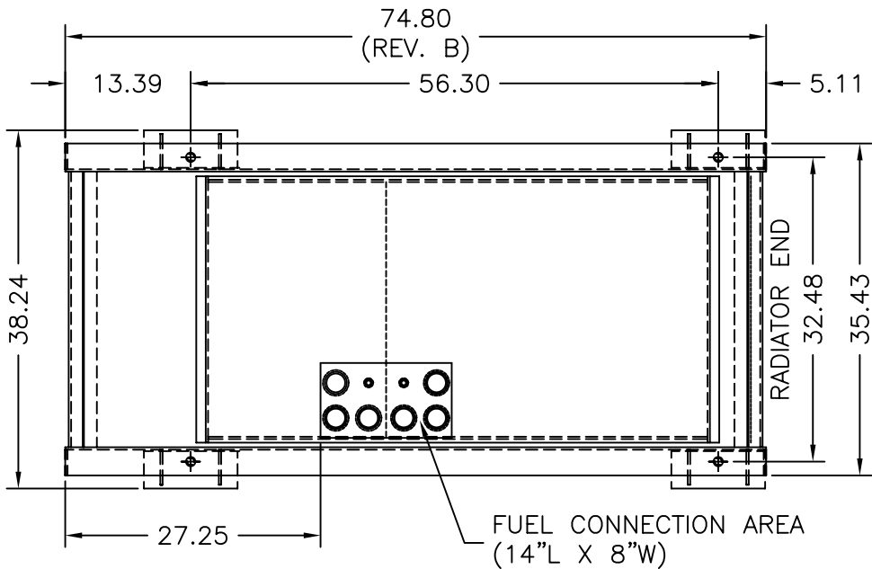
TOP VIEW OF 40GAL. SUBBASE TANK WITH RUPTURE BASIN & STUB-UP
