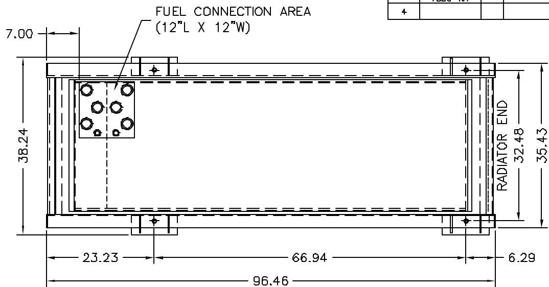
TOP VIEW OF 55GAL. SUBBASE TANK WITH RUPTURE BASIN & STUB-UP
