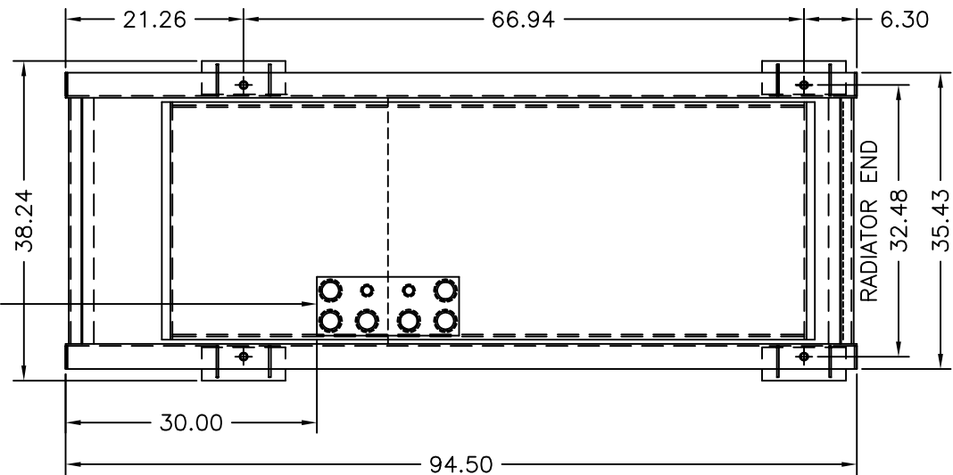
TOP VIEW OF 55GAL. SUBBASE TANK WITH RUPTURE BASIN & STUB-UP
