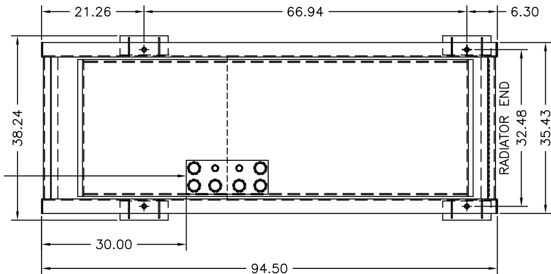
TOP VIEW OF 60GAL. SUBBASE TANK WITH RUPTURE BASIN & STUB-UP
