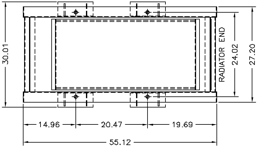
TOP VIEW OF 20GAL. SUBBASE TANK WITH RUPTURE BASIN & STUB-UP
