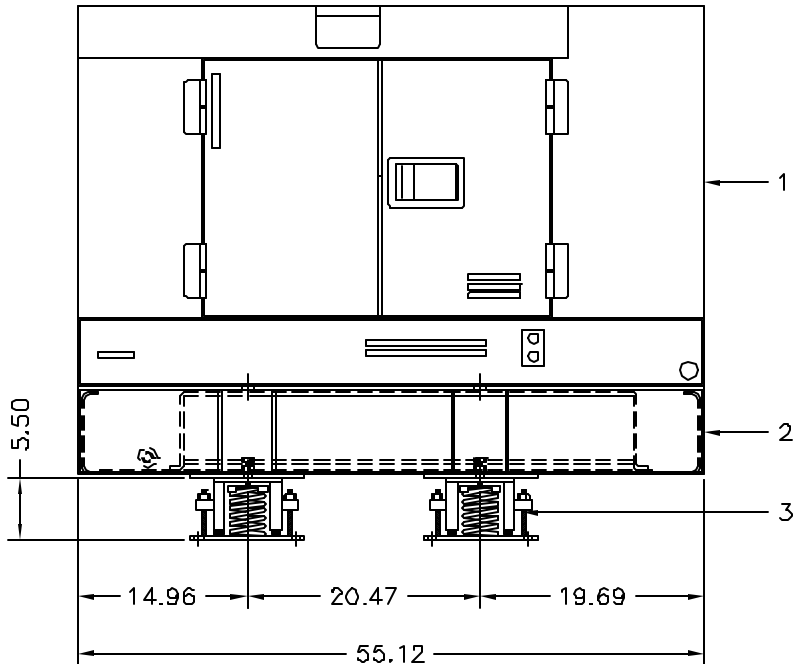
SIDE VIEW
