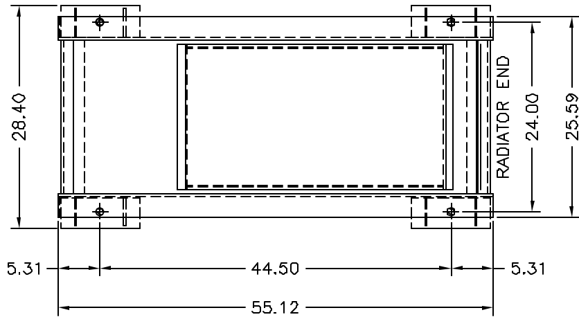
TOP VIEW OF 30GAL. SUBBASE TANK WITH RUPTURE BASIN & STUB-UP
