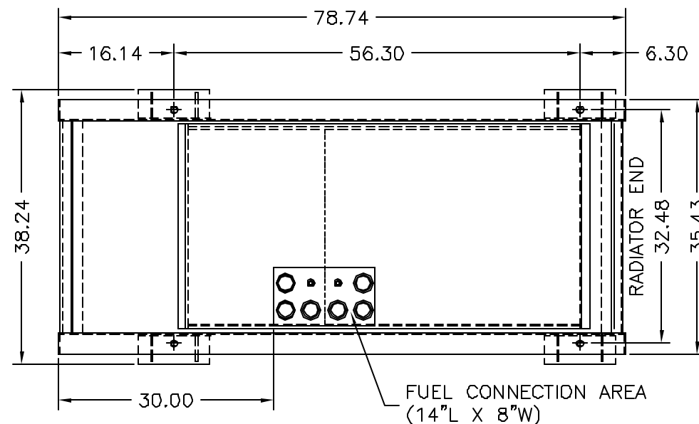
TOP VIEW OF 80GAL. SUBBASE TANK WITH RUPTURE BASIN & STUB-UP
