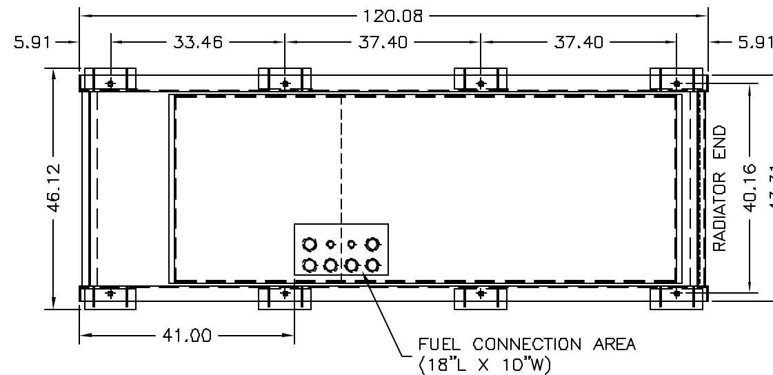
TOP VIEW OF 180GAL. SUBBASE TANK WITH RUPTURE BASIN & STUB-UP
