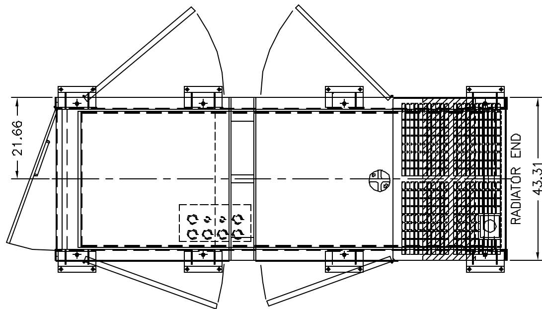
TOP VIEW
