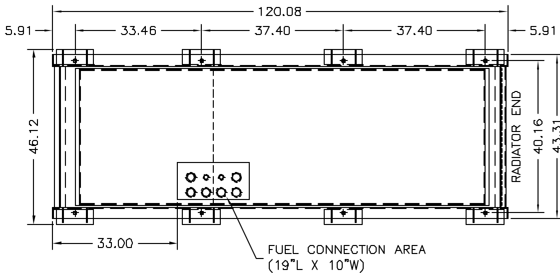
TOP VIEW OF 200GAL. SUBBASE TANK WITH RUPTURE BASIN & STUB-UP
