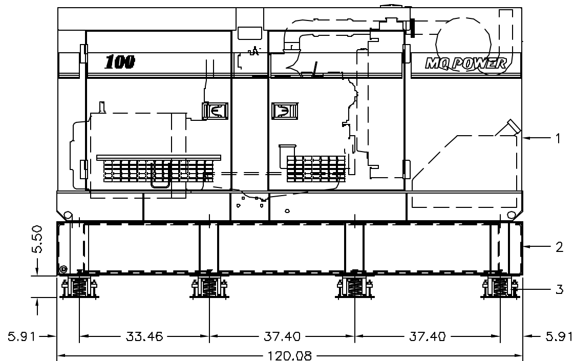
SIDE VIEW
