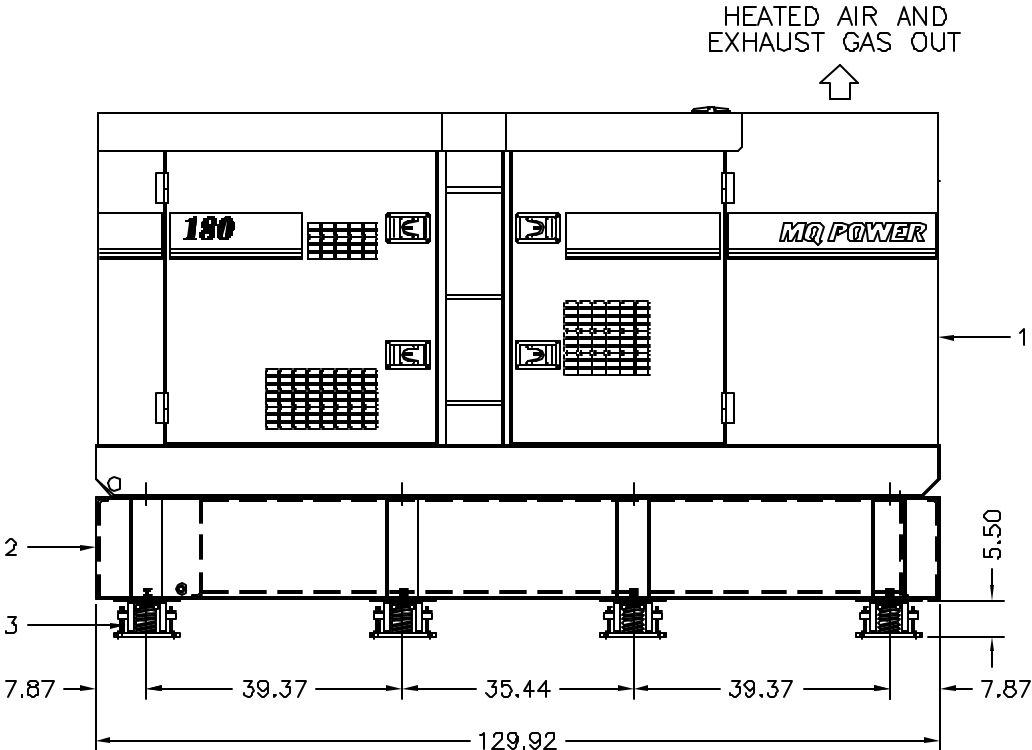
SIDE VIEW
