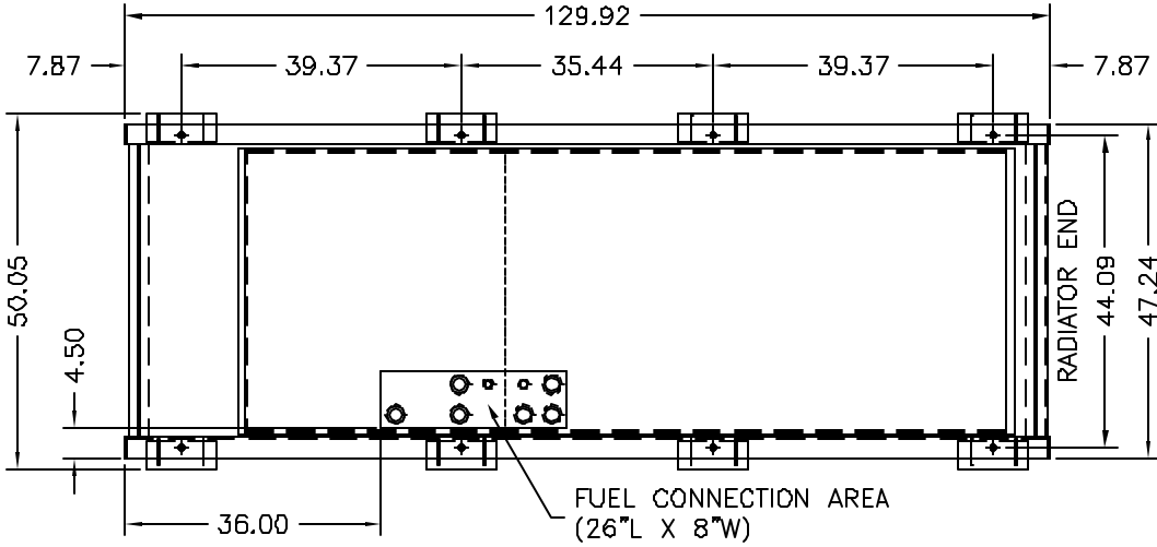
TOP VIEW OF 260GAL. SUBBASE TANK WITH RUPTURE BASIN & STUB-UP
