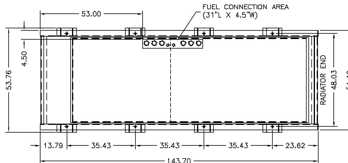
TOP VIEW OF 330GAL. SUBBASE TANK WITH RUPTURE BASIN & STUB-UP
