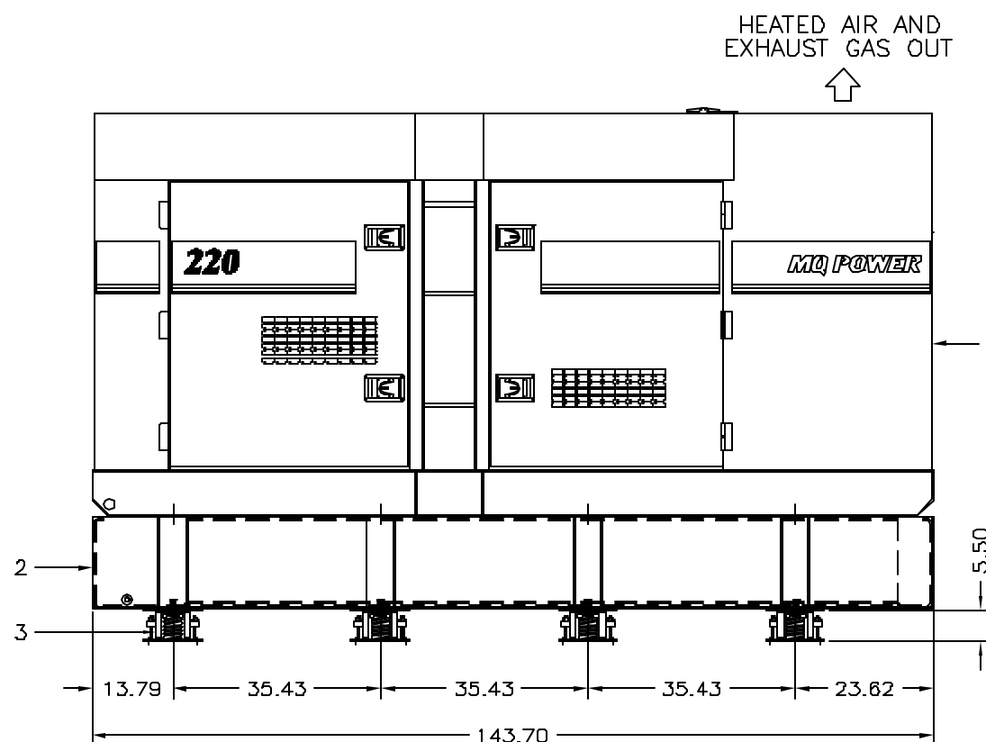
SIDE VIEW
