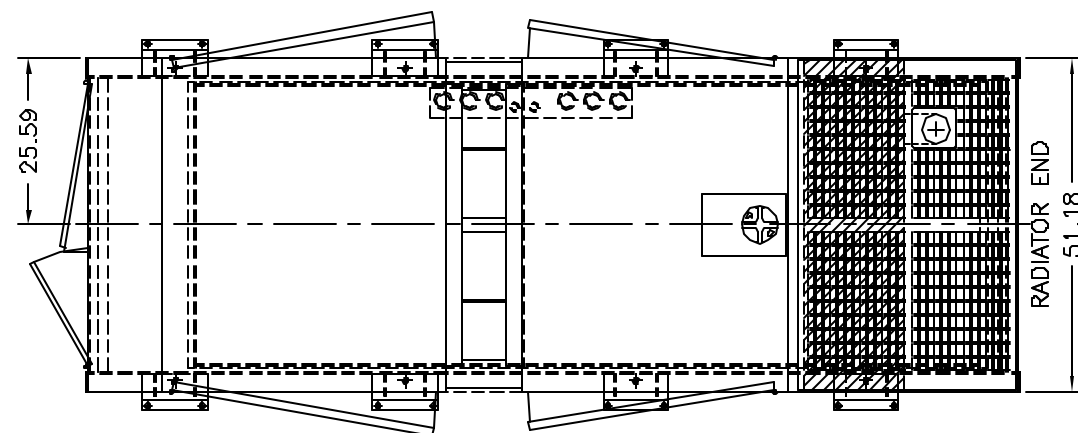
TOP VIEW
